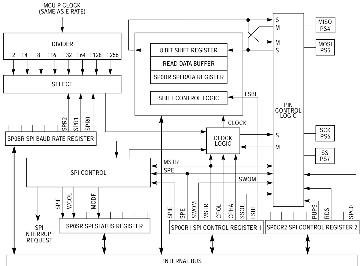
Figure 21 Serial Peripheral Interface Block Diagram
