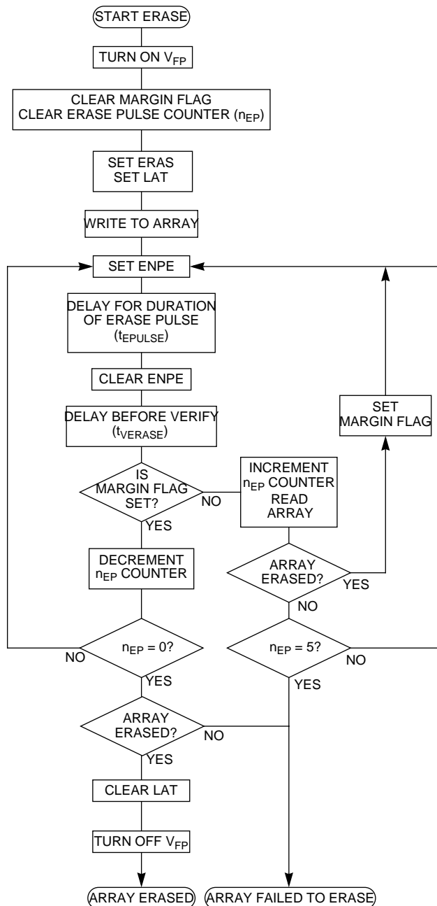
Figure 8 Erase Sequence Flow
