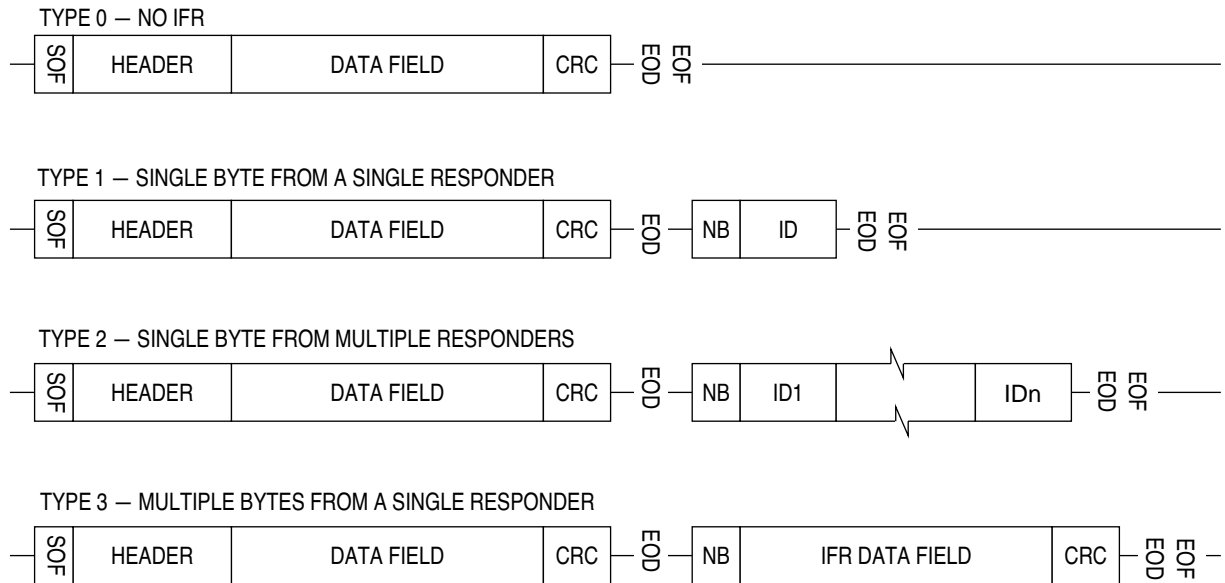
Figure 25 Types of In-Frame Response
