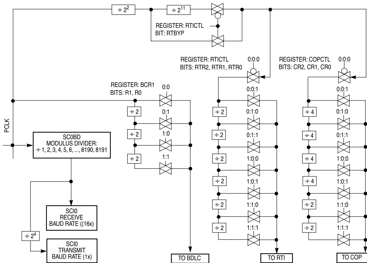
Figure 12 Clock Chain for SCI, BDLCL, RTI, COP
