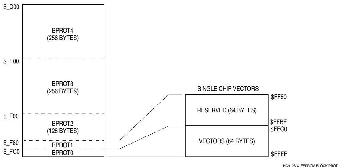
Figure 9 EEPROM Block Protect Mapping
