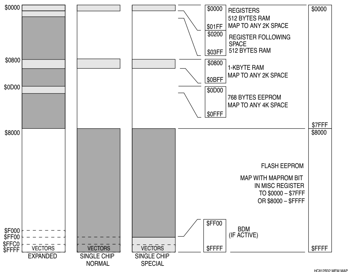
Figure 6 MC68HC912B32 Memory Map
