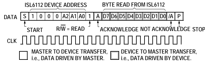
FIGURE 19. RECEIVE_BYTE PROTOCOL
