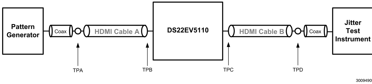
FIGURE 13. Simplified Test Setup as a Single Repeater
