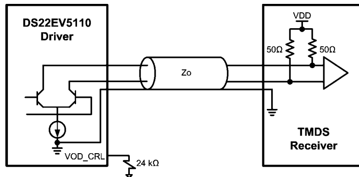
FIGURE 9. DC Coupled Application
