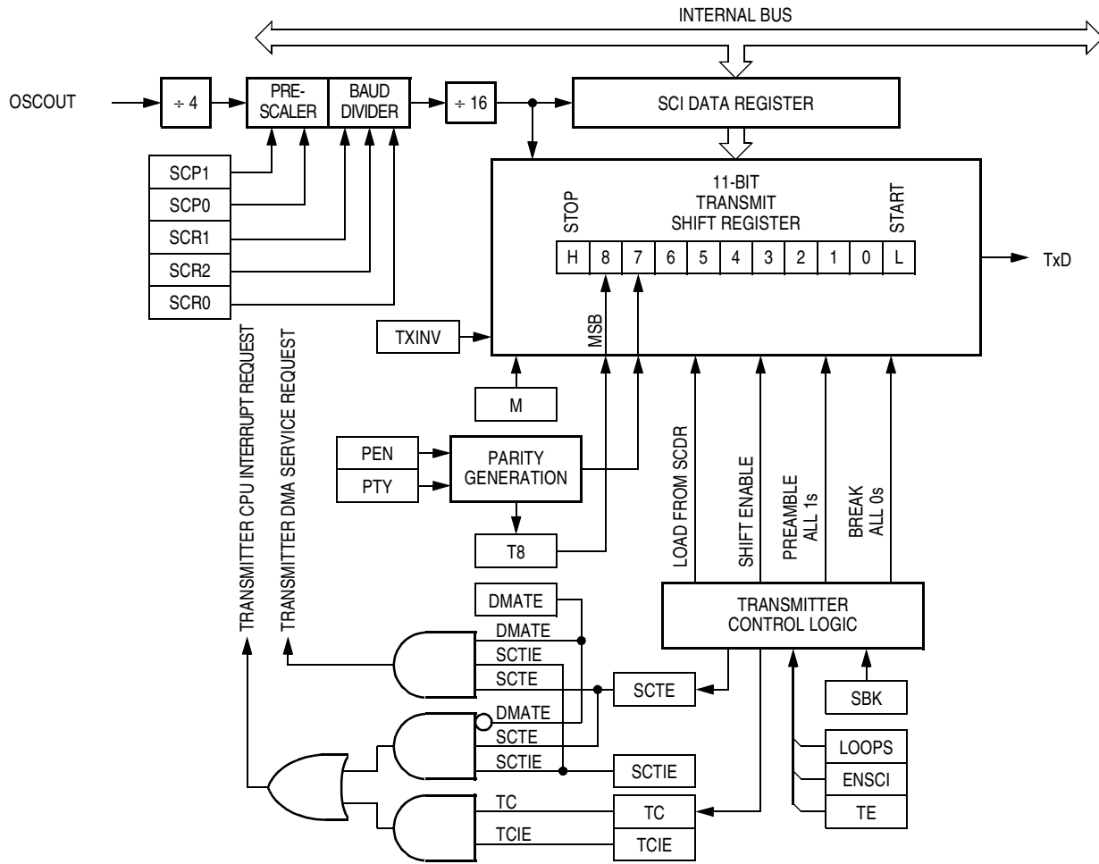
Figure 11-4. SCI Transmitter
