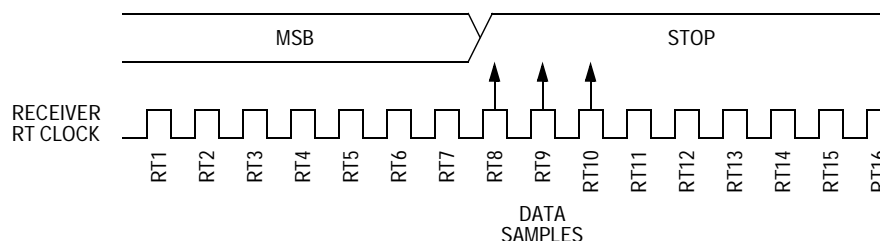
Figure 16-9. Slow Data
