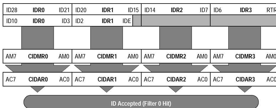
Figure 24-3. Single 32-Bit Maskable Identifier Acceptance Filter
