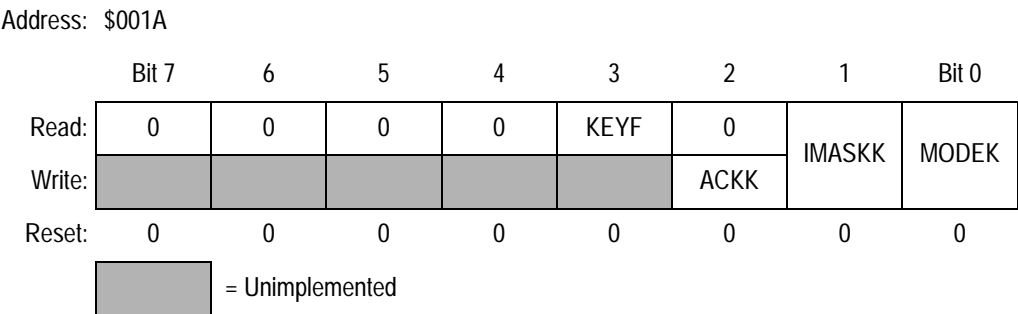
Figure 22-3. Keyboard Status and Control Register (KBSCR)
