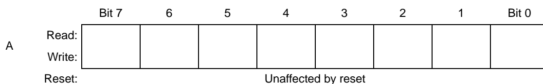
Figure 6-2. Accumulator (A)
