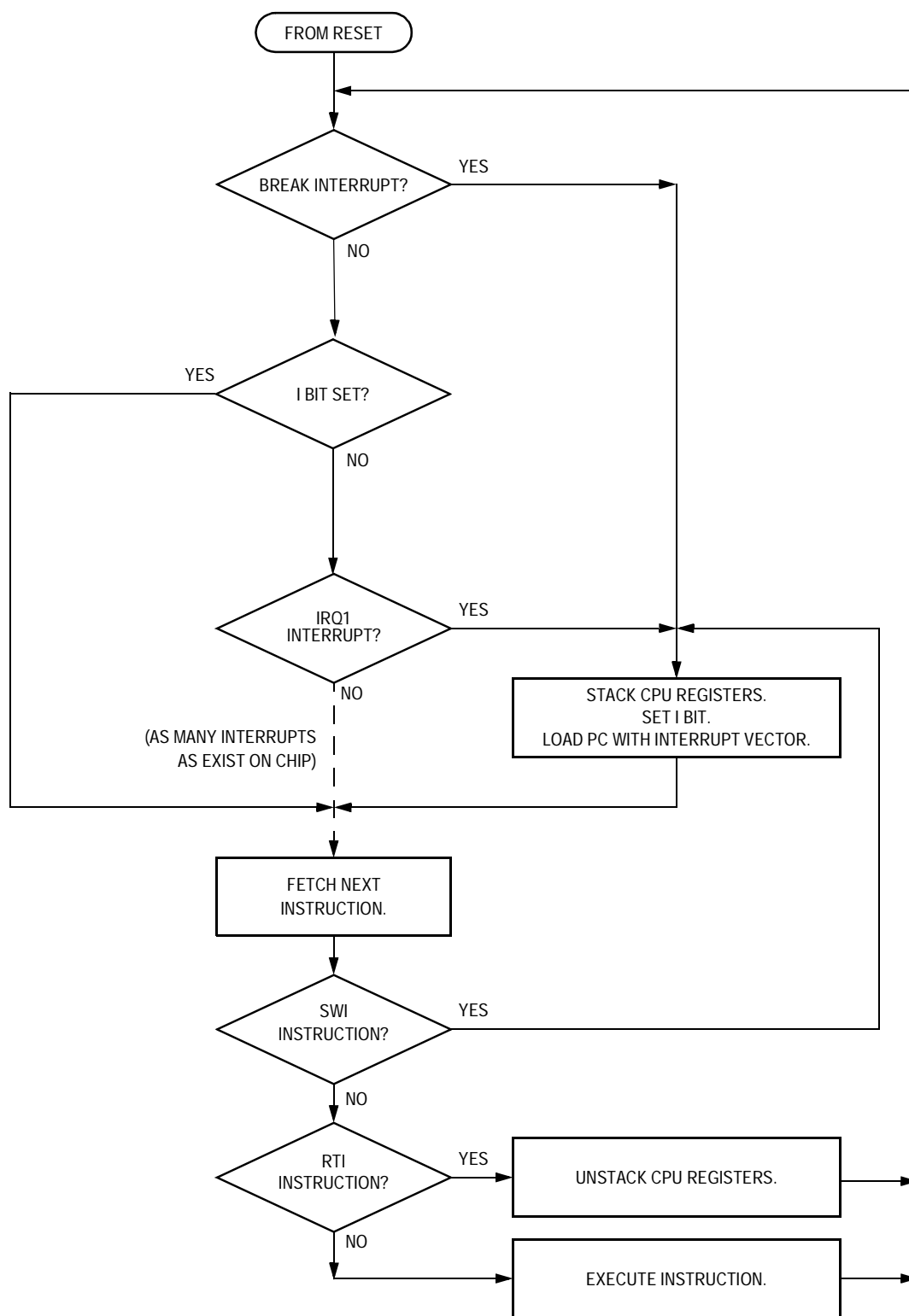
Figure 7-9. Interrupt Processing
