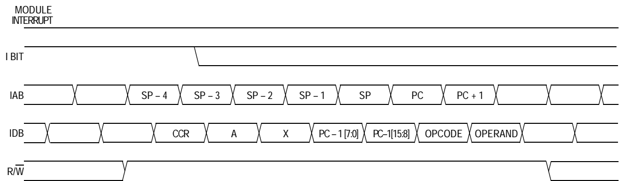
Figure 7-10. Interrupt Recovery
