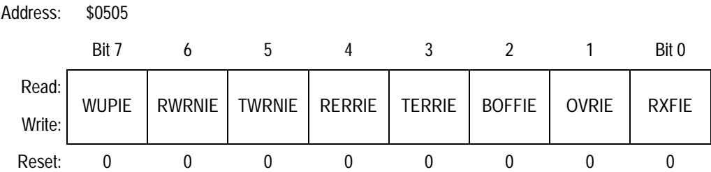
Figure 24-20. Receiver Interrupt Enable Register (CRIER)
