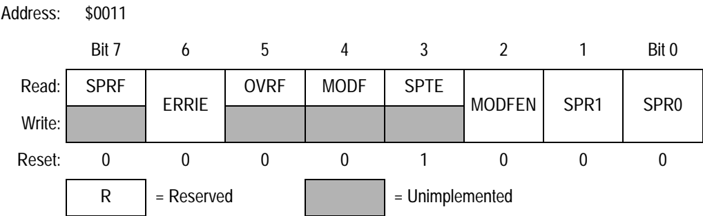
Figure 17-12. SPI Status and Control Register (SPSCR)
