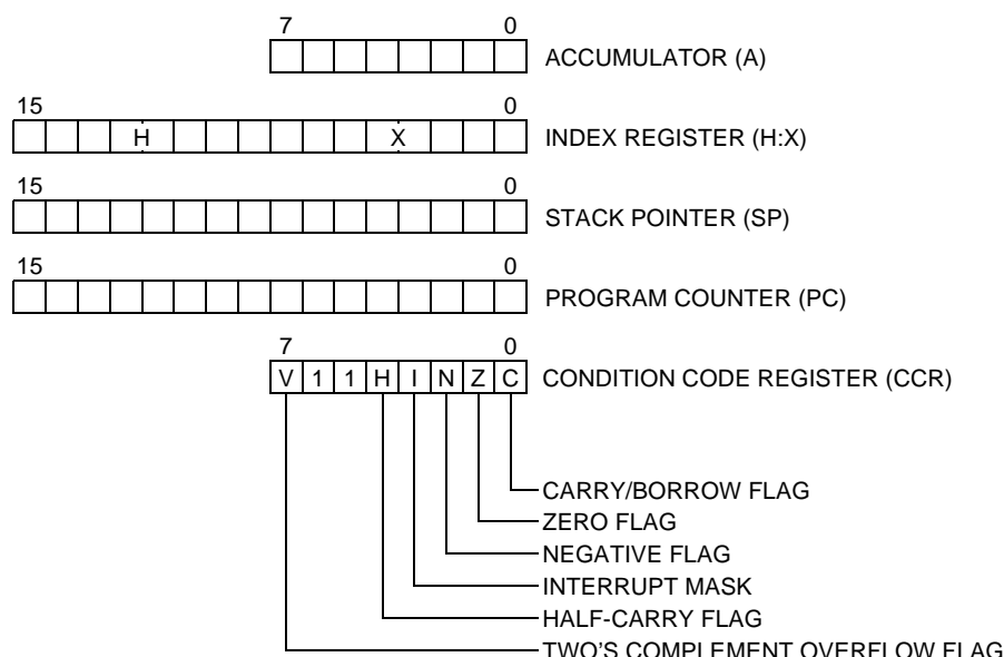
Figure 6-1. CPU registers
