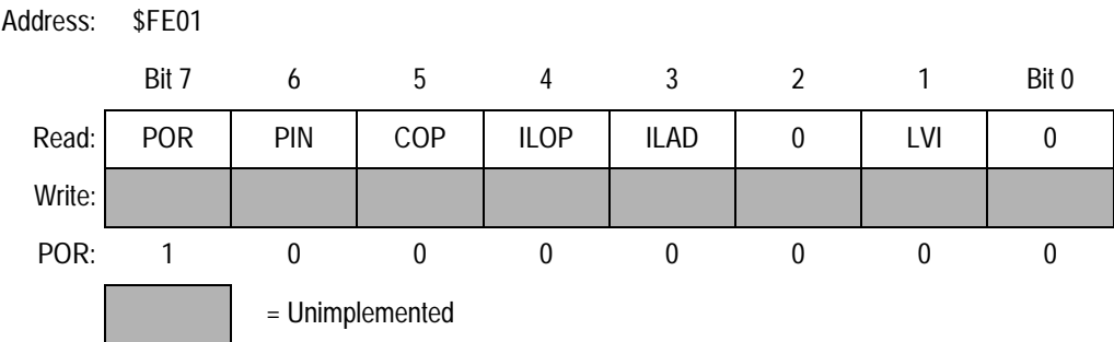
Figure 7-18. SIM Reset Status Register (SRSR)
