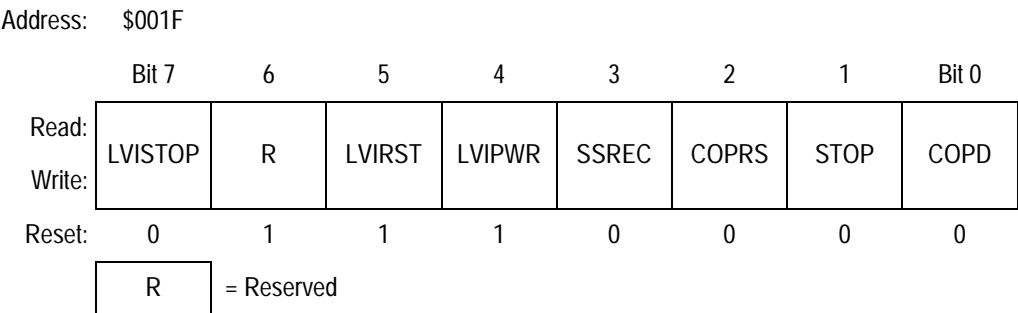
Figure 9-1. Configuration Register (CONFIG-1)
