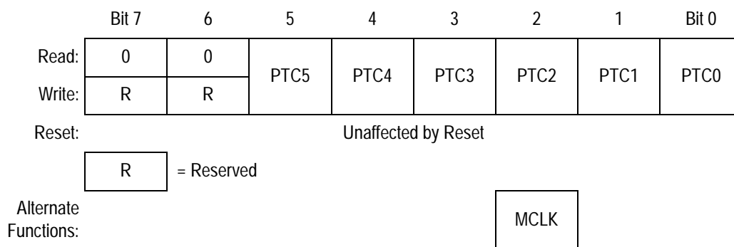
Figure 23-8. Port C Data Register (PTC)
