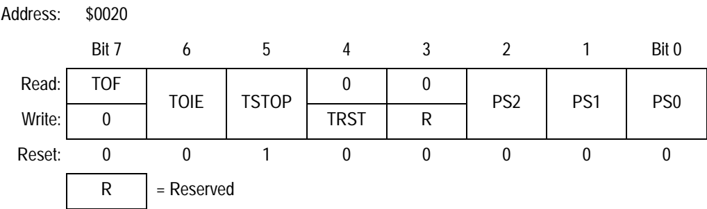
Figure 18-4. TIMA Status and Control Register (TASC)
