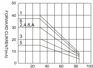
AMBIENT TEMPERATURE Ta(°C) FORWARD CURRENT VS. TEMPERATURE
