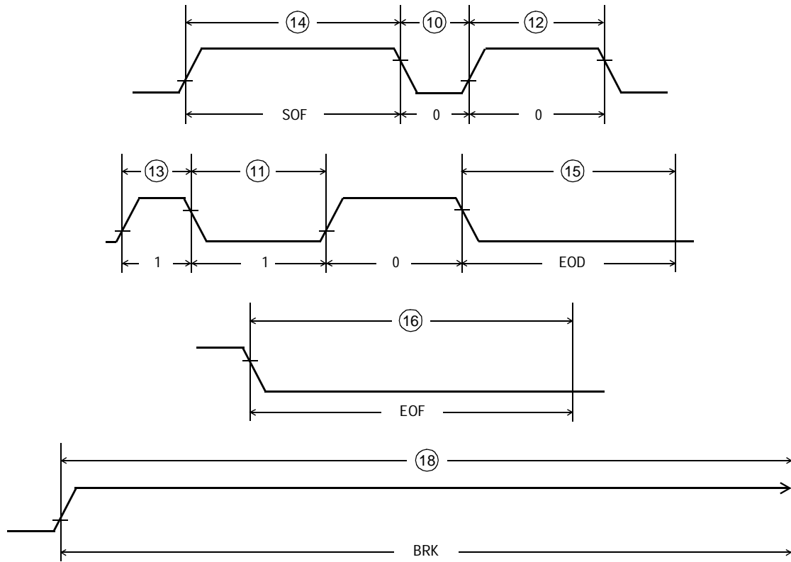
Figure 24-3. BDLC Variable Pulse-Width Modulation (VPW) Symbol Timing
