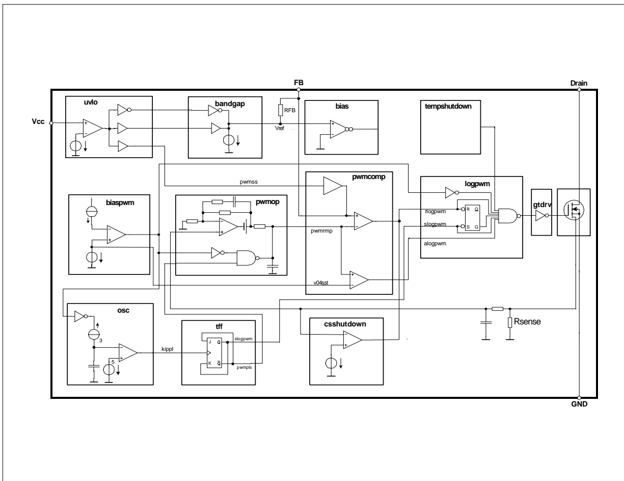
Figure 3 Block Diagram
