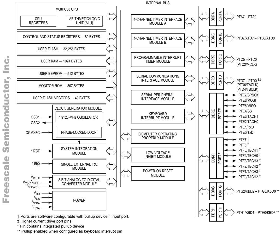
Figure 1-1. MC68HC908AB32 Block Diagram
