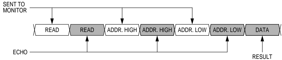
Figure 10-4. Read Transaction
