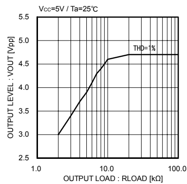
Fig.12 Delay side output load drive characteristic
