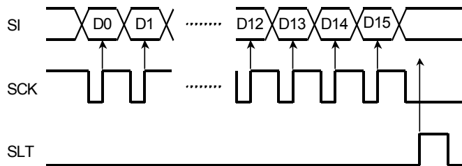
Fig.33 Serial interface specification
