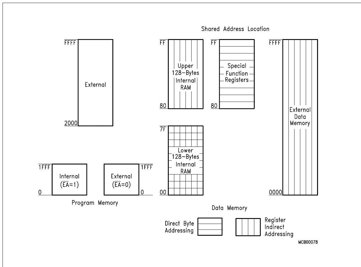
Figure 2 Memory Mapping
