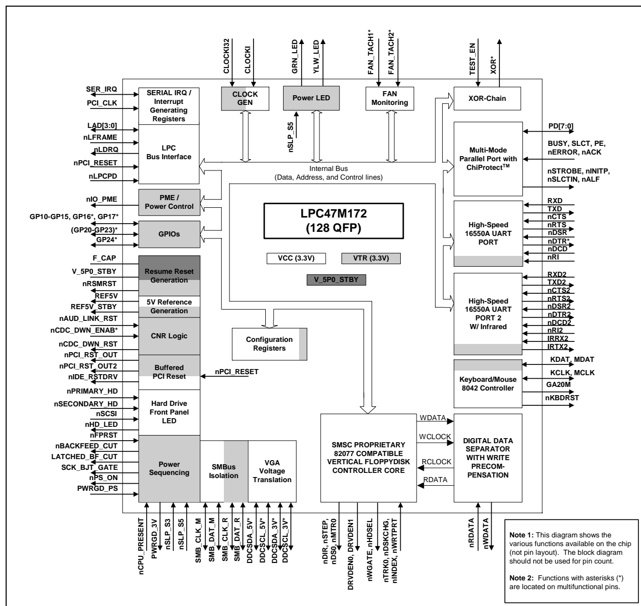
Figure 4.1 - LPC47M172 Block Diagram
