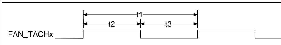
Figure 13.23 - Fan Tachometer Input Timing
