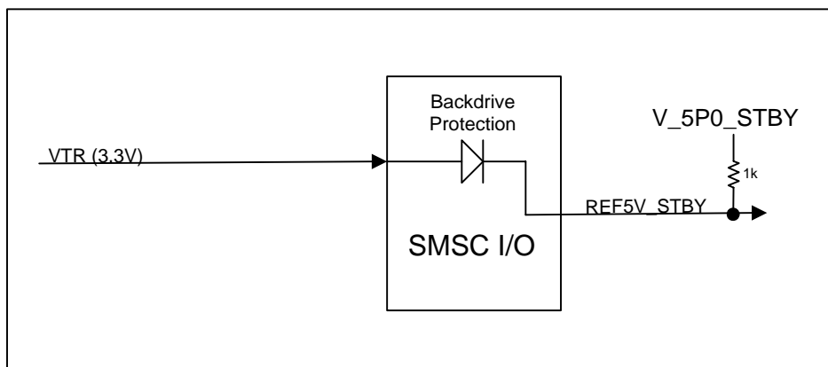
Figure 7.9 - REF5V_STBY
