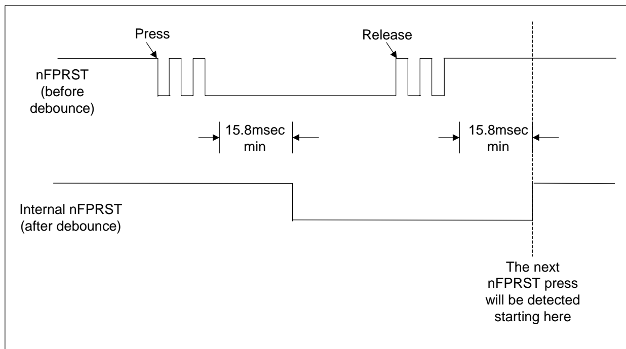
Figure 7.14 - NFPST Timing
