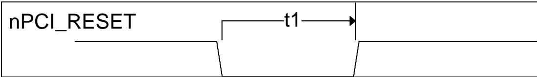
Figure 13.4 - Reset Timing
