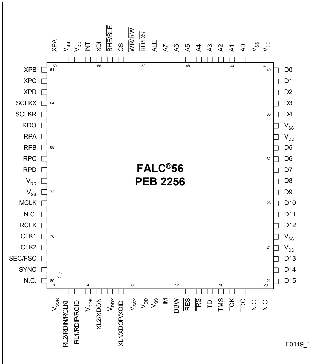
Figure 4 Pin Configuration P-MQFP-80-1
