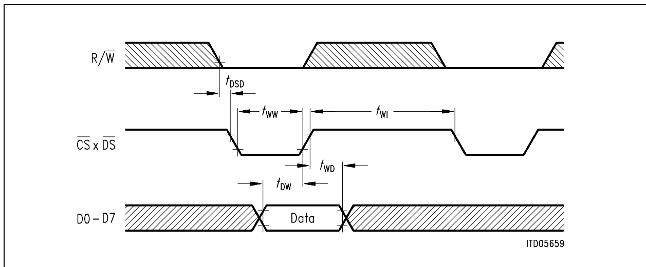
Figure 93 Microprocessor Write Cycle
