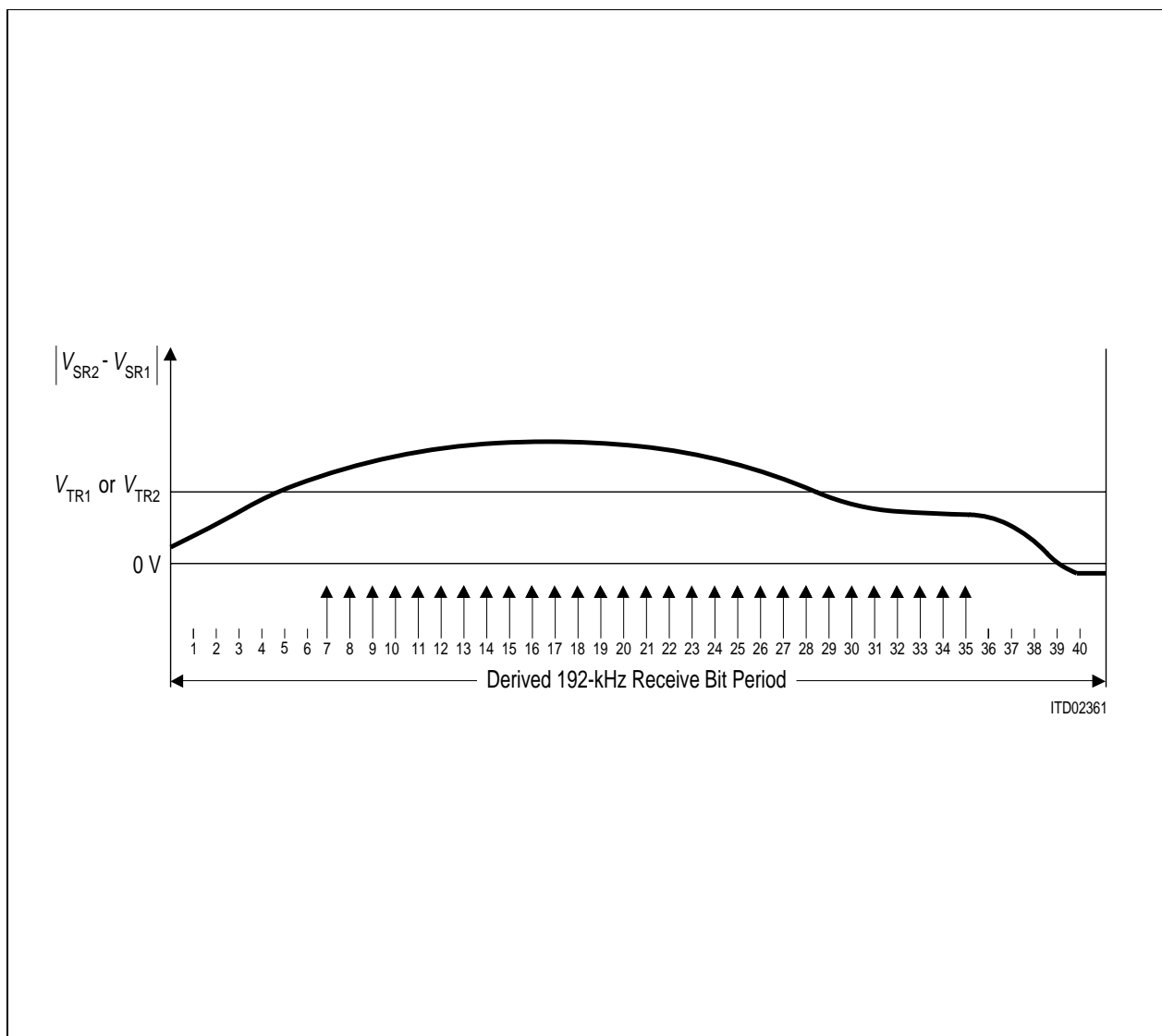
Figure 50 S/T Receive Signal Oversampling
