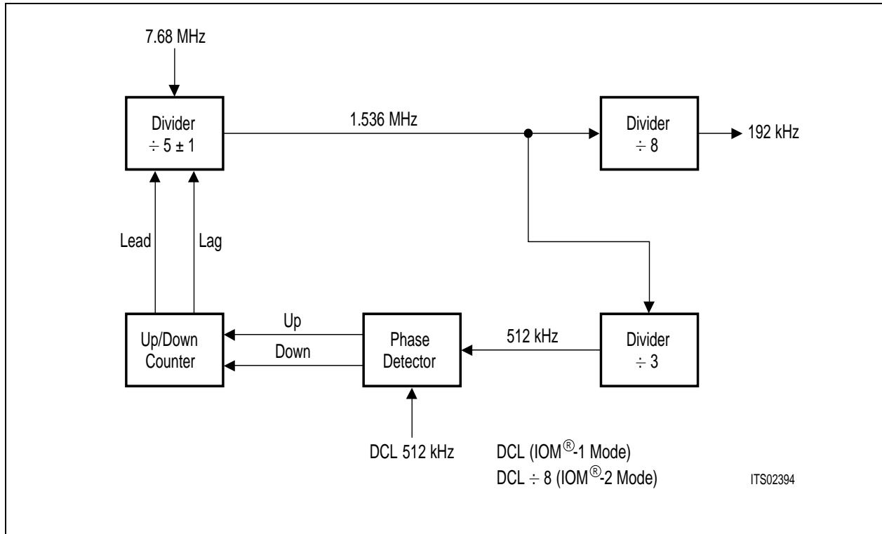
Figure 104 Block Diagram of XPLL
