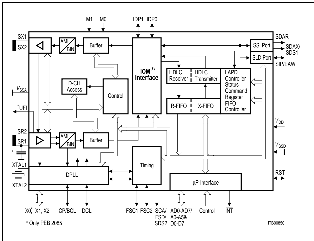
Figure 10 Architecture of the ISAC ® -S
