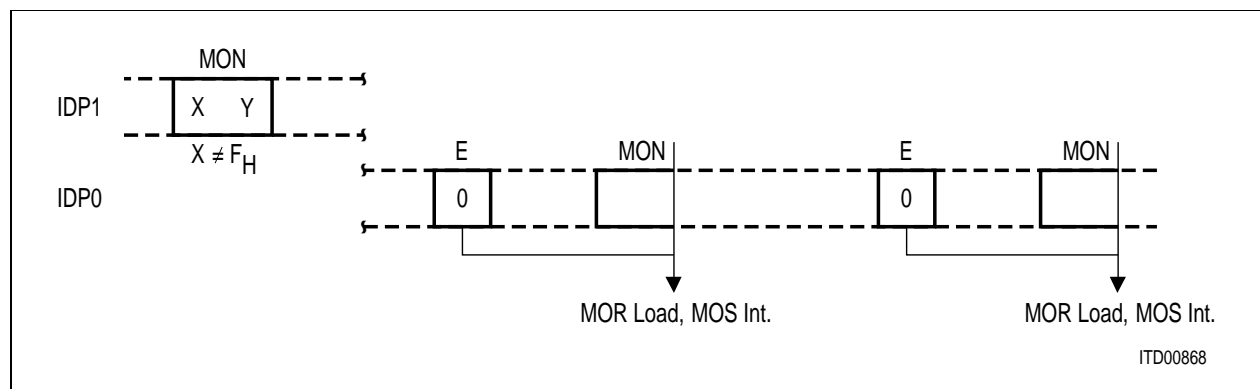
Figure 23 MONITOR Channel Protocol (IOM ® -1)
