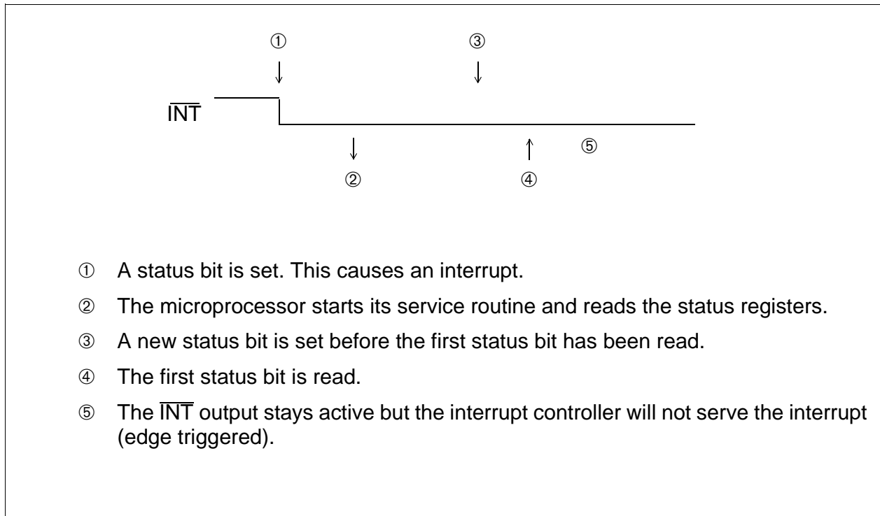
Figure 69 INT Handling
