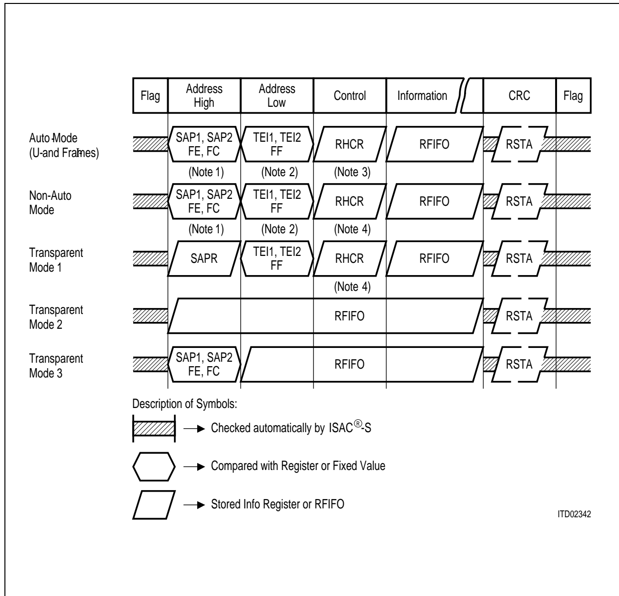
Figure 58 Receive Data Flow
