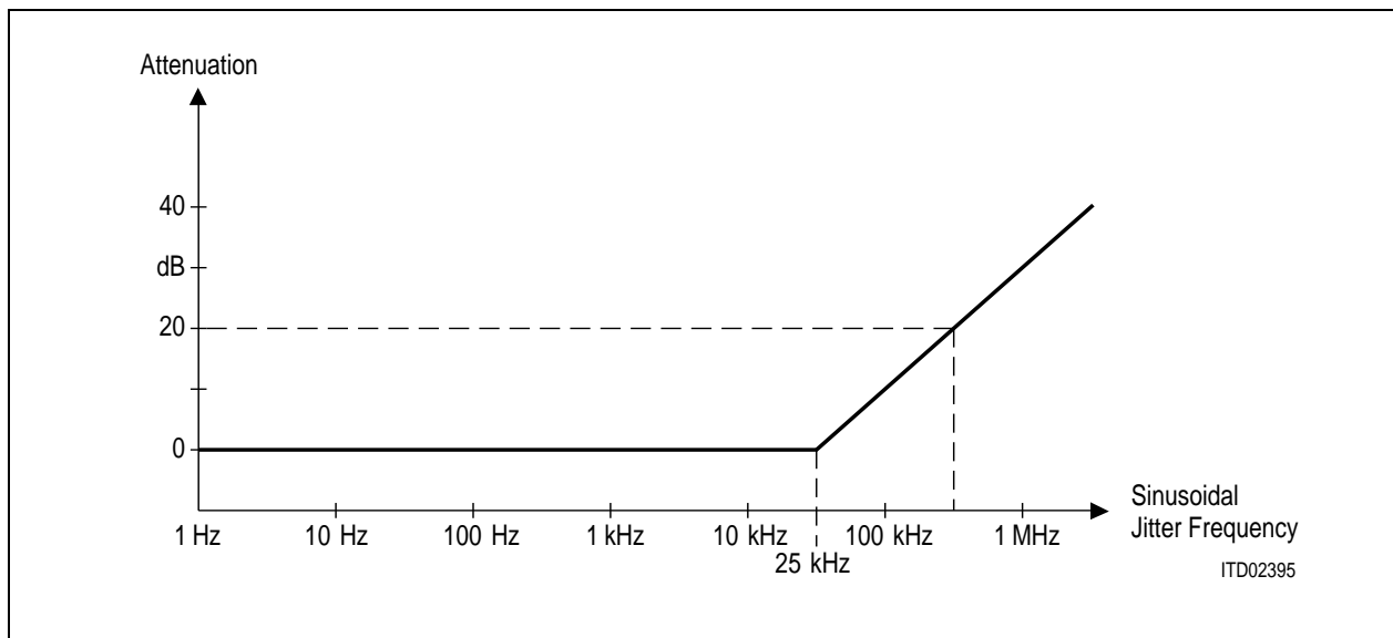
Figure 105 Jitter Transfer Curve of XPLL
