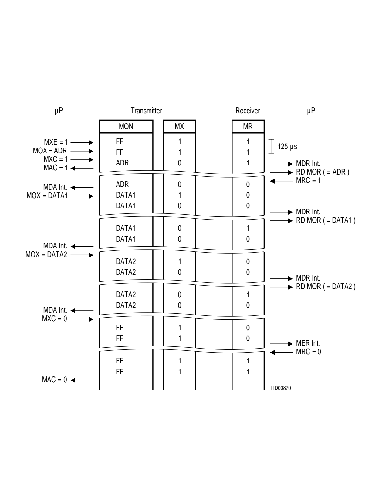
Figure 37 MONITOR Channel Protocol (IOM ® -2)
