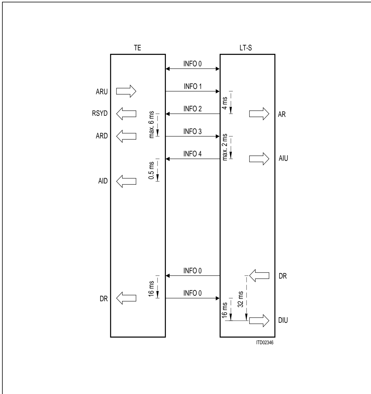
Figure 78 Example of Activation/Deactivation
