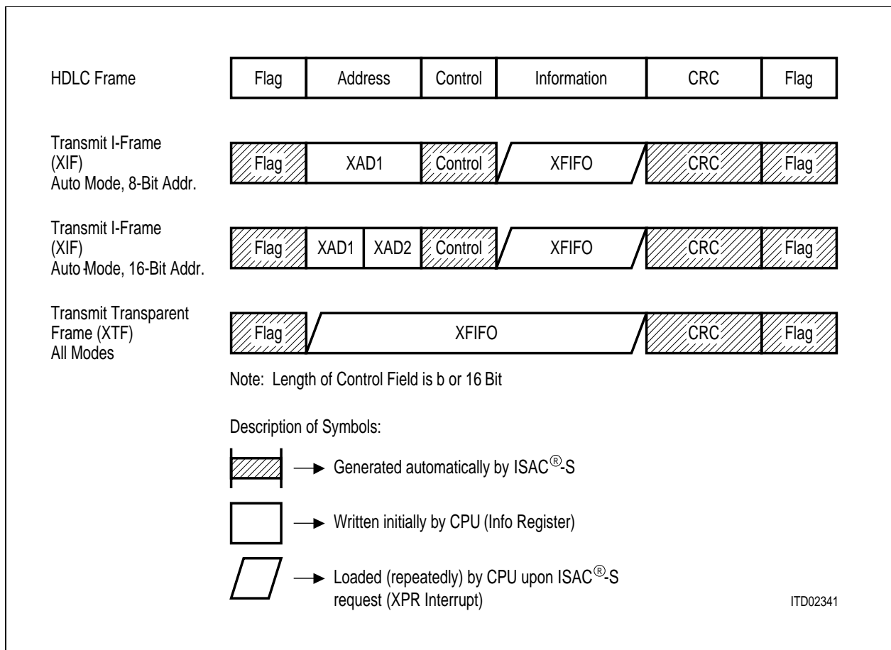
Figure 60 Transmitter Data Flow
