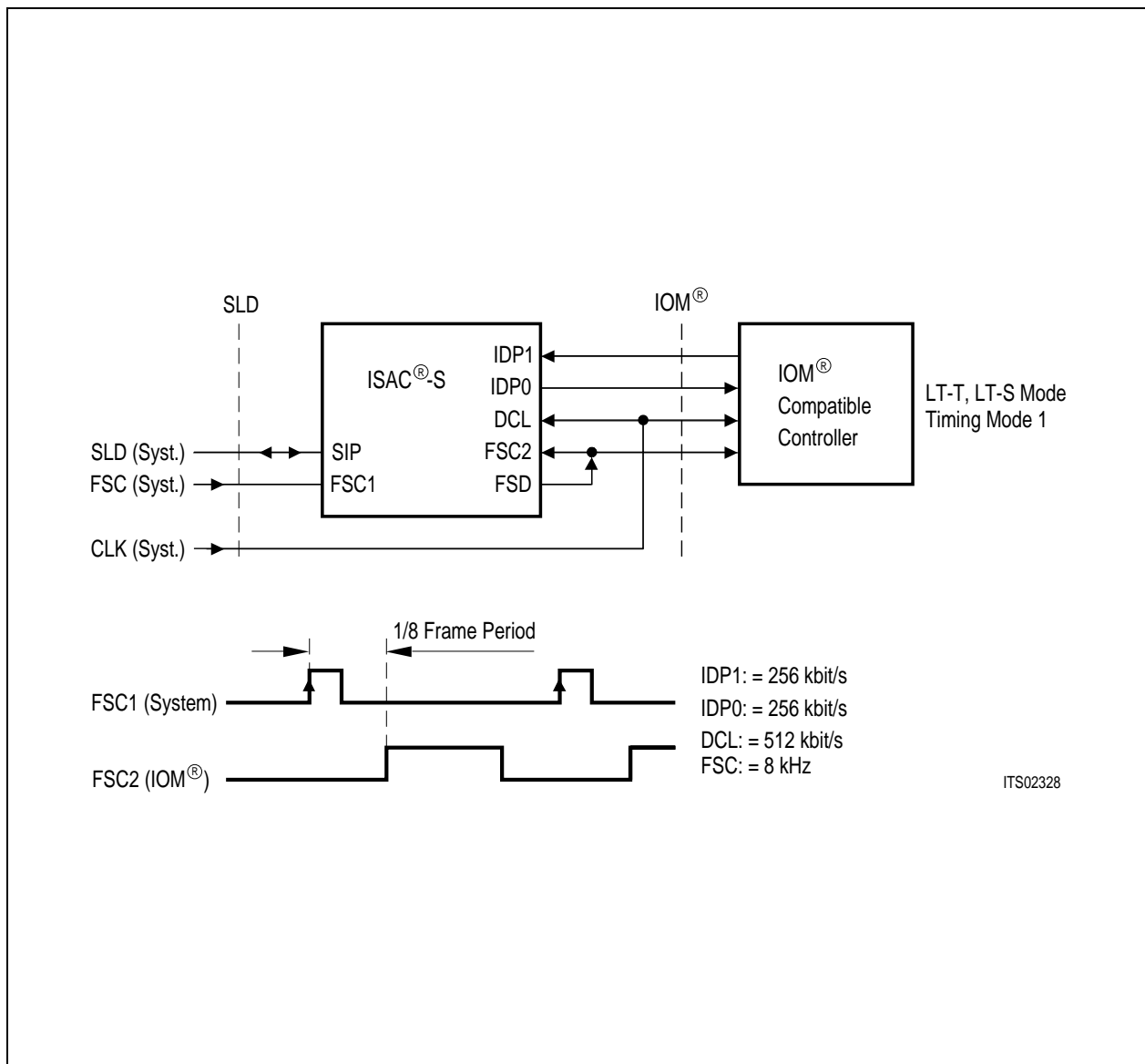
Figure 15 IOM ® -1 Interface Signals/Timing Mode 1
