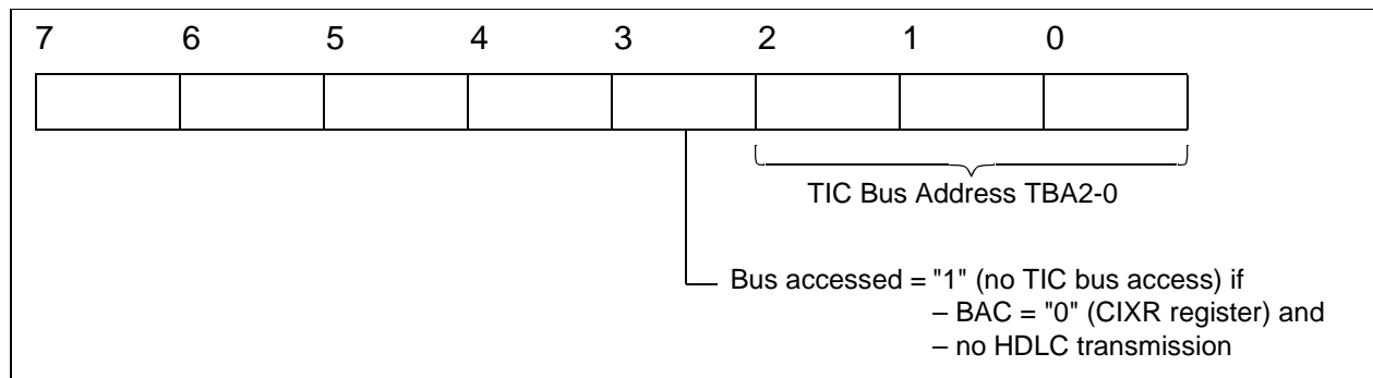
Figure 25 MONITOR Channel Structure on IDP1
