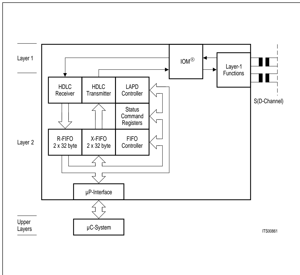
Figure 56 D-Channel Processing of the ISAC ® -S
