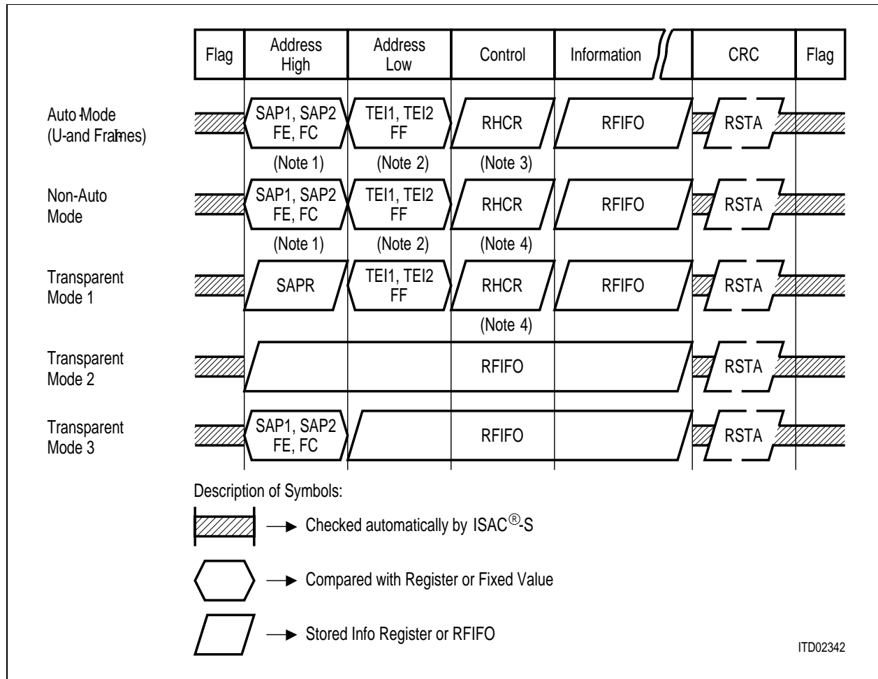
Figure 80 Receive Data Flow
