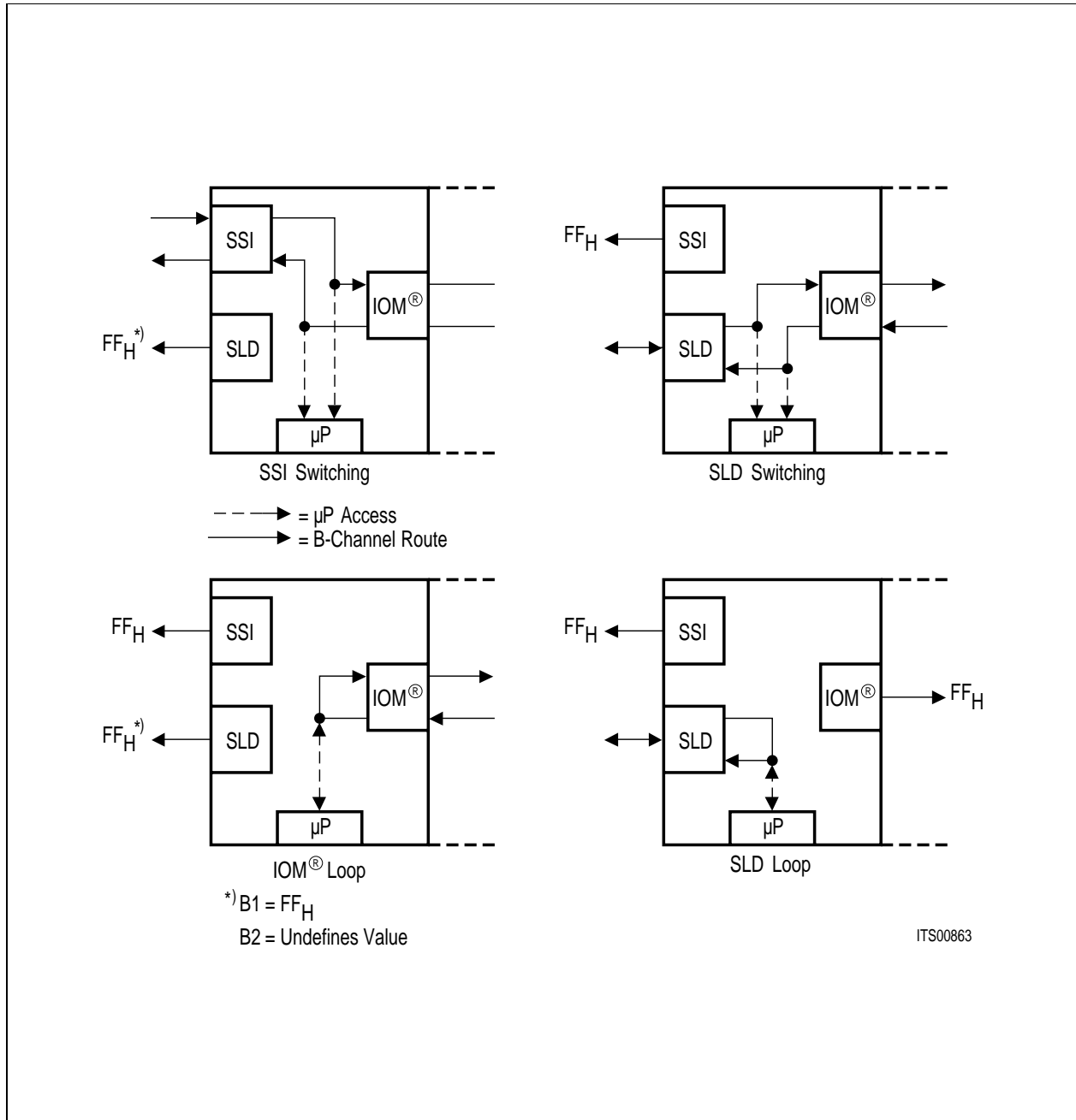
Figure 21 B-Channel Routes and Access to B-Channel Data
