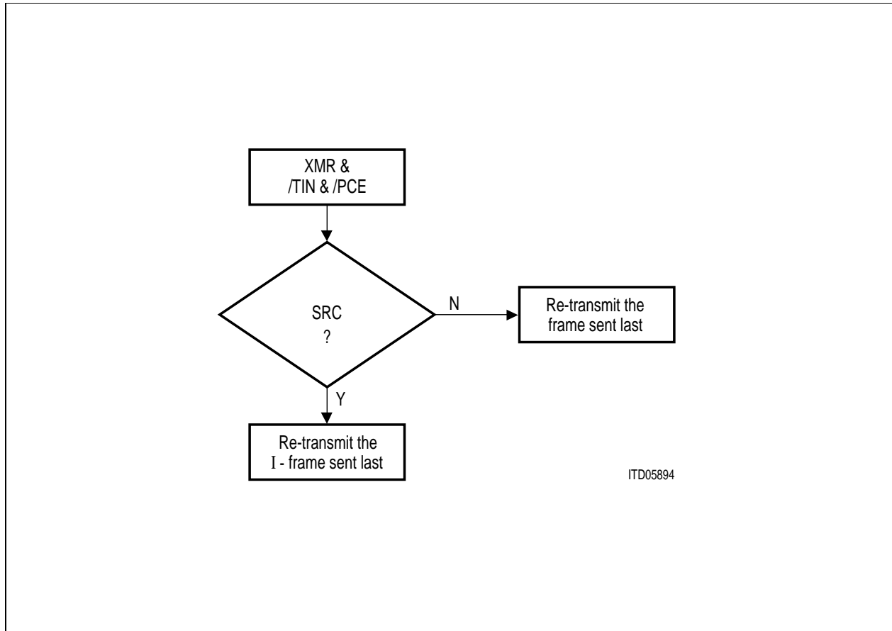
Figure 64 Interrupt Service Routine after XMR
