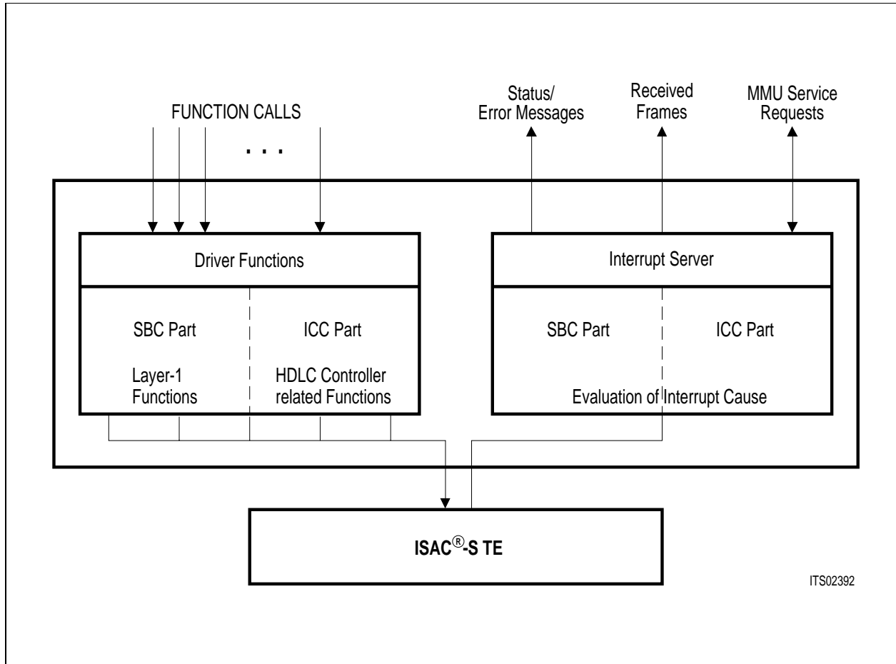
Figure 112 LLC Architecture
