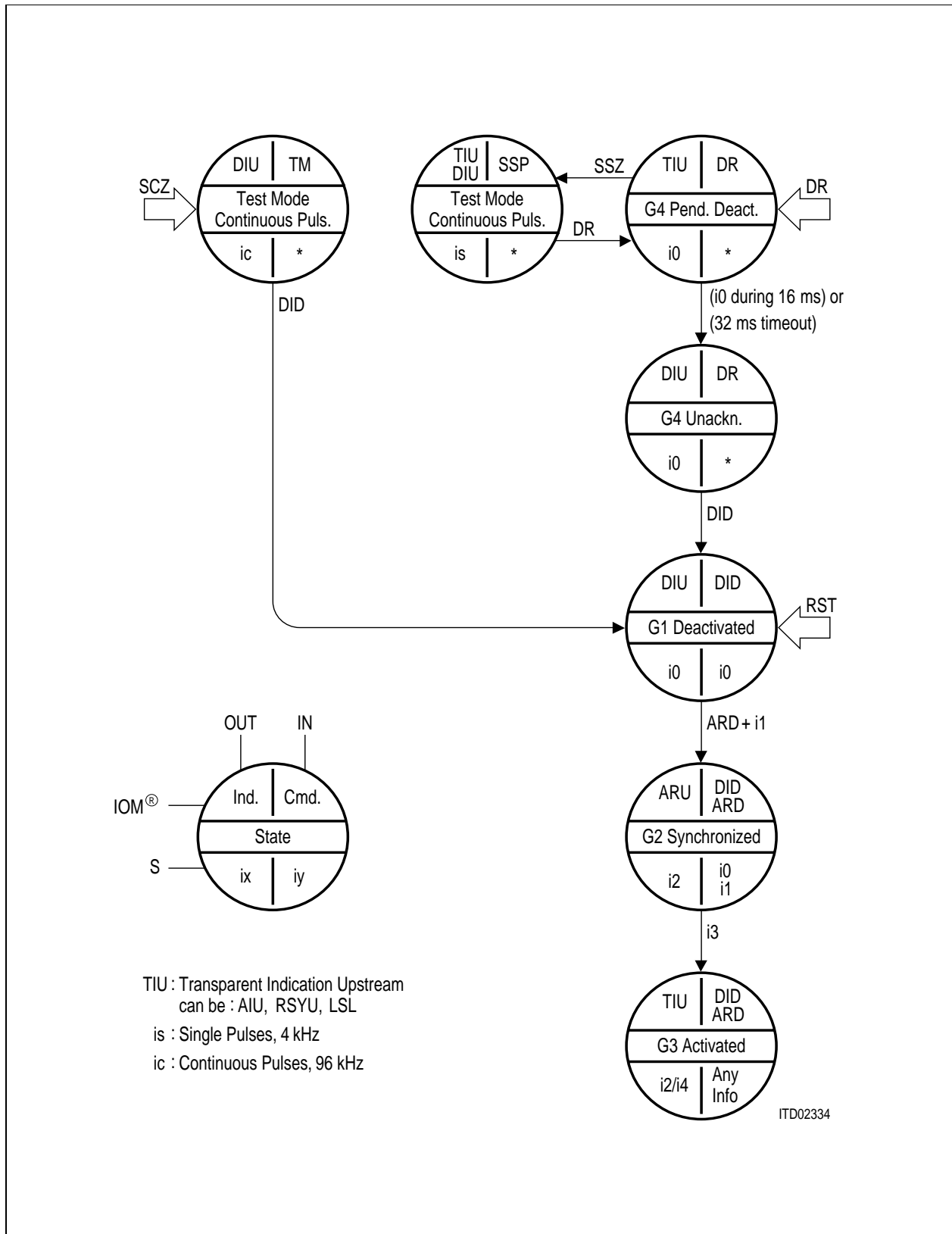
Figure 76 State Diagram of LT-S Mode
