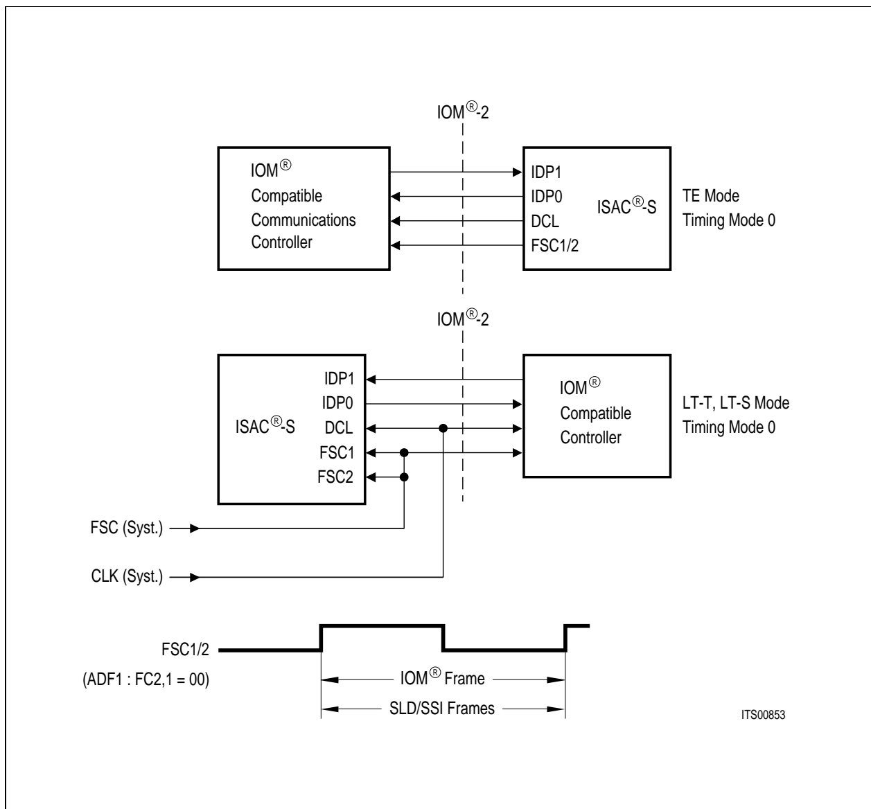
Figure 14 IOM ® -1 Interface Signals/Timing Mode 0
