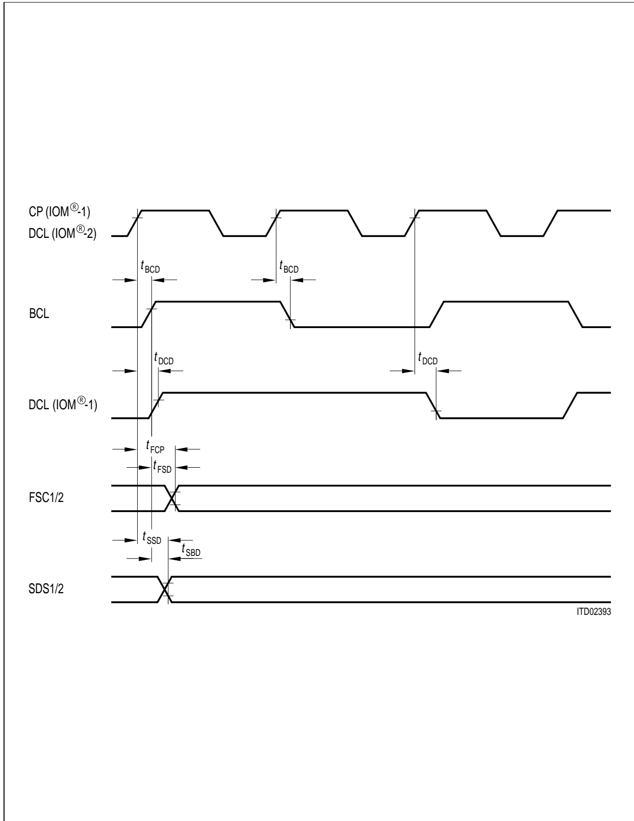
Figure 102 Timing Relationships between ISAC ® -S Clock Signals
