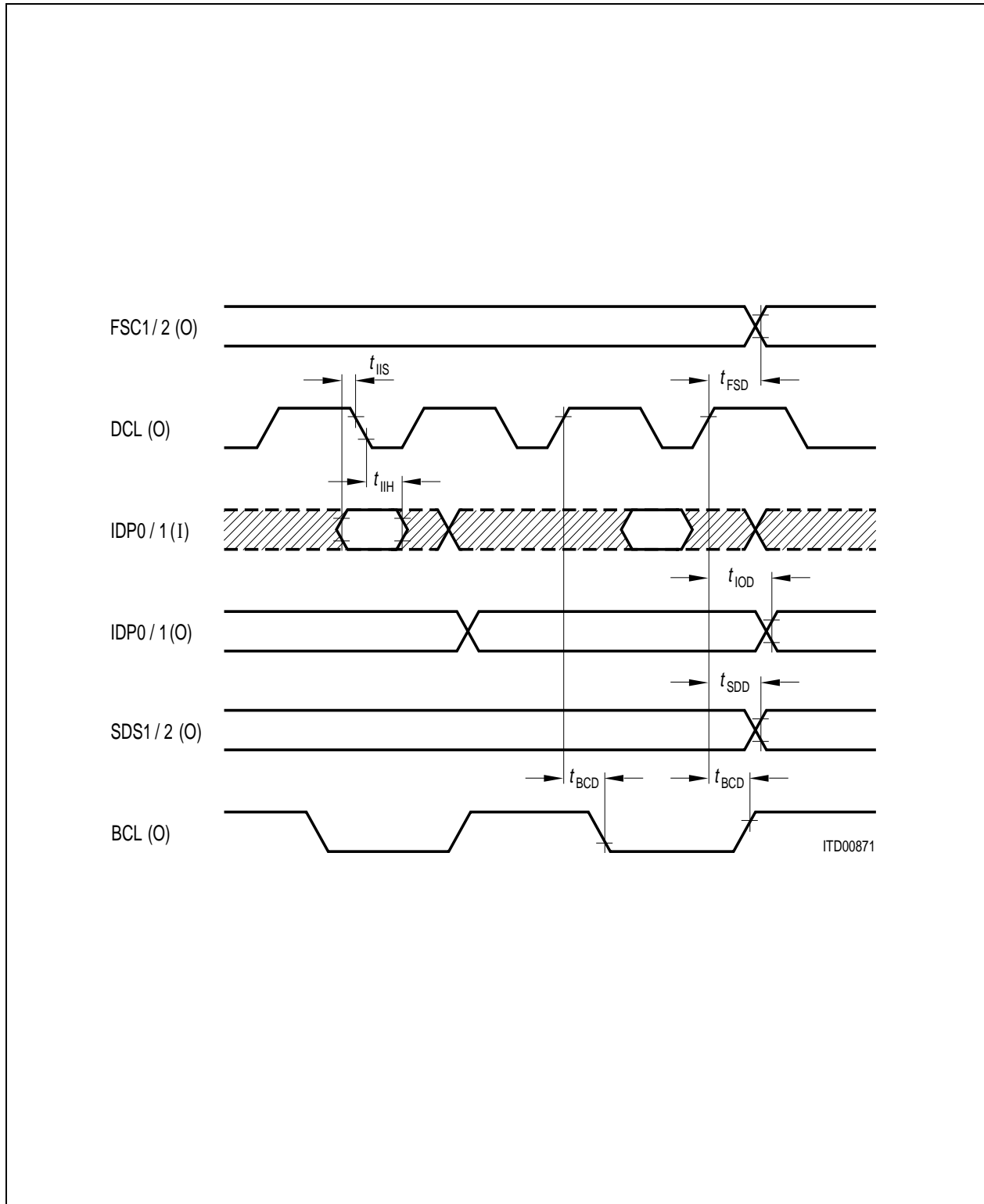
Figure 95 IOM® Timing (TE mode)
