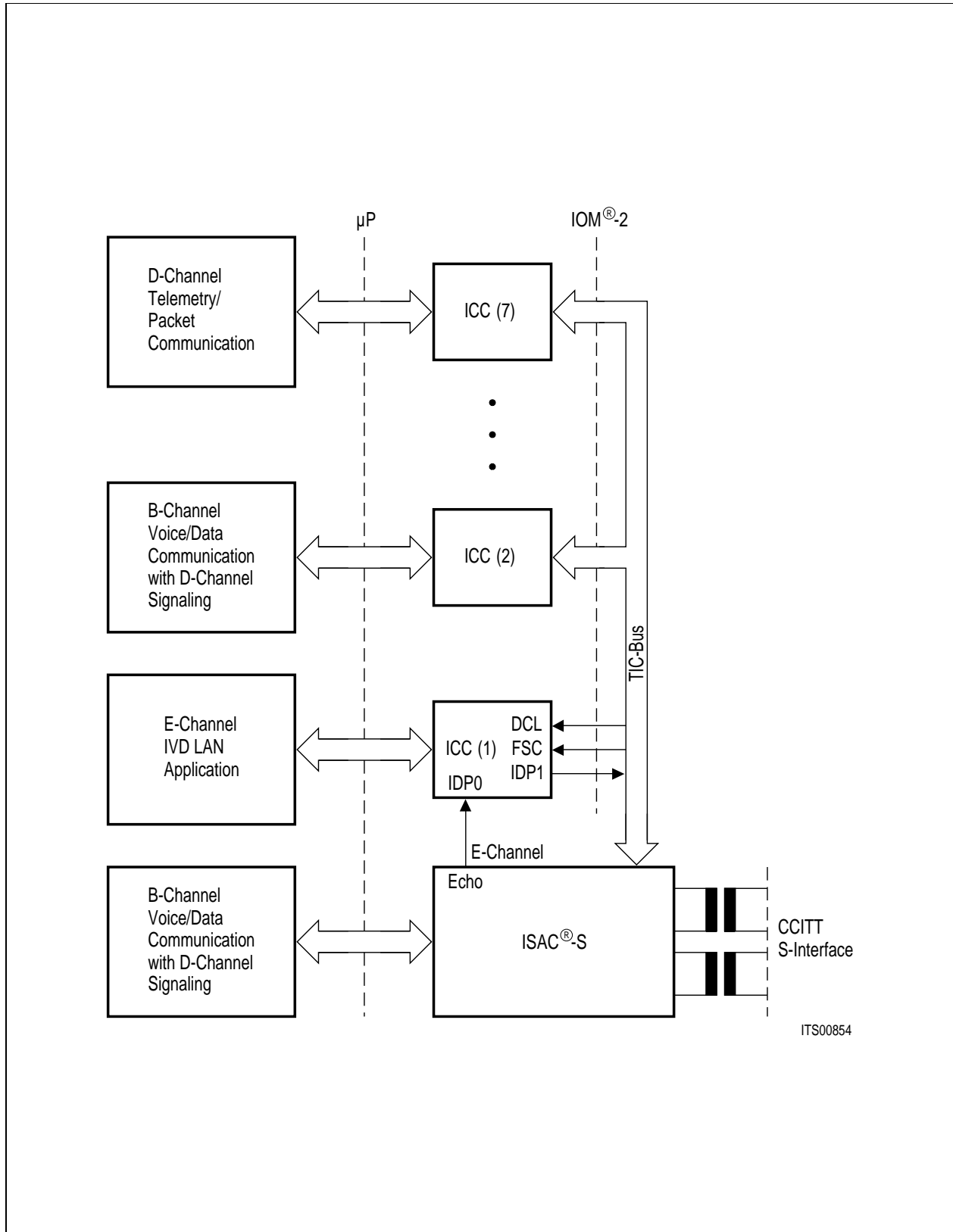
Figure 24 Applications of IOM ® Bus Configuration
