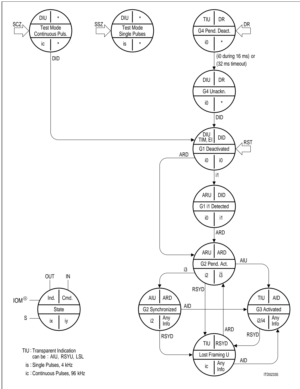
Figure 77 State Diagram of NT Mode
