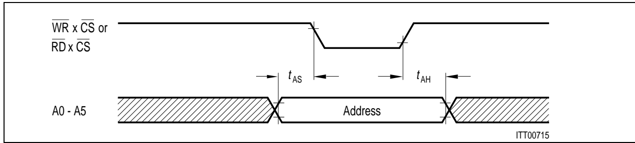
Figure 91 Non-Multiplexed Address Timing
