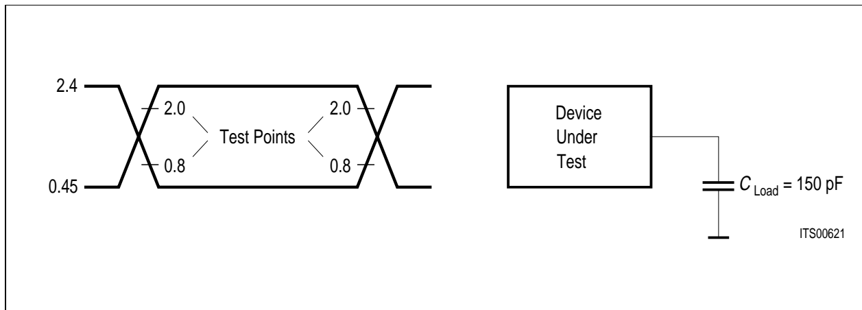
Figure 87 Input/Output Waveform for AC Tests
