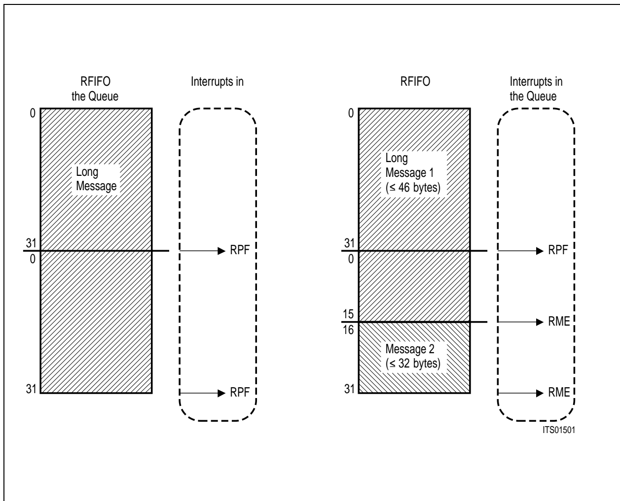
Figure 59 Contents of the RFIFO (long messages)
