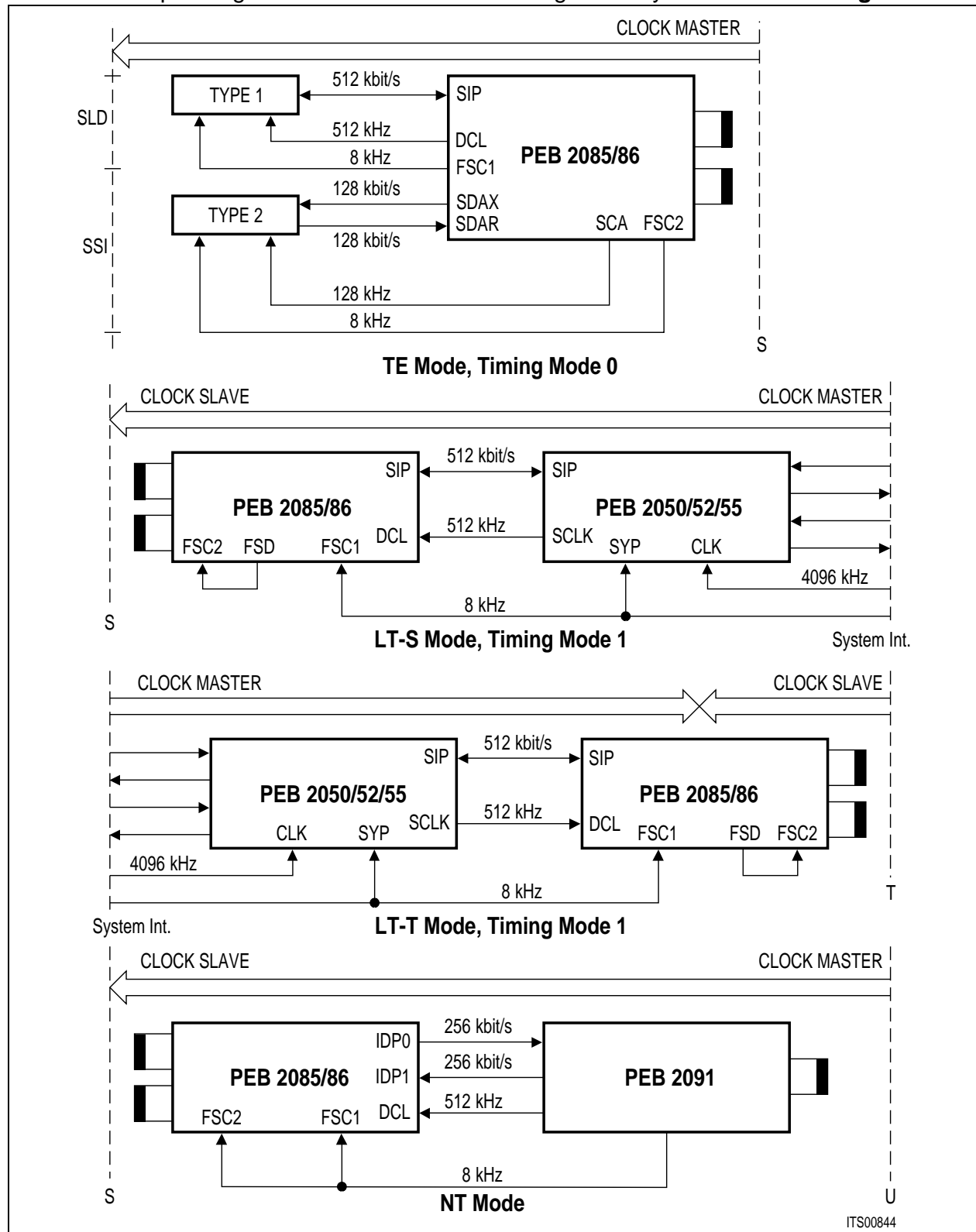
Figure 11 Operating Modes of the ISAC ® -S (IOM ® -1)
