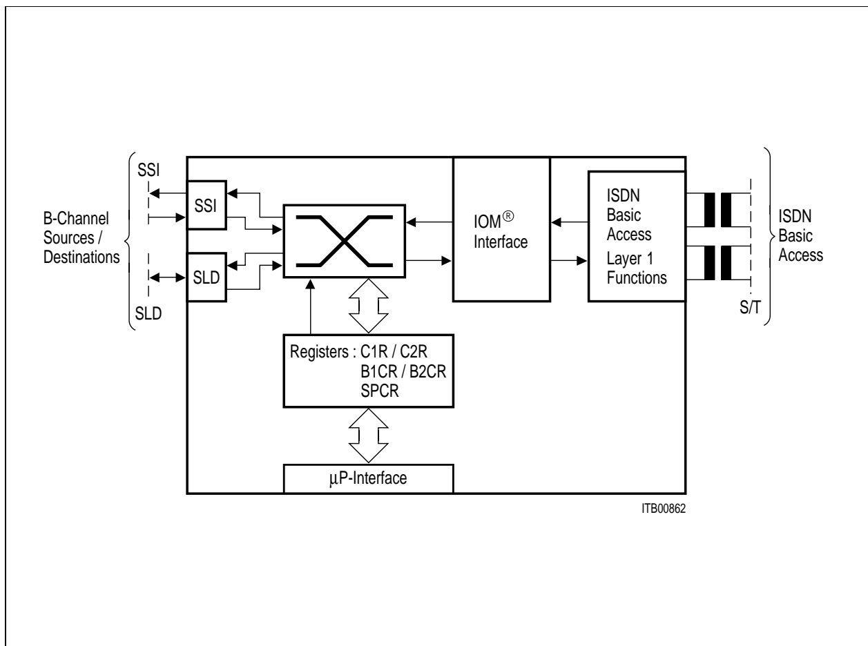
Figure 20 Principle of B-Channel Switching
