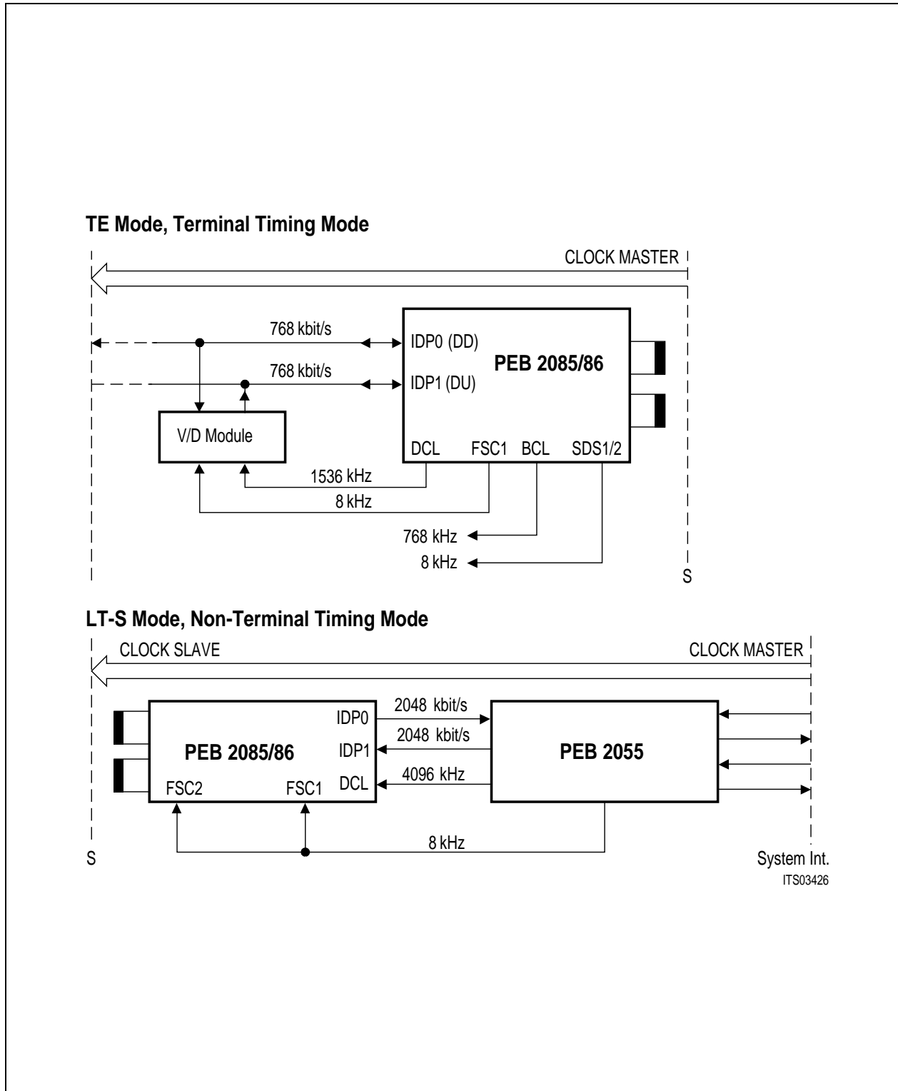
Figure 12a Operating Modes of ISAC ® -S (IOM ® -2)
