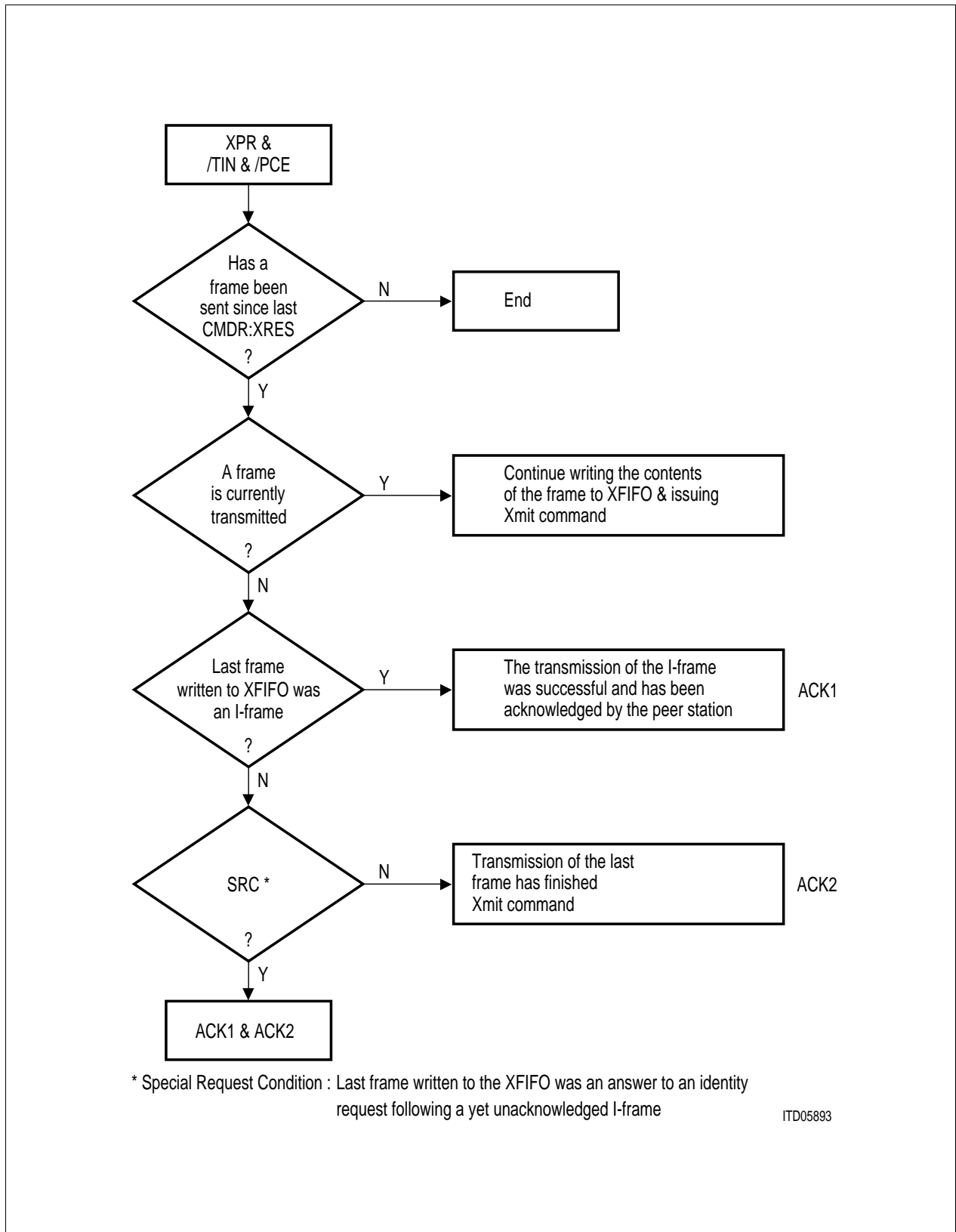
Figure 63 Interrupt Service Routine after XPR
