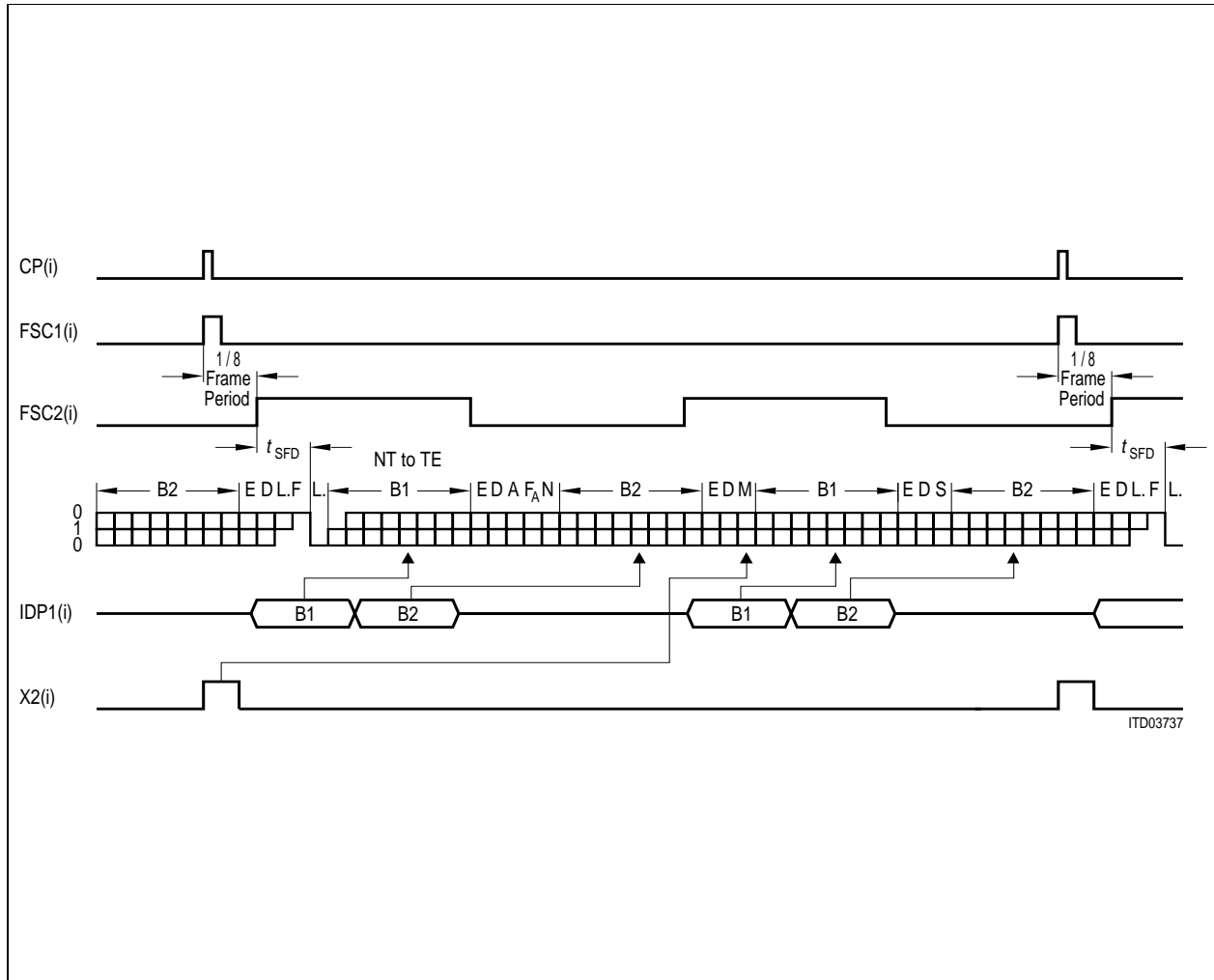
Figure 110 Frame Relationship in Timing Mode 1
