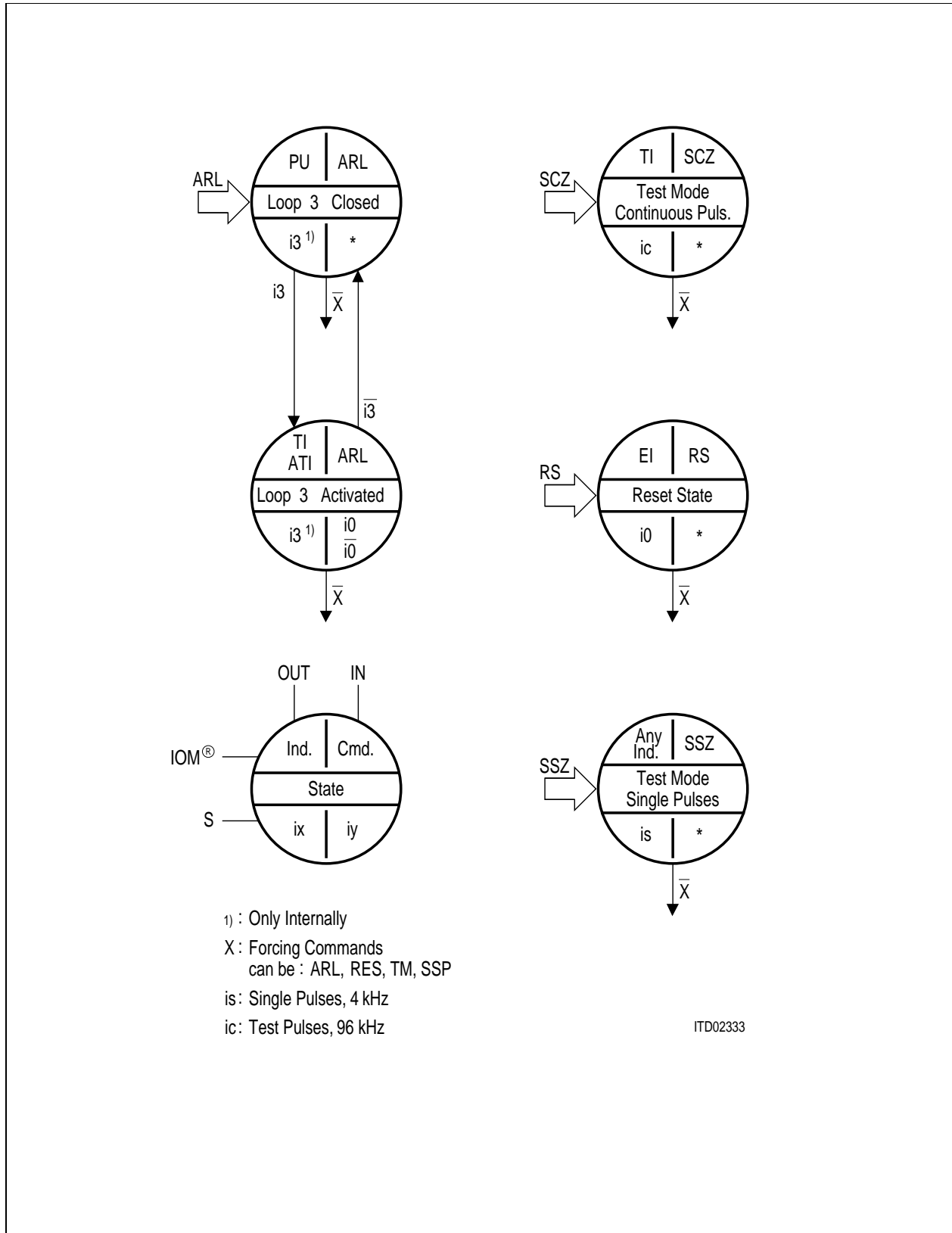
Figure 75b State Diagram of TE/LT-T Mode: Unconditional Transitions
