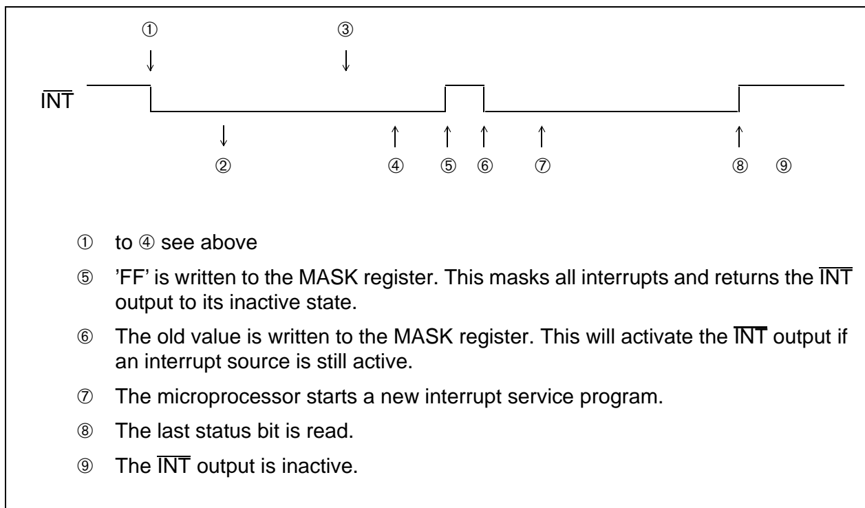
Figure 70 Service Program for Edge-Triggered Interrupt Controllers
