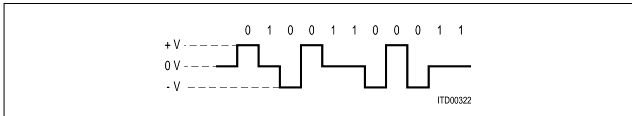
Figure 42 S/T Interface Line Code
