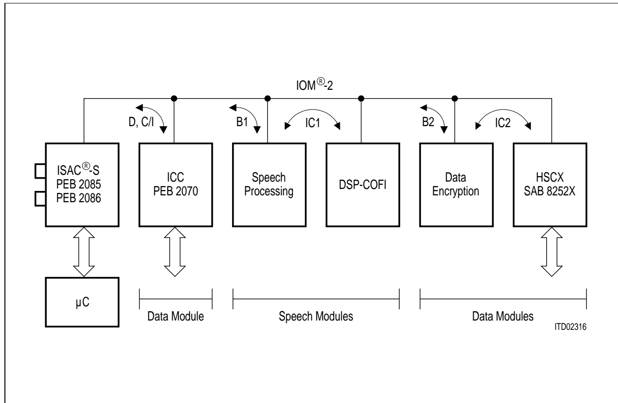
Figure 6 Example of an ISDN ® -S Voice/Data Terminal
