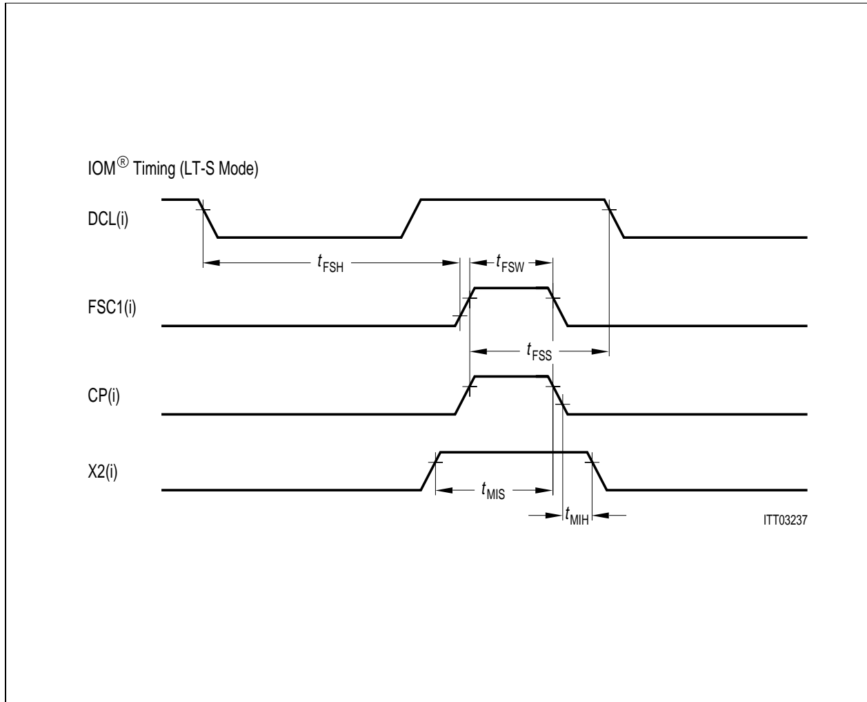
Figure 107 External Trigger for the S-Frame Synchronization
