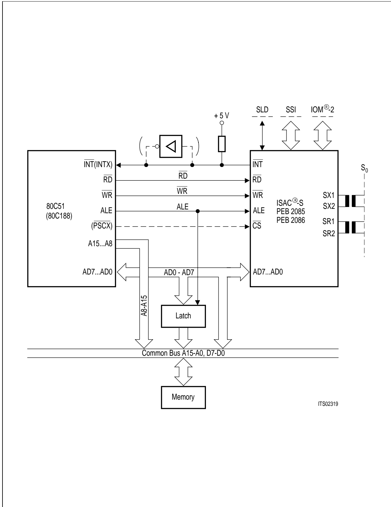
Figure 9 Connecting the ISAC ® -S to Siemens/Intel Microcontroller
