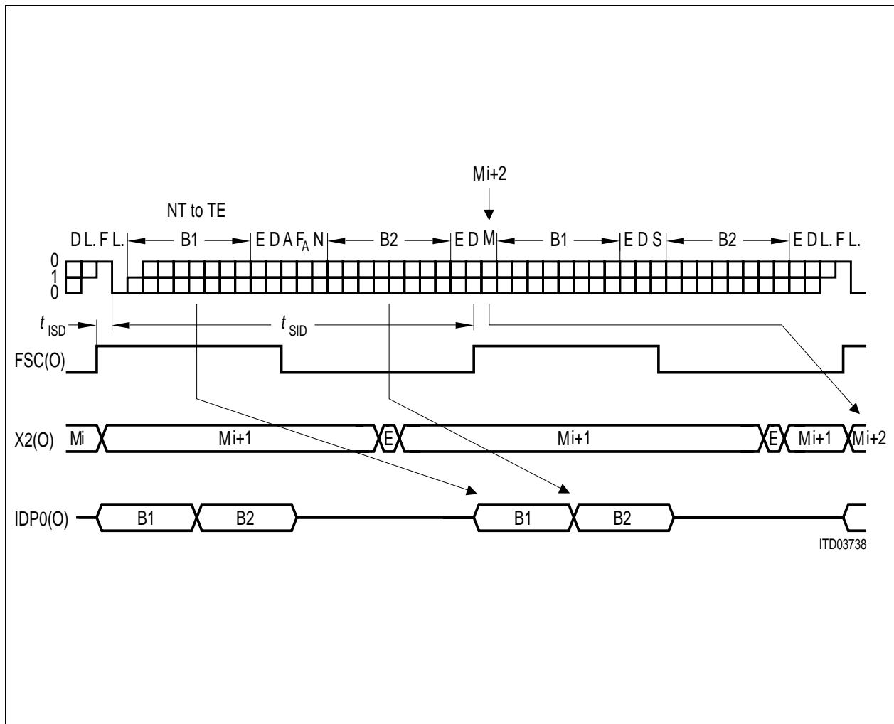
Figure 111 Frame Relationship in TE-Mode
