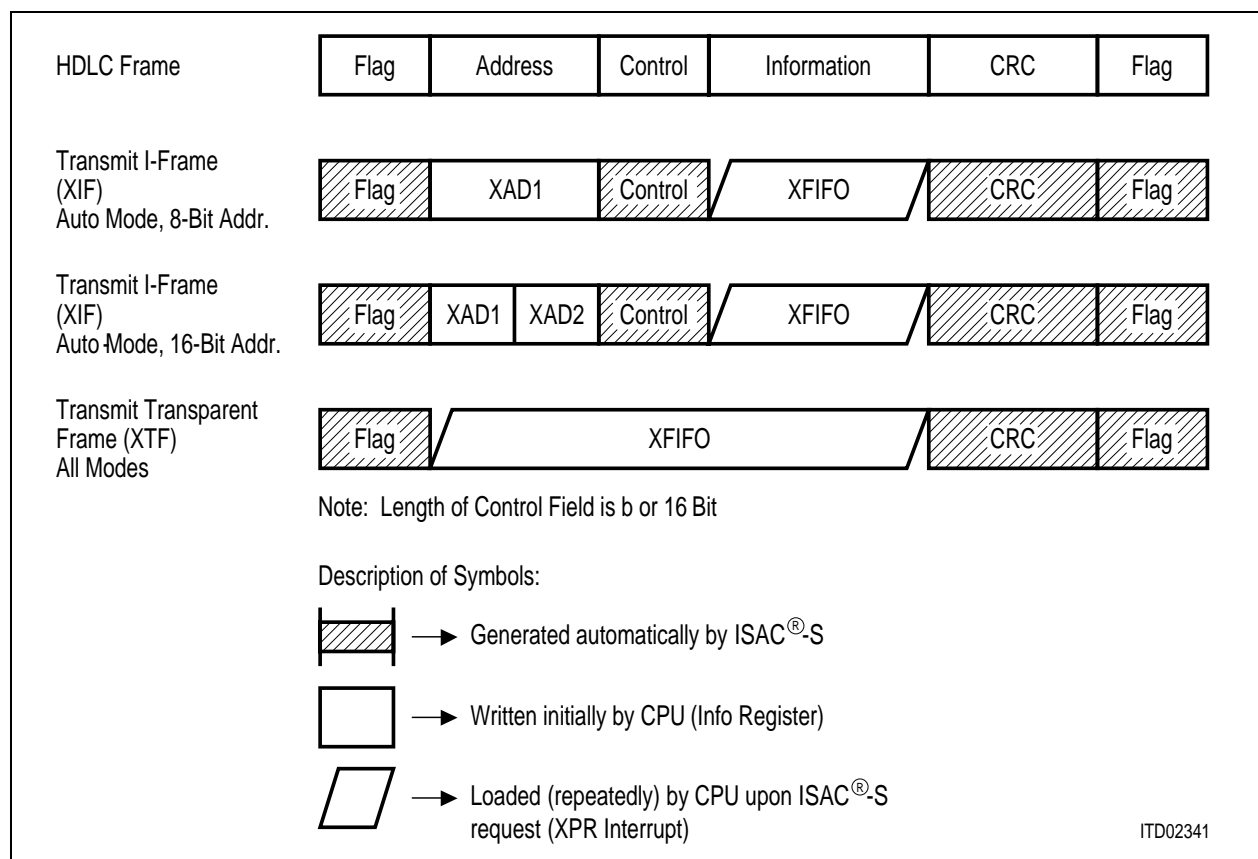
Figure 81 Transmit Data Flow
