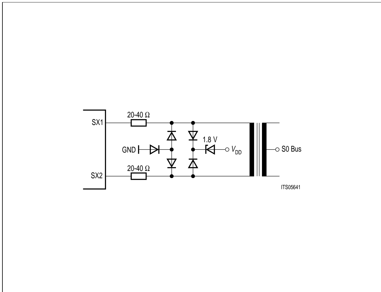
Figure 47 External Circuitry for Transmitters
