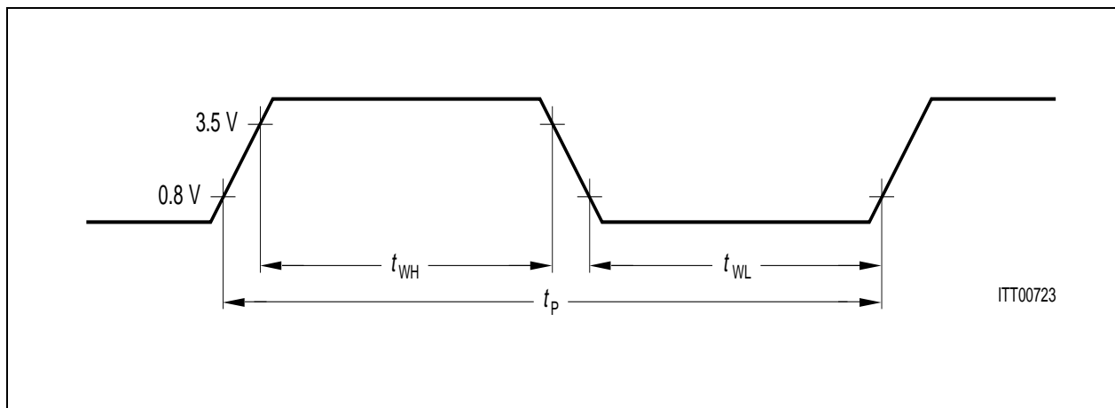
Figure 103 Definition of Clock Period and Width
