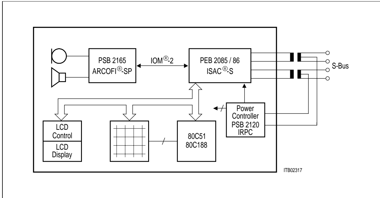
Figure 7 Basic ISDN Feature Telephone
