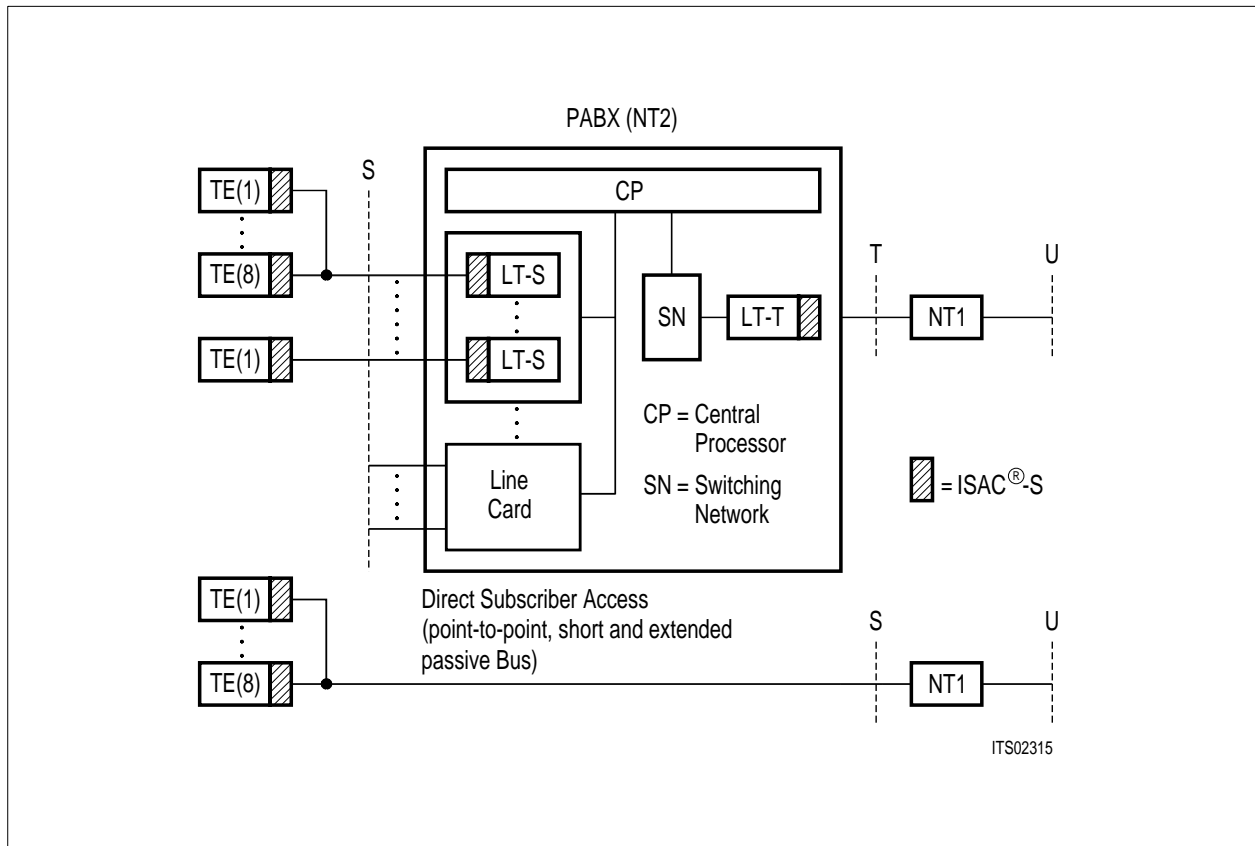
Figure 5 Applications of the ISAC®-S (ISDN Basic Access)
