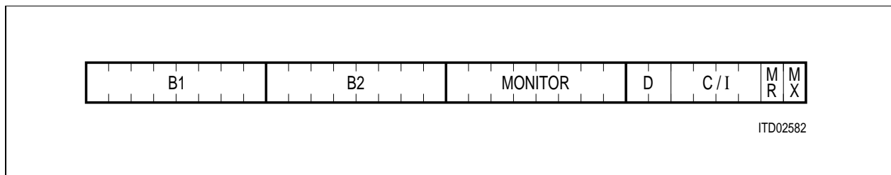
Figure 27 Channel Structure of IOM ® -2
