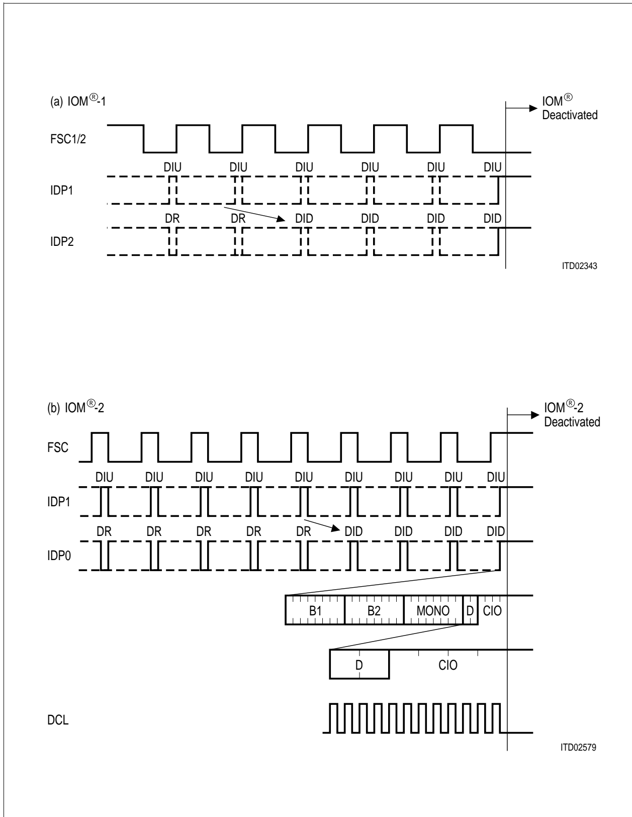
Figure 72 Deactivation of the IOM ® Interface
