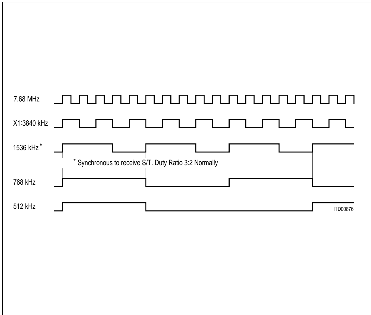
Figure 101 Phase Relationships of ISAC ® -S Clock Signals
