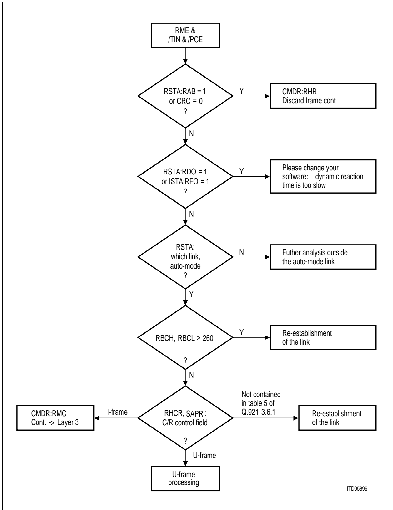
Figure 61 Interrupt Service Routine after RME
