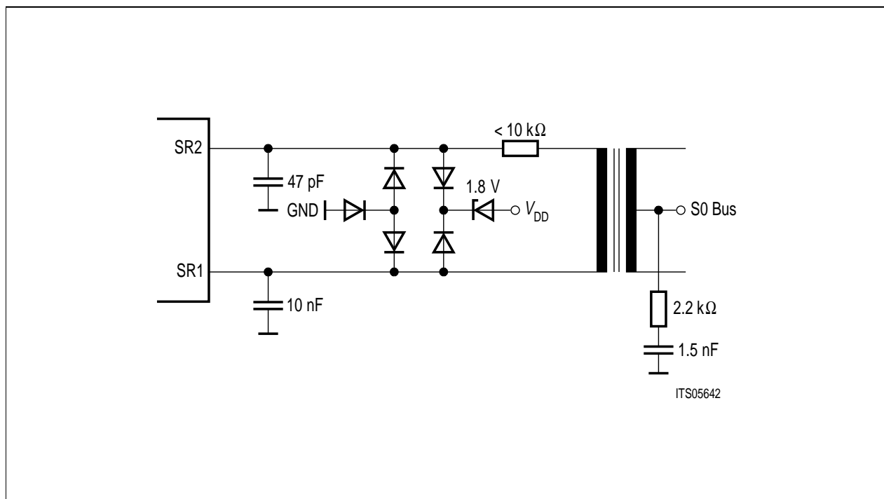
Figure 48 External Circuitry for Unsymmetrical Receivers (PEB 2086)
