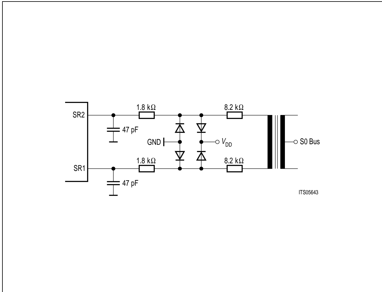
Figure 49 External Circuitry for Symmetrical Receivers
