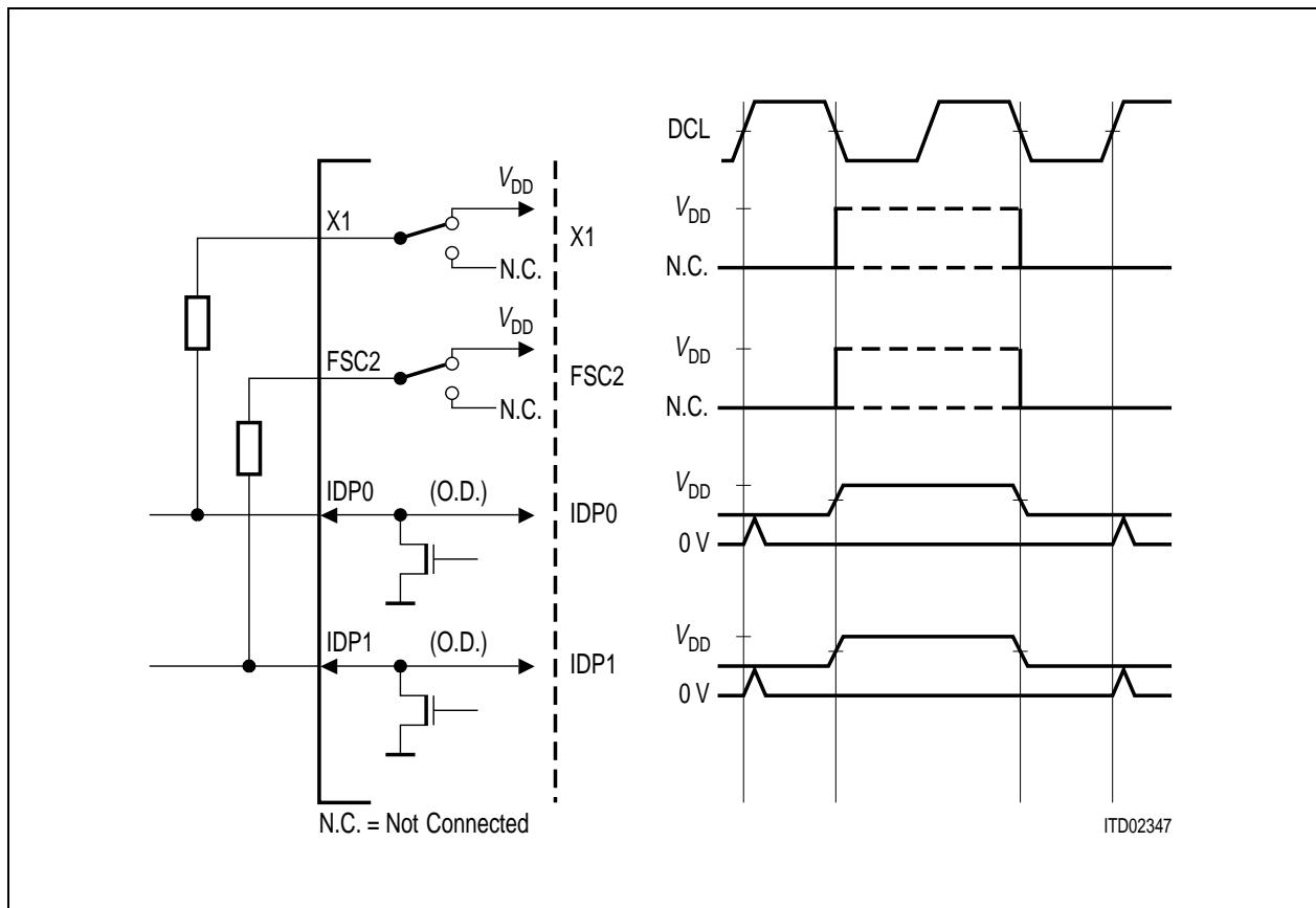
Figure 32 IOM ® -2 Connections for Power Saving Option
