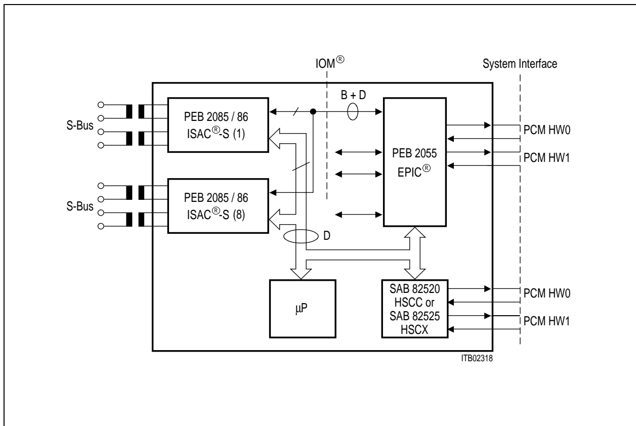
Figure 8 ISDN PABX Line Card Implementation
