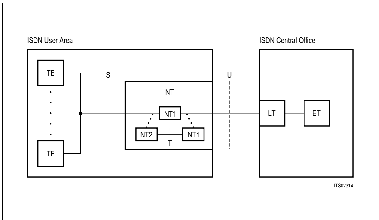
Figure 4 ISDN Basic Subscriber Access Architecture
