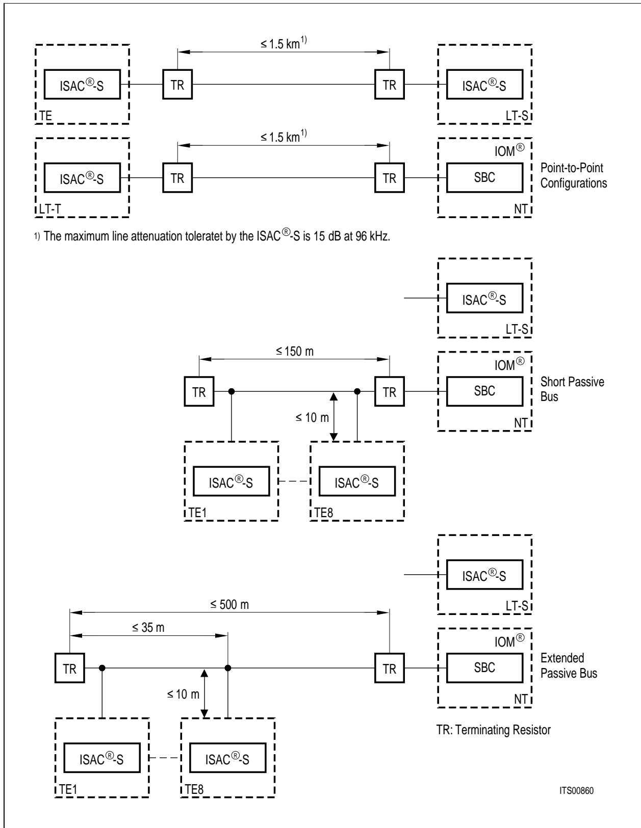
Figure 41 Wiring Configurations in User Premises
