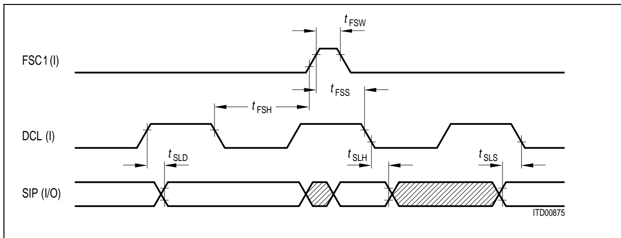
Figure 100 SLD Timing (LT-S / LT-T mode)
