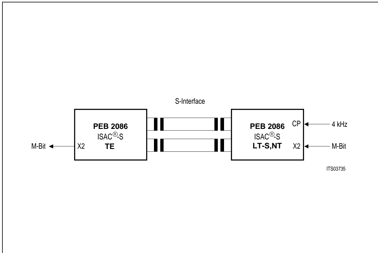
Figure 54 Multiframe Synchronization using the M-Bit
