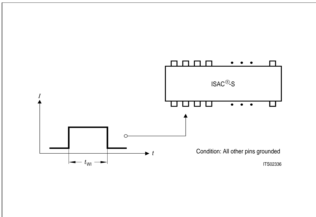
Figure 82 Test Condition for Maximum Input Current
