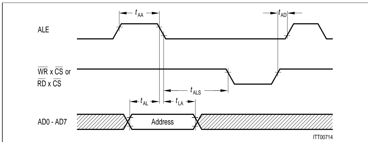
Figure 90 Multiplexed Address Timing
