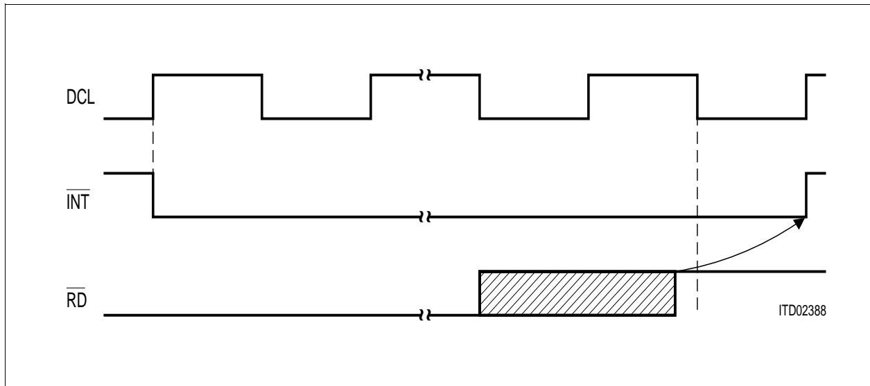
Figure 71 Timing of \overline{\text{INT}} Pin
