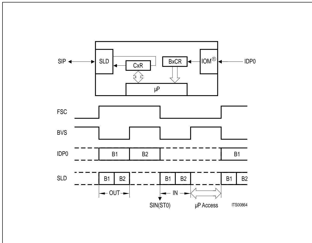
Figure 22 Bx Channel Access
