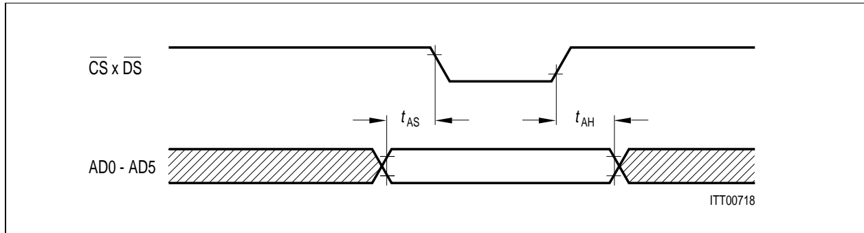
Figure 94 Non-Multiplexed Address Timing
