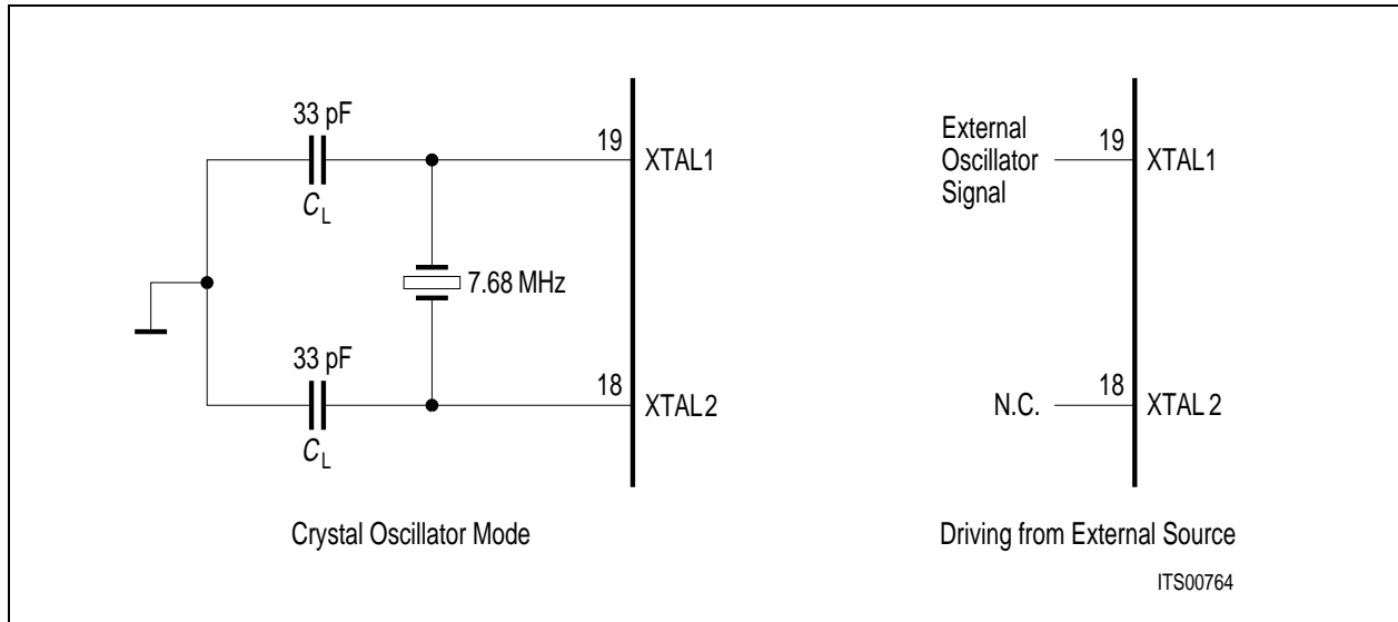
Figure 86 Oscillator Circuits Crystal Specification
