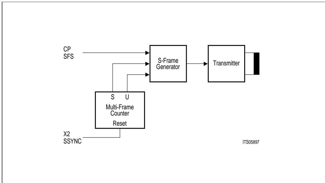
Figure 55 S-Frame Trigger and Multiframe Generation
