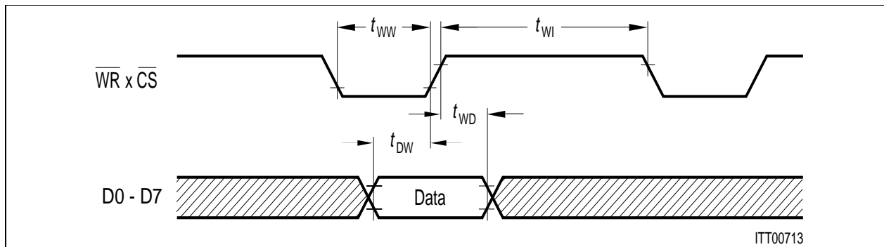
Figure 89 Microprocessor Write Cycle
