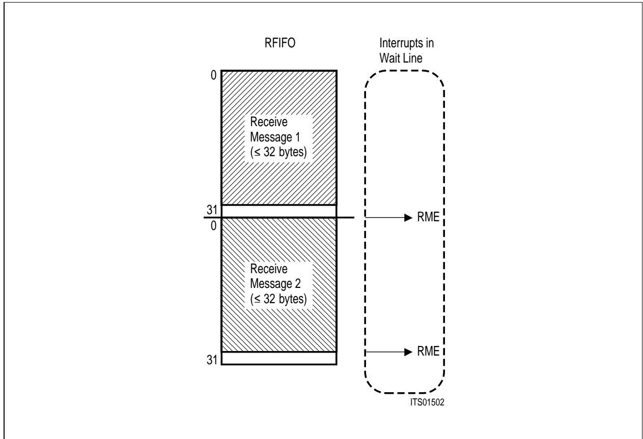
Figure 57 Contents of RFIFO (short message)
