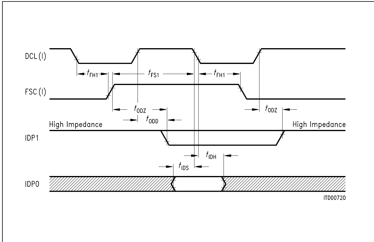
Figure 97 FSC1 (strobe) Characteristics
