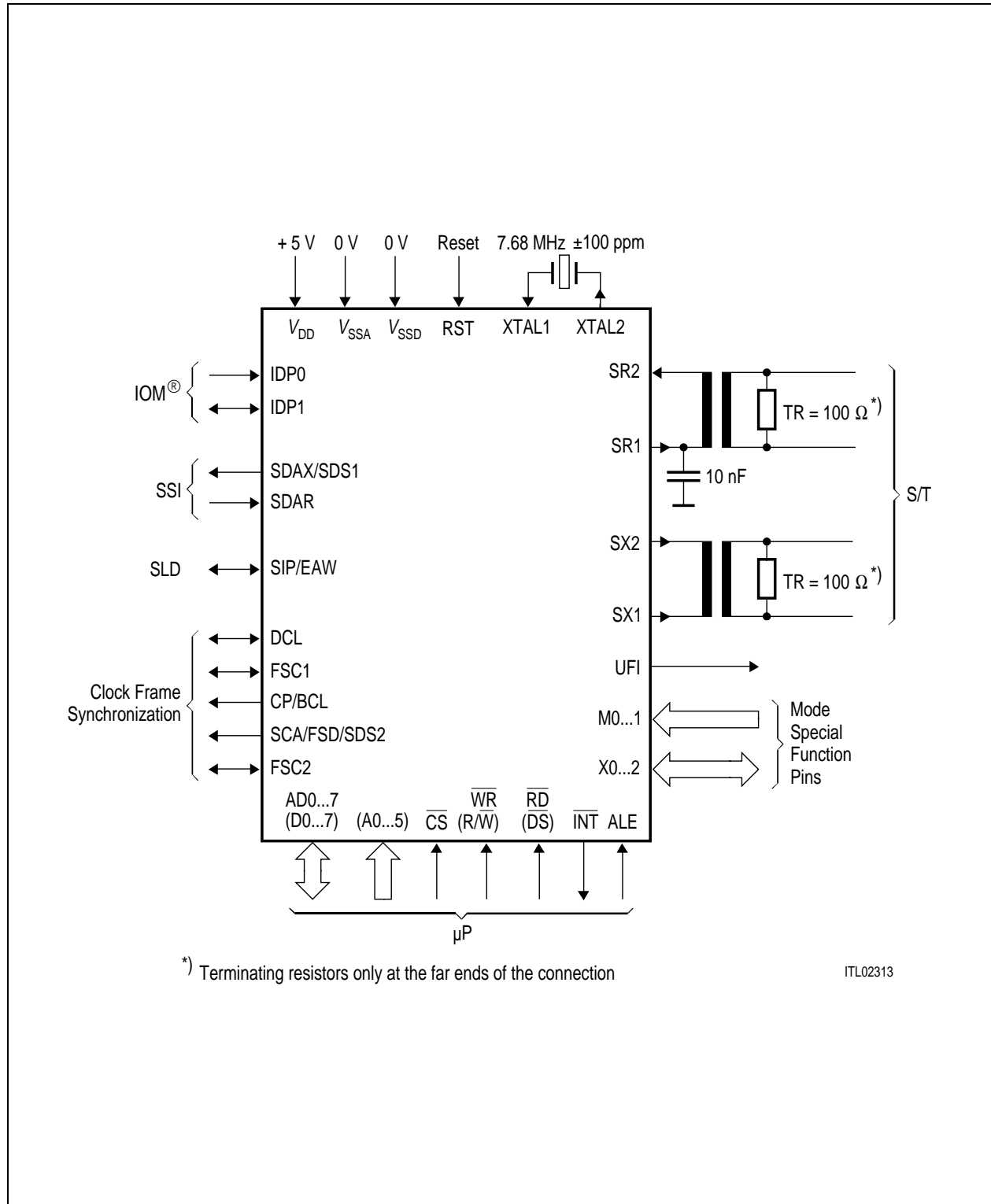
Figure 1 Logic Symbol of the ISAC ® -S
