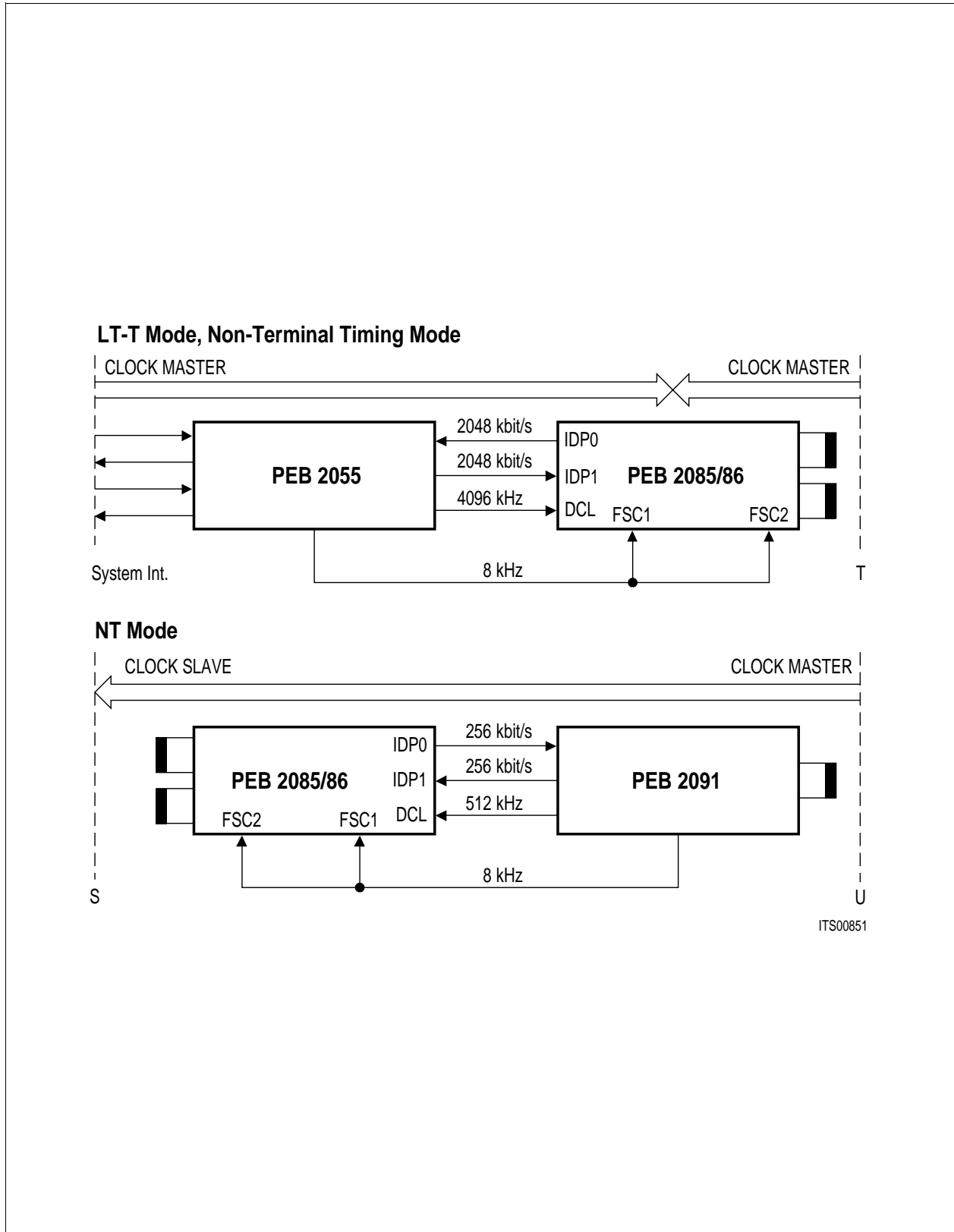
Figure 12b Operating Modes of ISAC ® -S (IOM ® -2)
