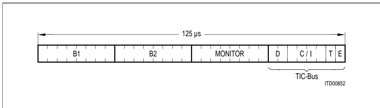
Figure 13 IOM ® -1 Frame Structure
