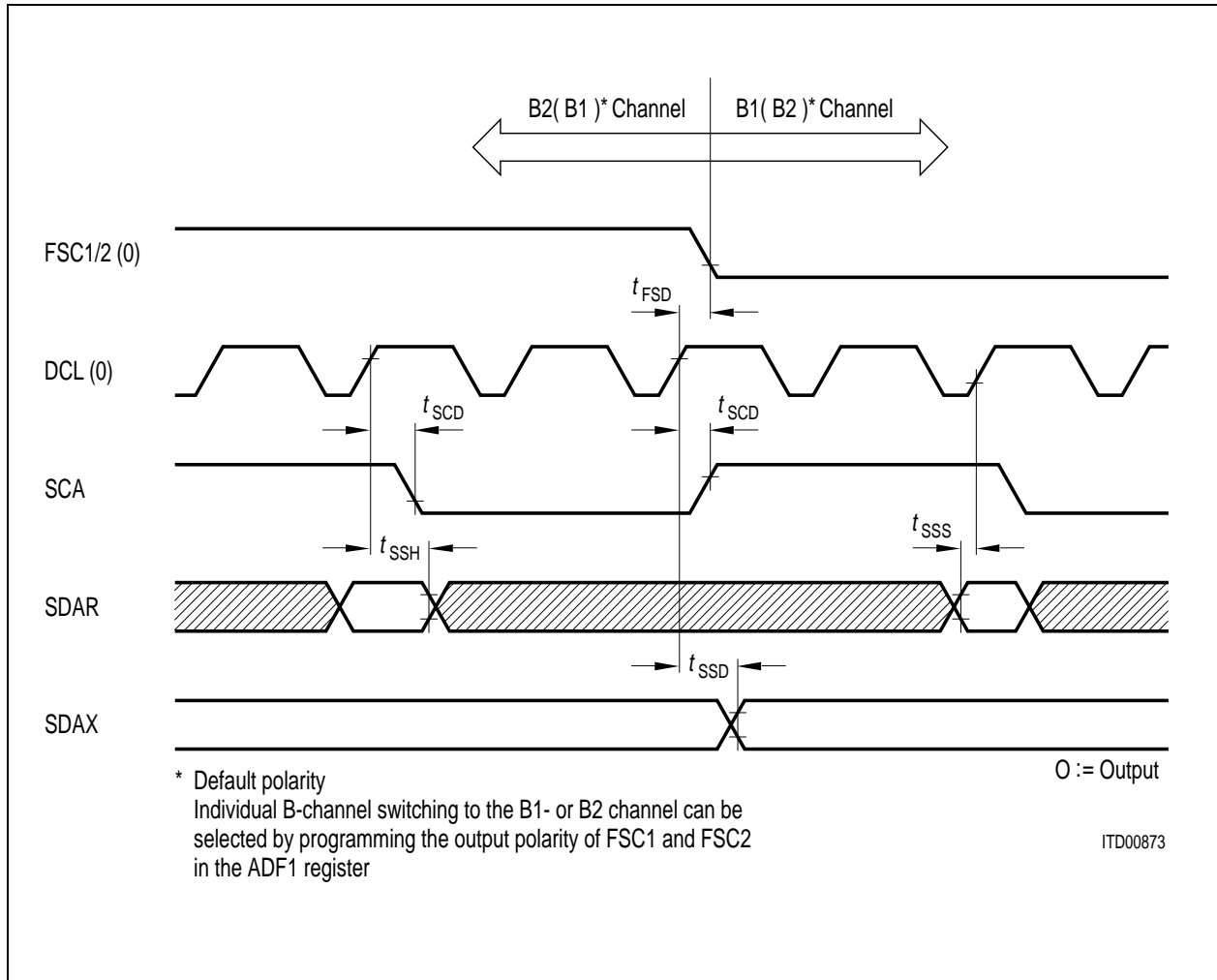
Figure 98 SSI Timing (TE, timing mode 0)
