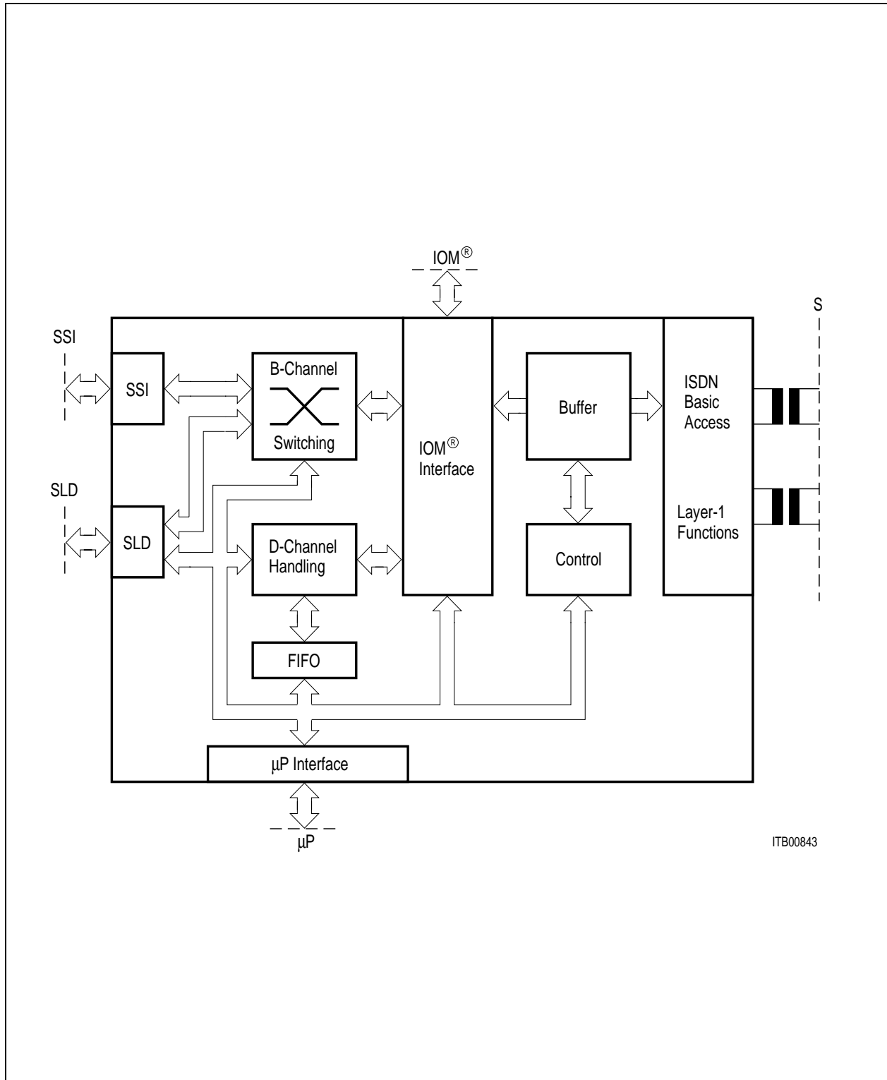
Figure 3 Block Diagram of the ISAC ® -S
