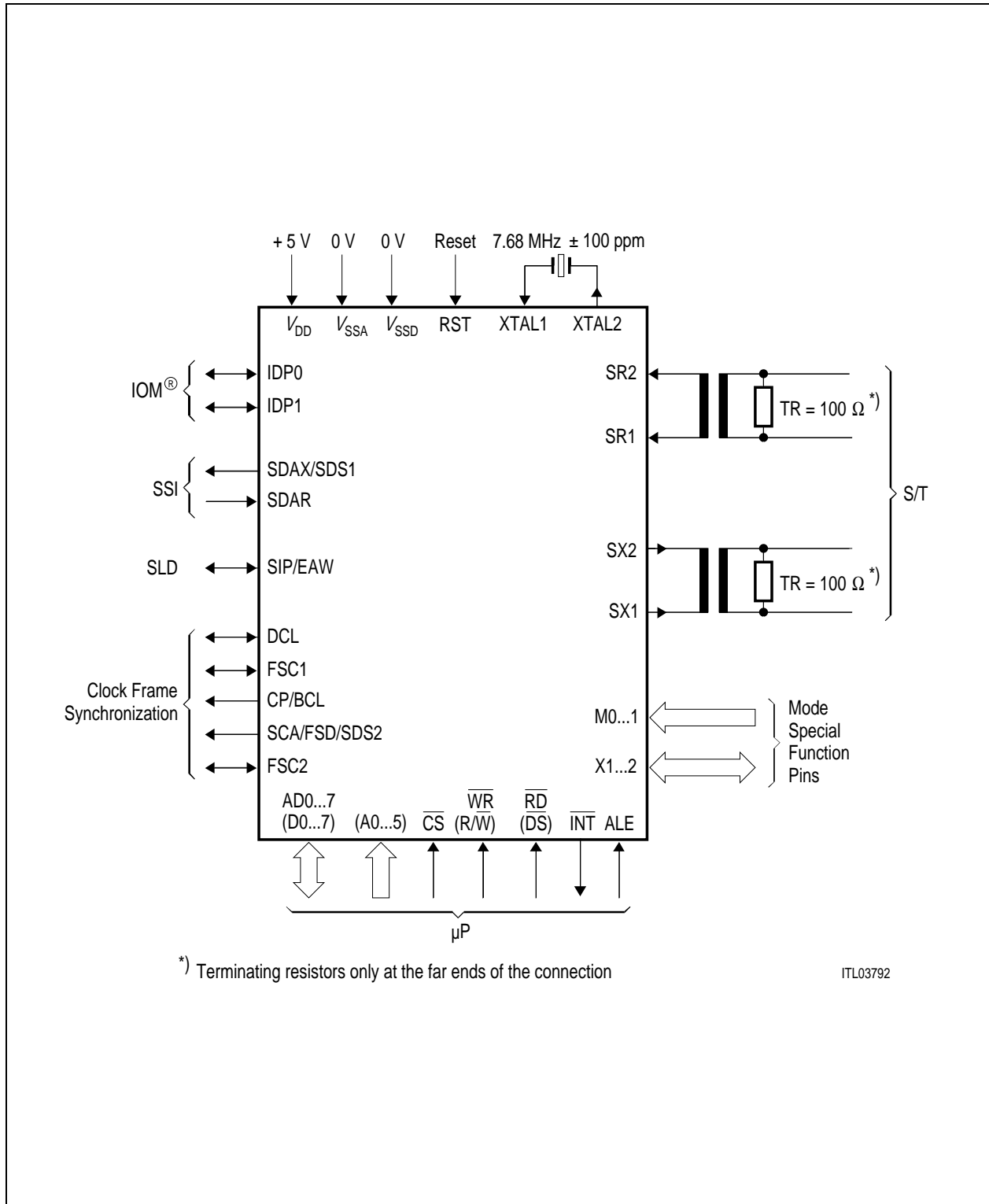
Figure 2 Logic Symbol of the ISAC ® -S
