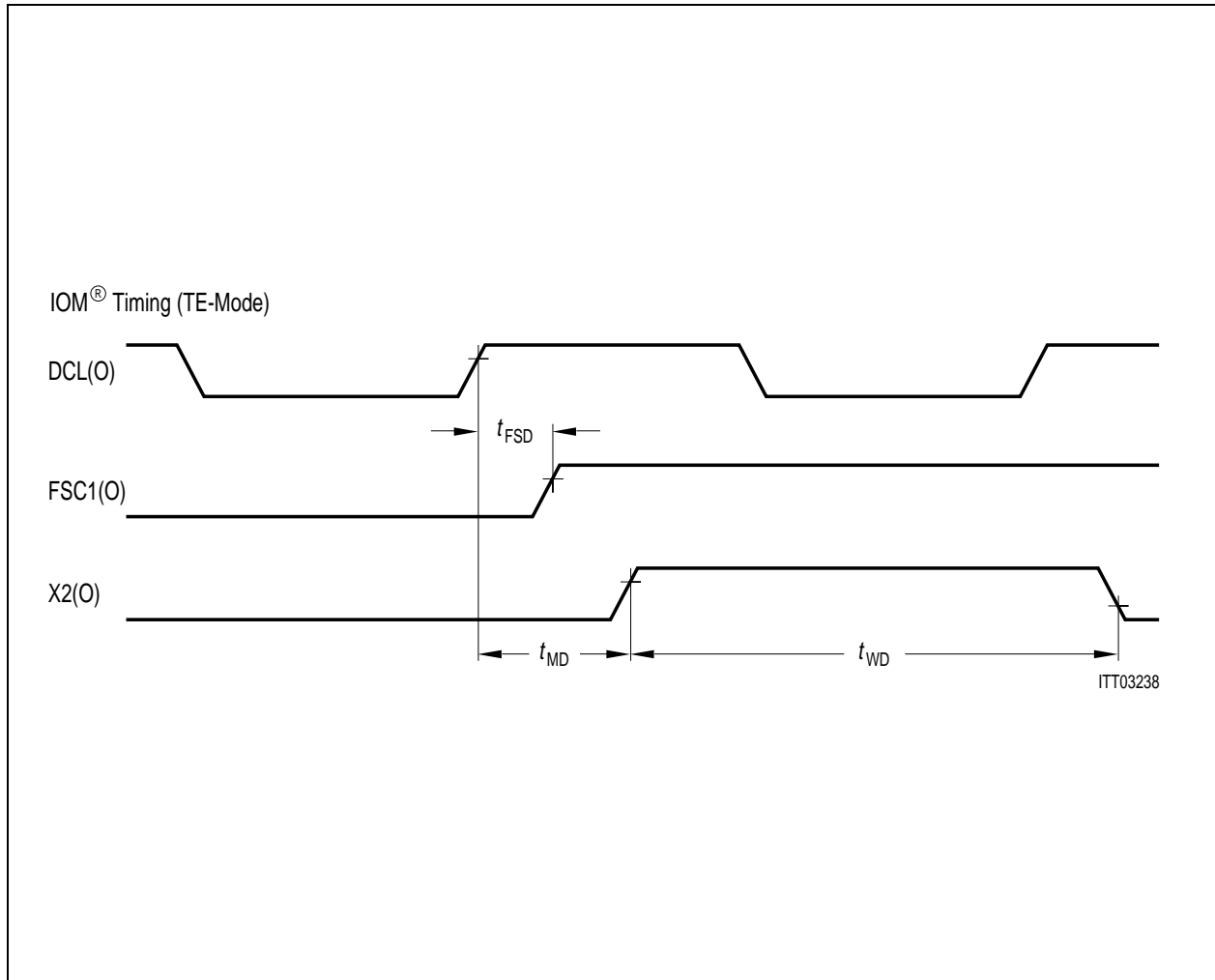
Figure 108 Multiframe Synchronization Output
