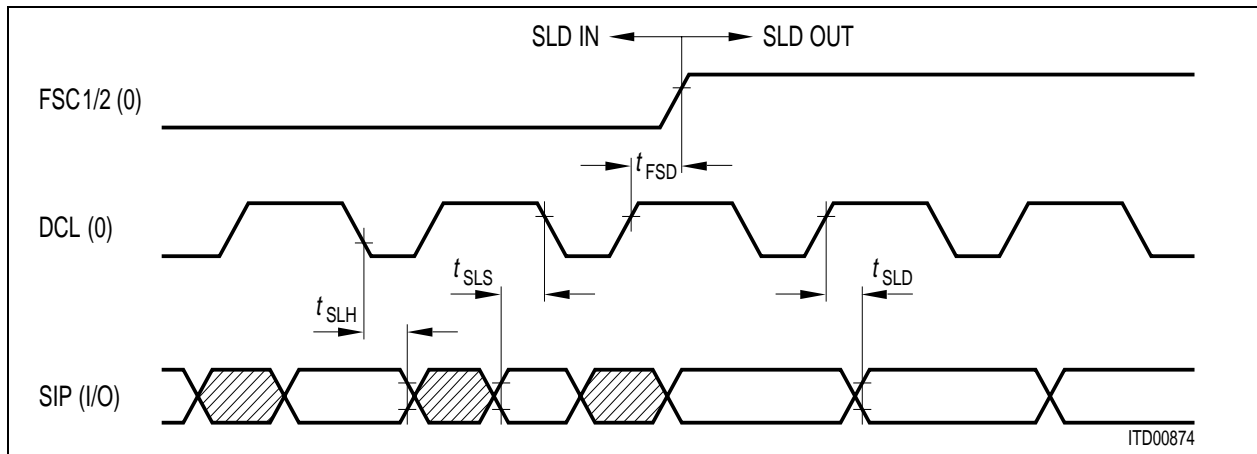
Figure 99 SLD Timing (TE mode)
