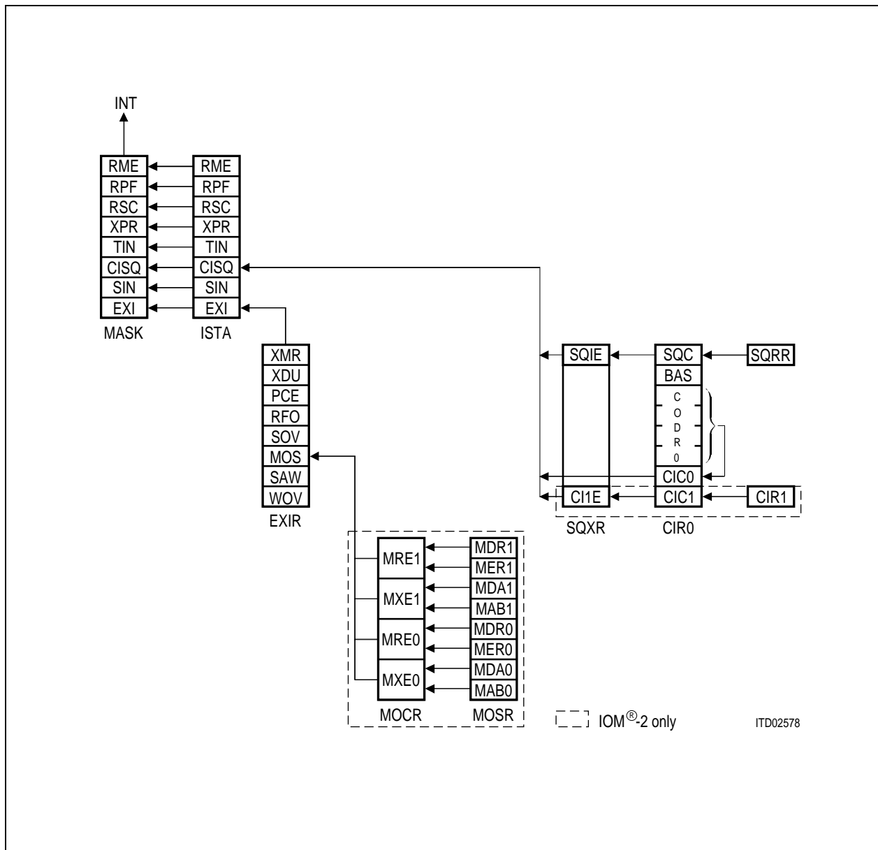
Figure 68 ISAC ® -S Interrupt Structure
