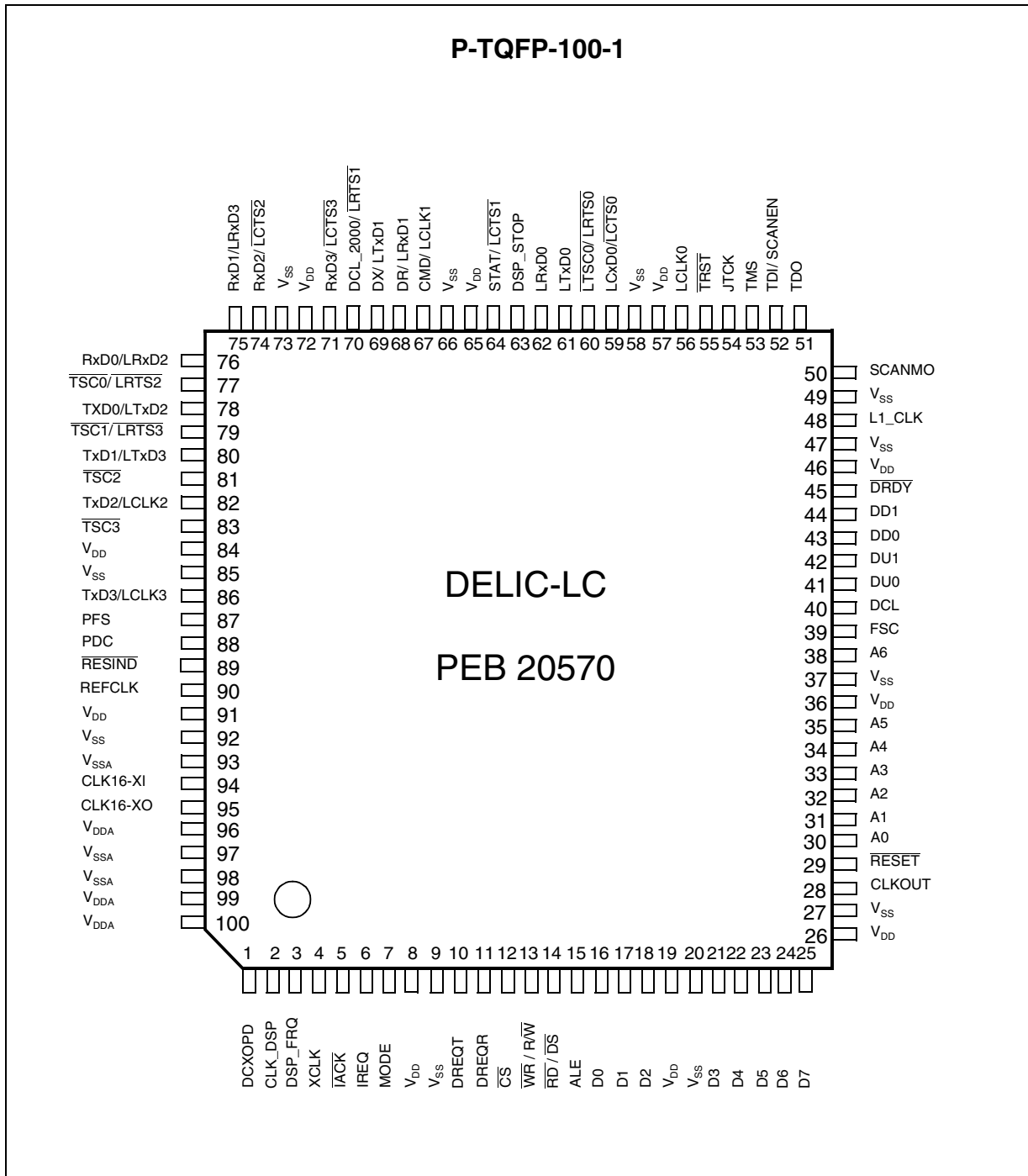
Figure 2-1 Pin Configuration DELIC-LC
