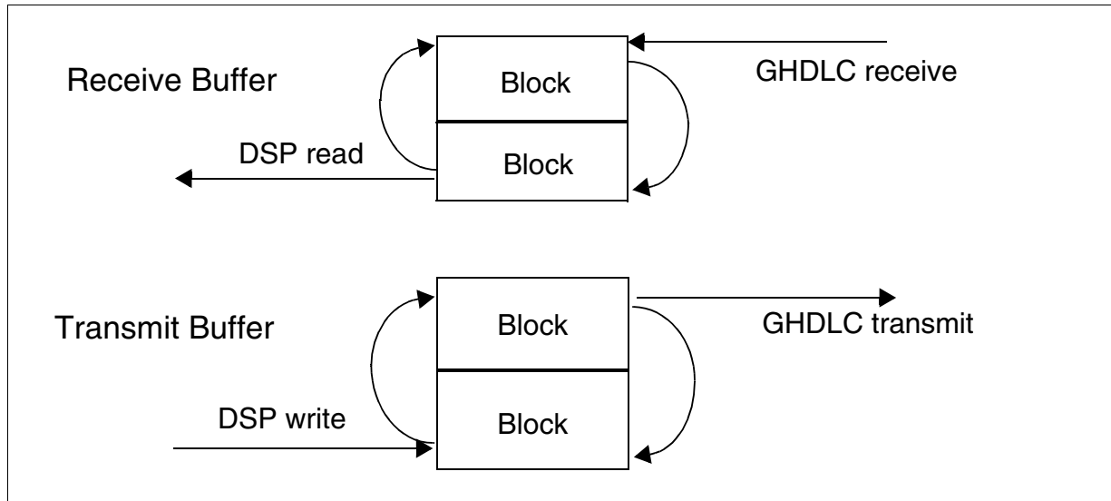
Figure 4-14 GHDLC Receive and Transmit Buffer Structure
