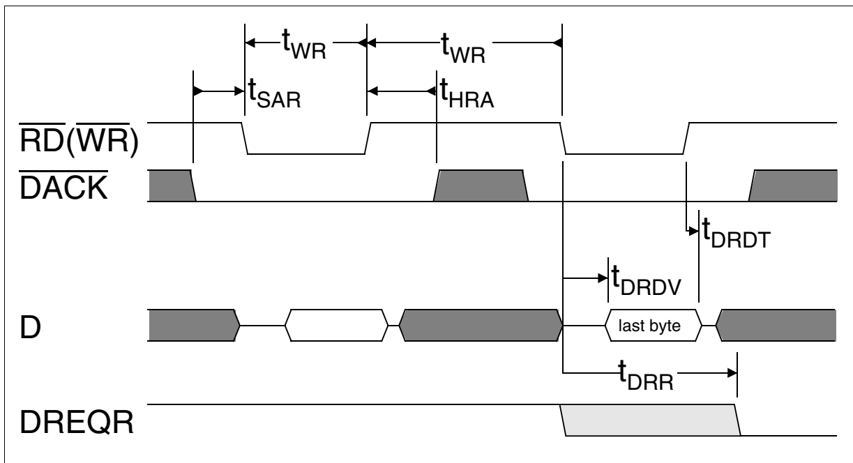
Figure 9-13 DMA Read Transaction Timing in Intel/Infineon Mode
