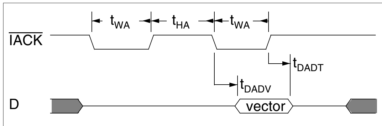
Figure 9-8 Interrupt Acknowledge Cycle Timing in Intel/Infineon Mode
