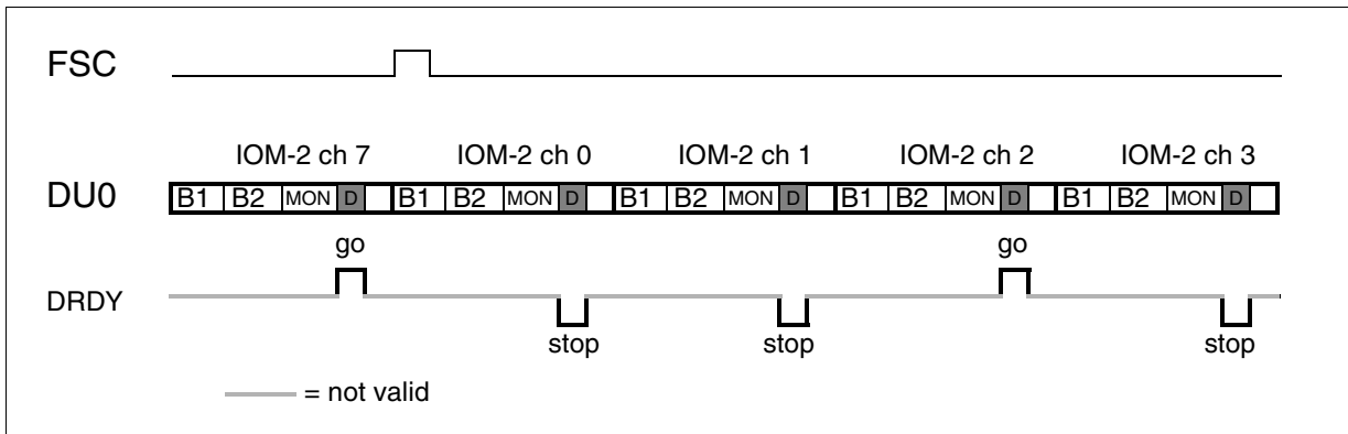
Figure 4-7 DRDY Signal Behavior
