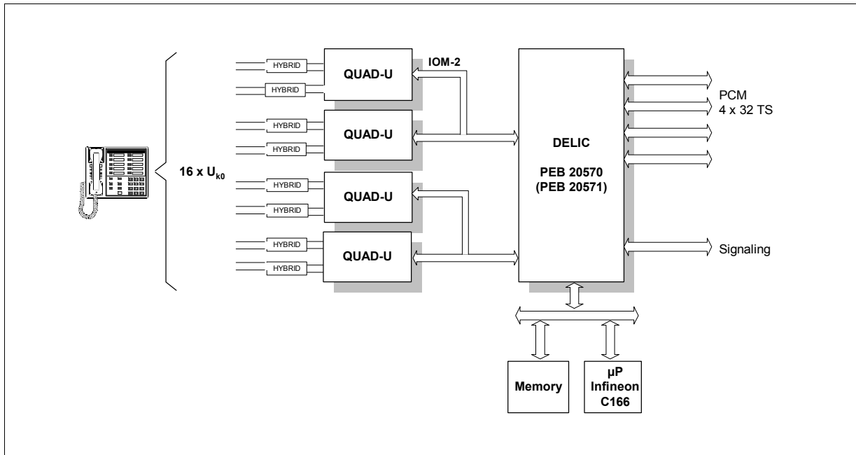
Figure 1-3 DELIC-LC in Uk0 Line Card for 16 Subscribers
