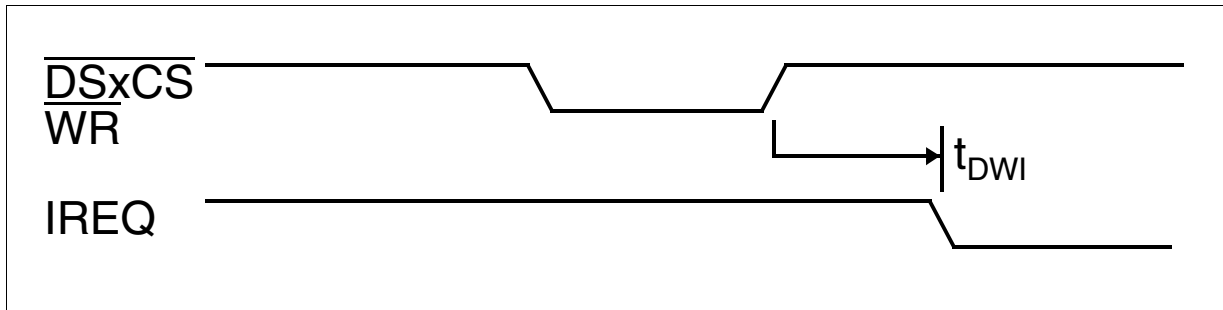
Figure 9-9 IREQ Deactivation Timing
