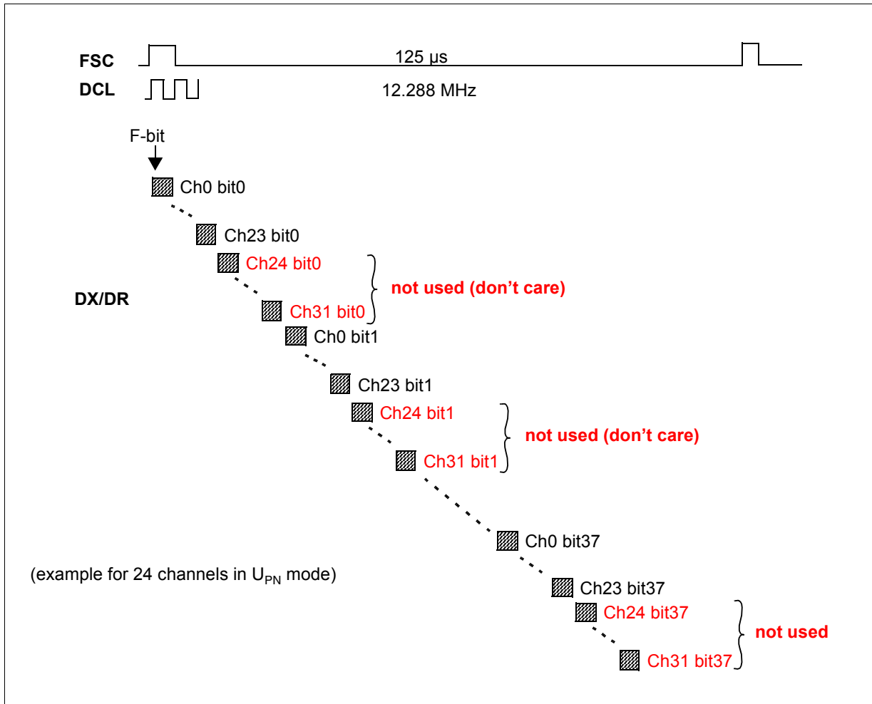
Figure 3-3 IOM-2000 Data Order (3 VIPs with 24 Channels)
