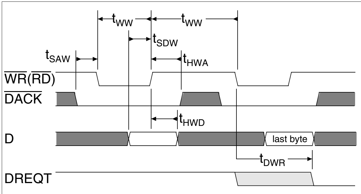
Figure 9-12 DMA Write Transaction Timing in Intel/Infineon Mode
