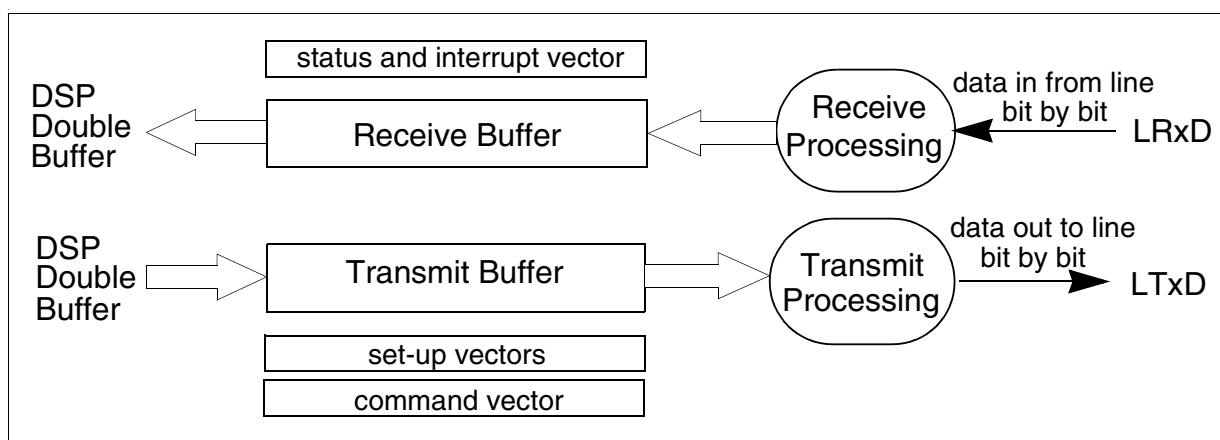
Figure 4-12 Data Processing in the GHDLC
