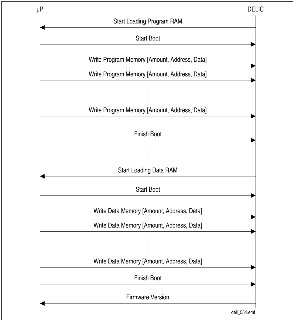
Figure 11-4 Boot Sequence
