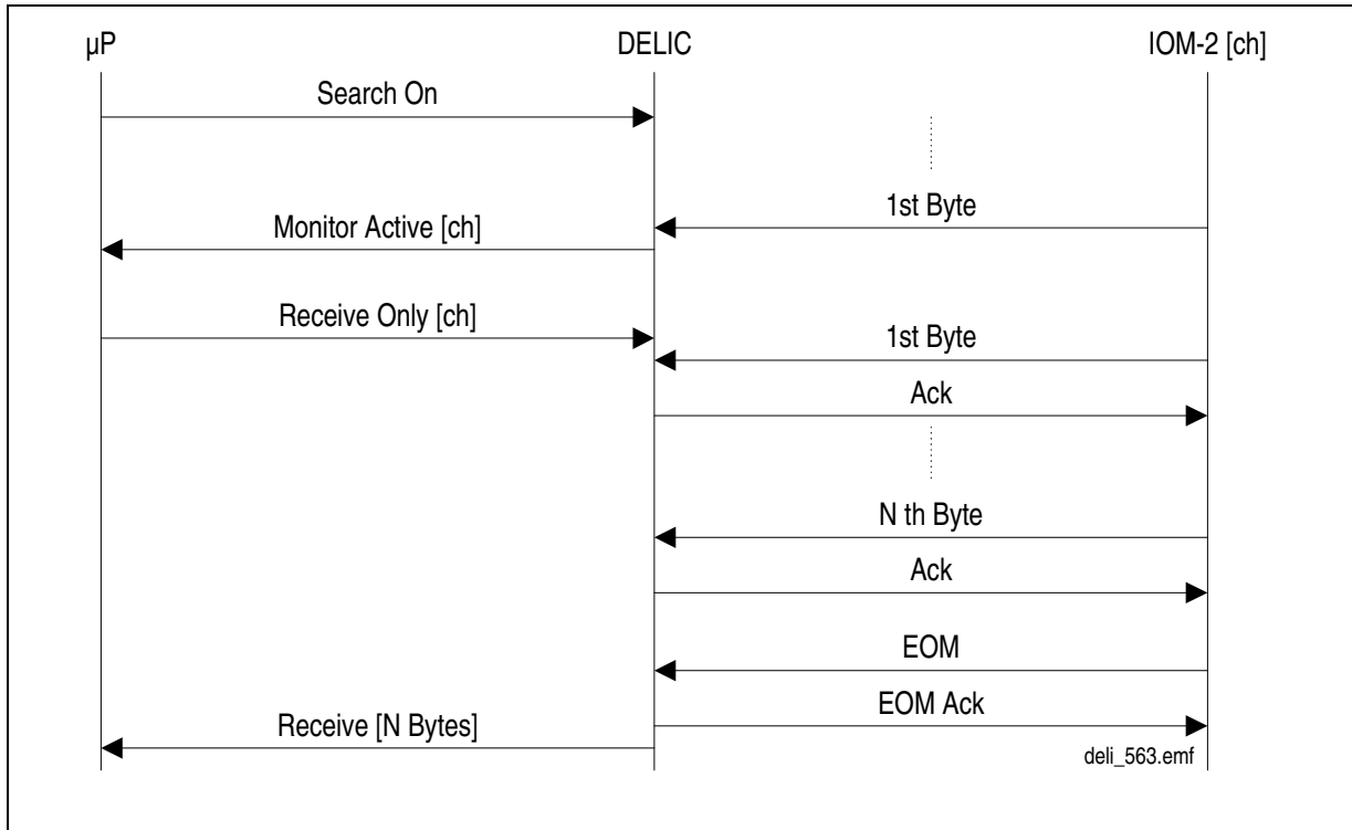
Figure 11-9 Monitor Flow Diagram: Search Mode
