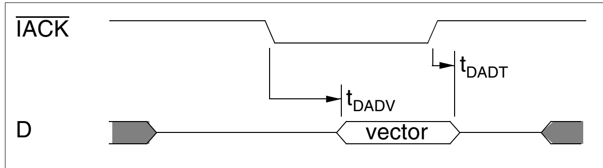
Figure 9-7 Interrupt Acknowledge Cycle Timing in Motorola Mode
