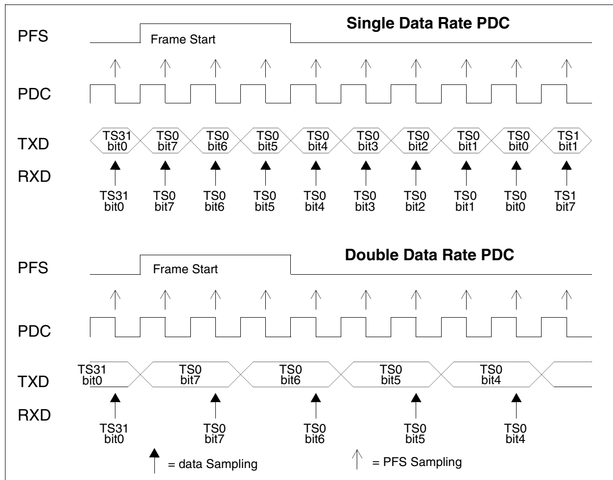
Figure 4-10 IOM-2 Interface Timing in Single/Double Clock Mode
