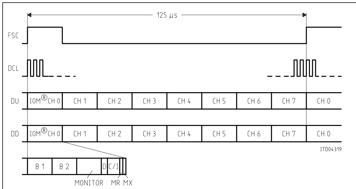
Figure 3-9 IOM ® -2 Interface in Digital Linecard Mode
