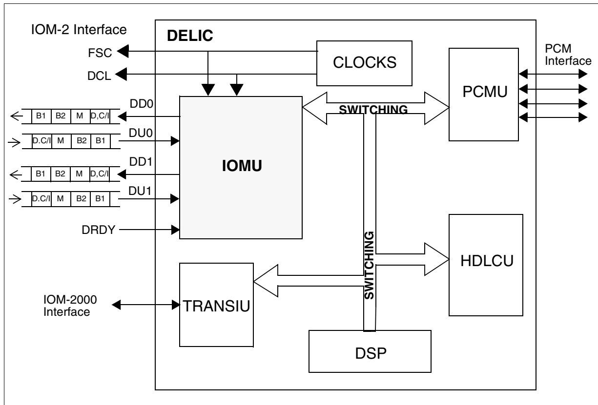
Figure 4-3 IOMU Integration in DELIC
