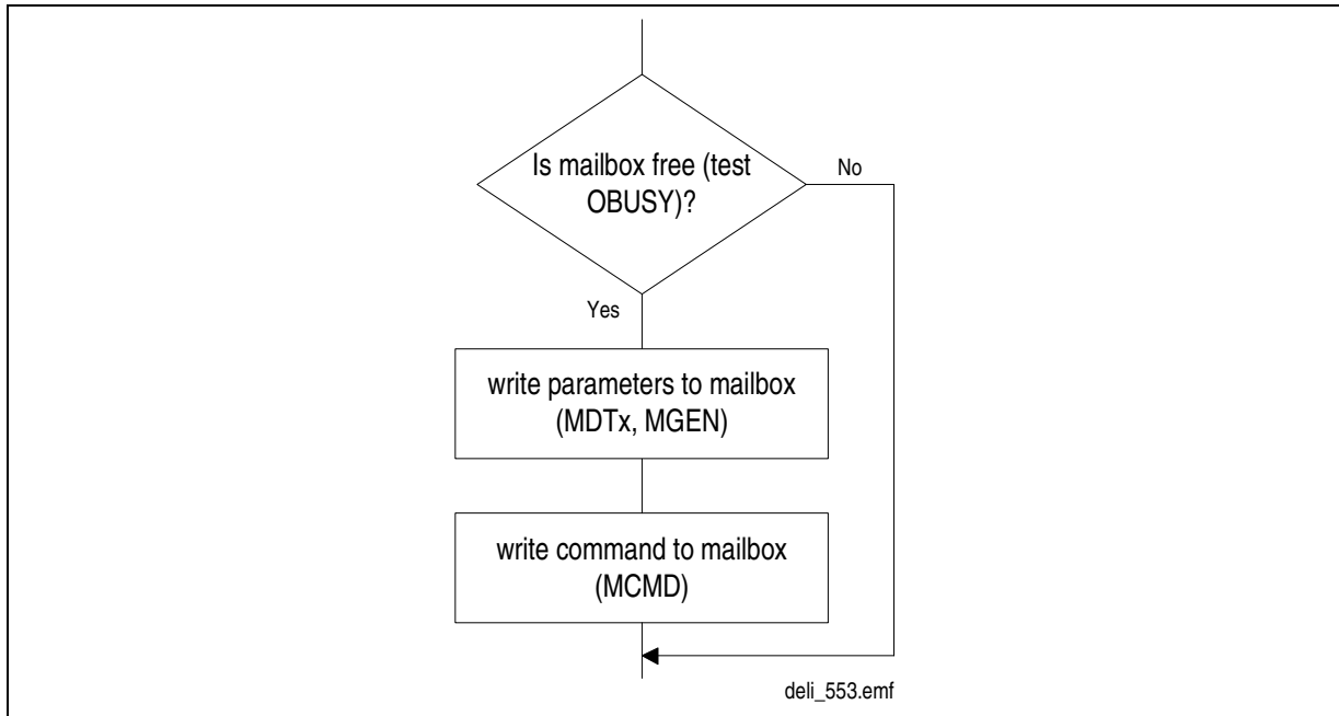
Figure 11-3 Flow Diagram: Mailbox Write Access
