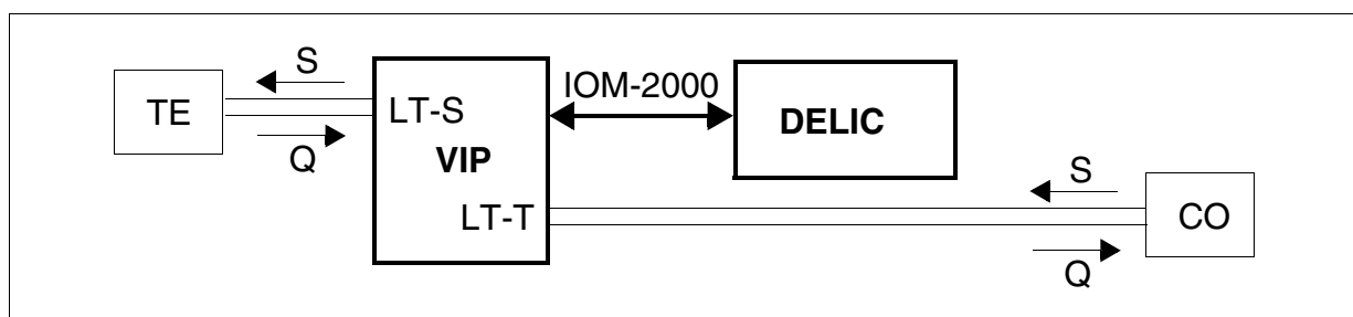
Figure 4-2 S/Q Channel Assignment
