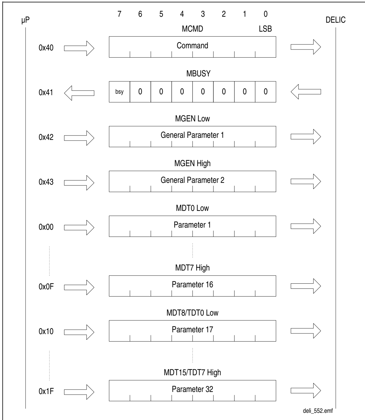
Figure 11-1 Transmit Mailbox Structure
