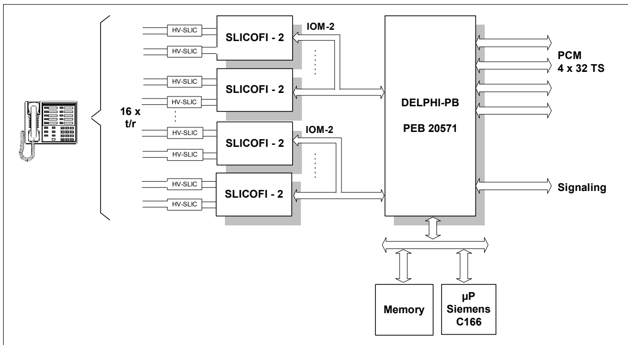
Figure 1-4 DELIC-PB in Analog Line Card for 16 Subscribers
