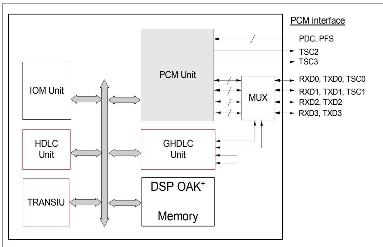
Figure 4-9 PCMU Integration in DELIC
