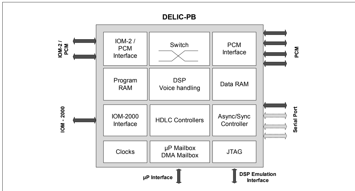
Figure 1-2 Block Diagram of the DELIC-PB
