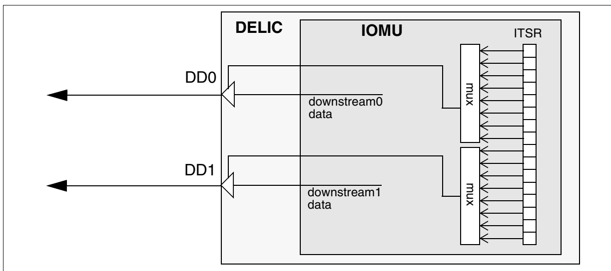
Figure 4-6 IOM-2 Interface Push-Pull Mode
