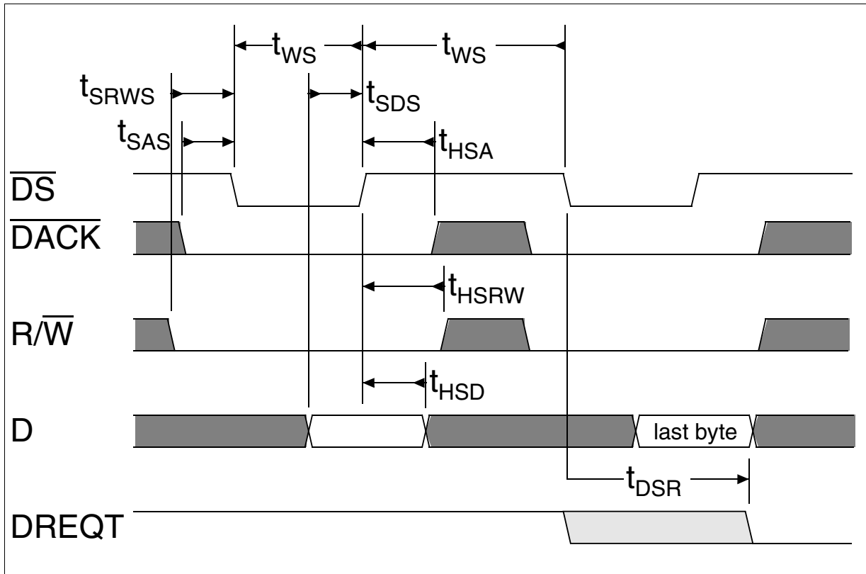
Figure 9-10 DMA Write Transaction Timing in Motorola Mode
