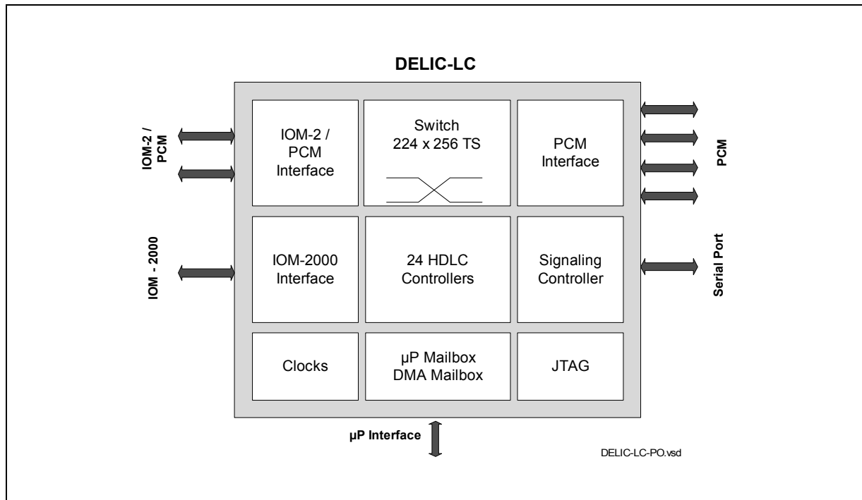
Figure 1-1 Block Diagram of the DELIC-LC
