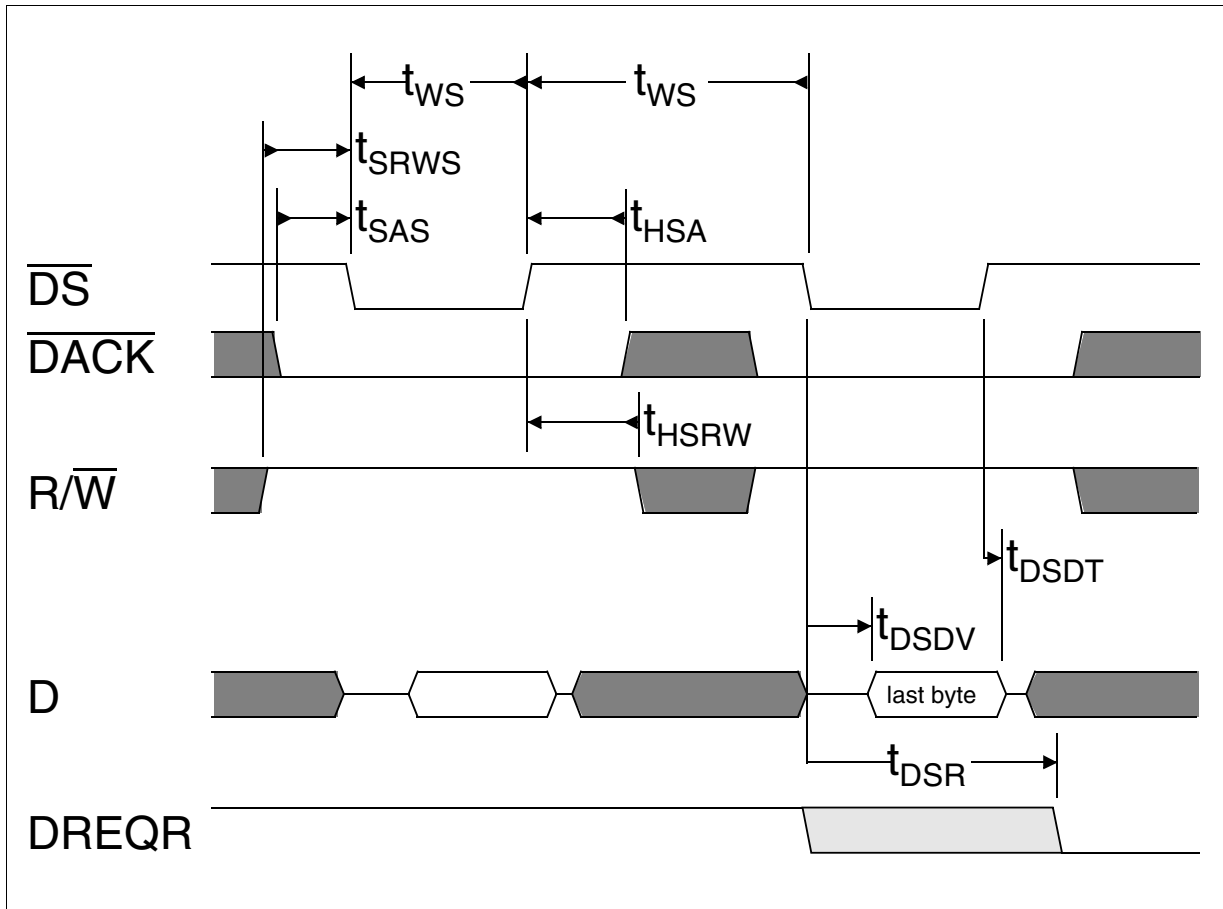
Figure 9-11 DMA Read-Transaction Timing in Motorola Mode
