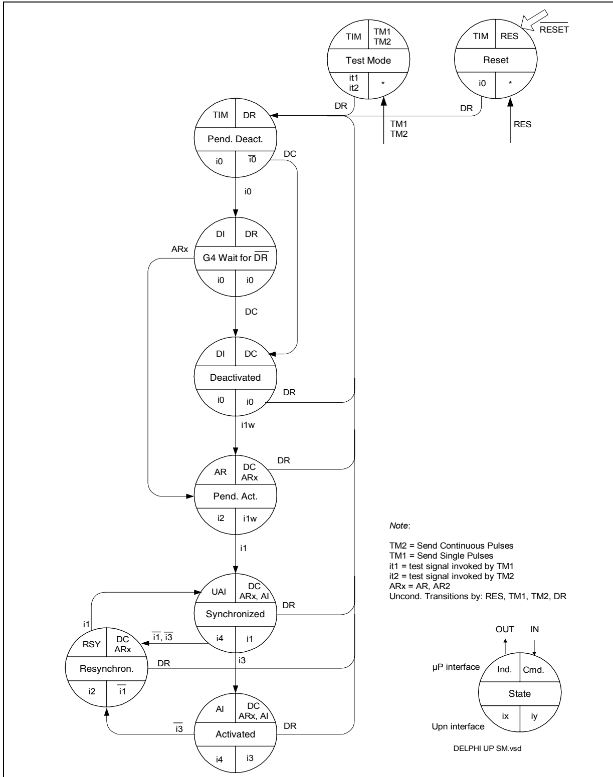
Figure 3-6 U PN State Diagram
