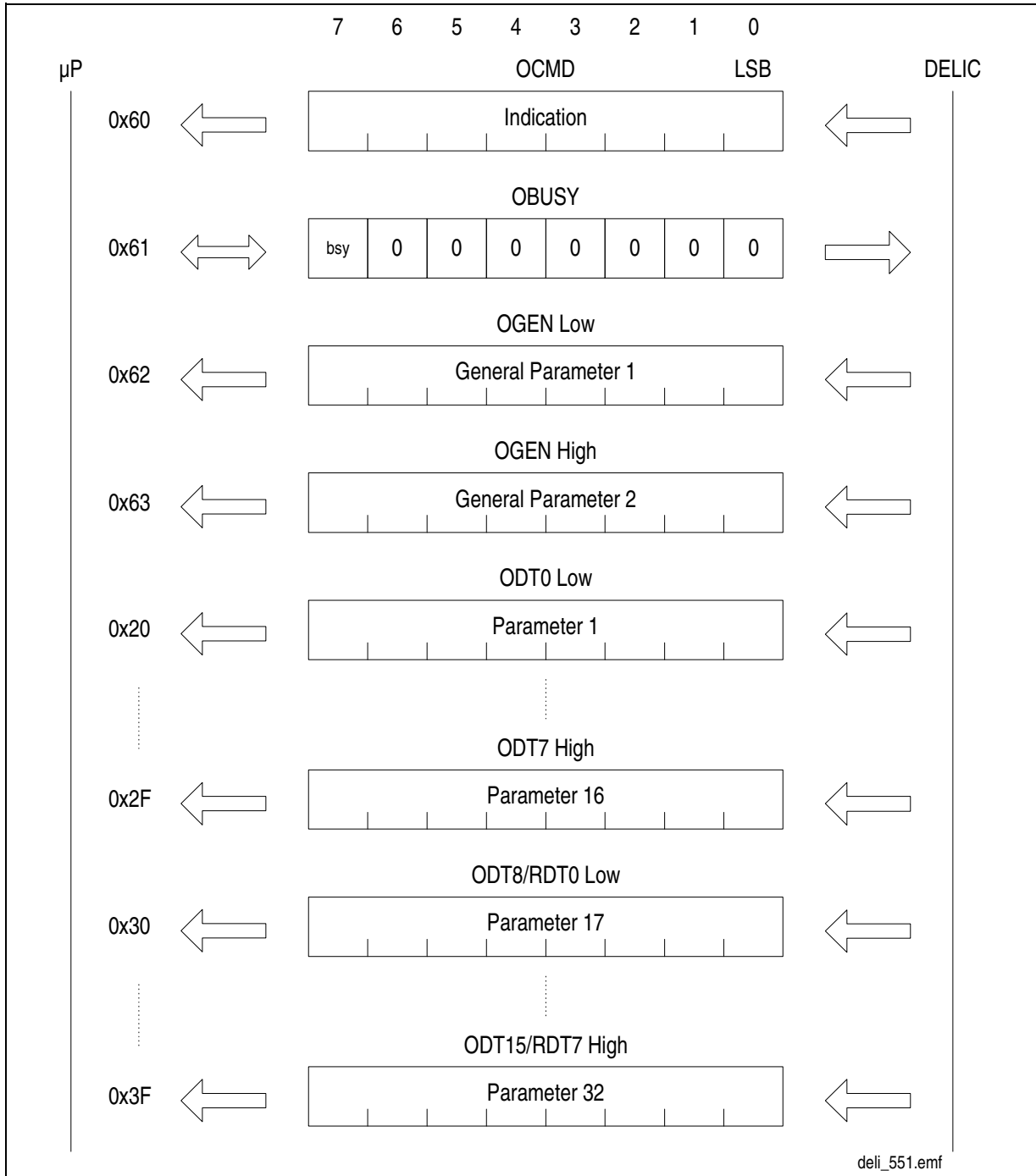
Figure 11-2 Receive Mailbox Structure
