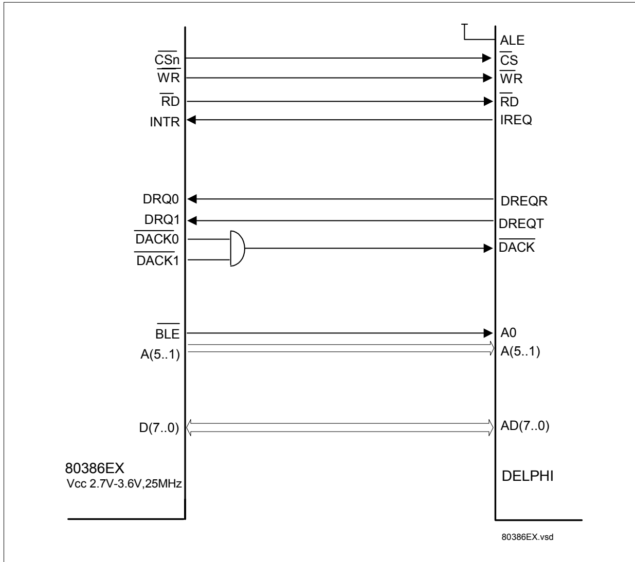
Figure 10-1 DELIC Connection to Intel 80386EX (Demuxed Configuration)
