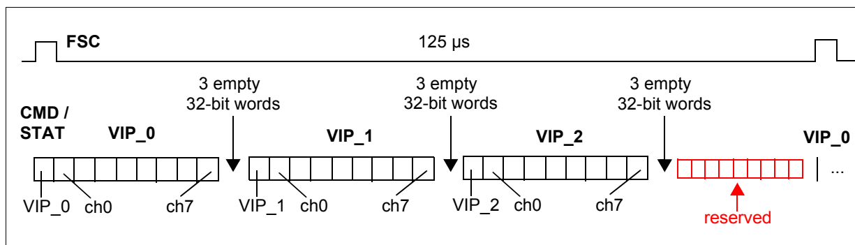
Figure 3-5 IOM-2000 Command/Status Sequence (3 VIPs with 24 Channels)
