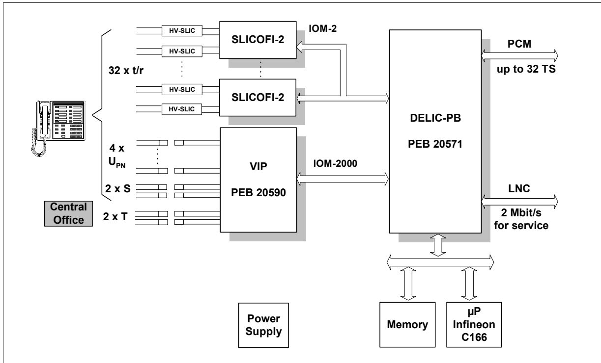
Figure 1-5 DELIC-PB in Small PBX
