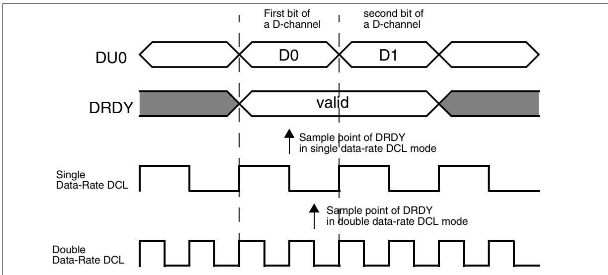
Figure 4-8 DRDY Sampling Timing
