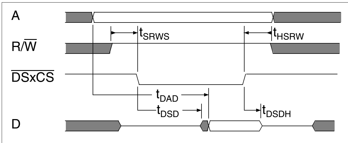
Figure 9-2 Read Cycle in Motorola Mode
