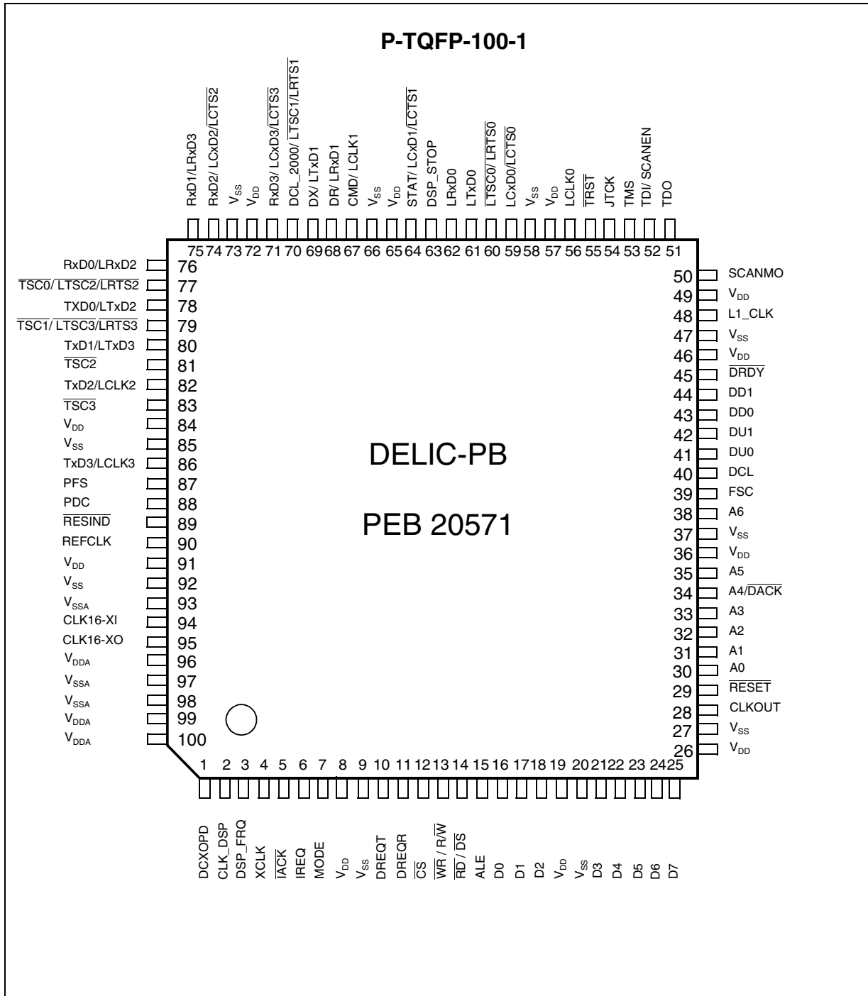
Figure 2-2 Pin Configuration DELIC-PB
