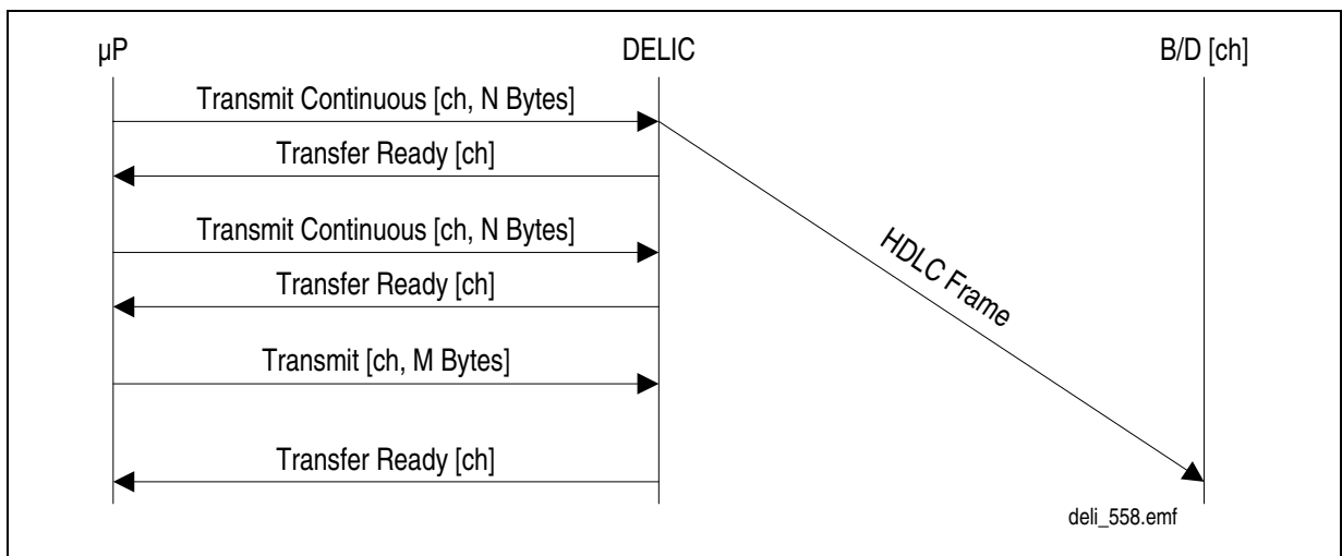
Figure 11-14 HDLC Flow Diagram: Transmit Continuous
