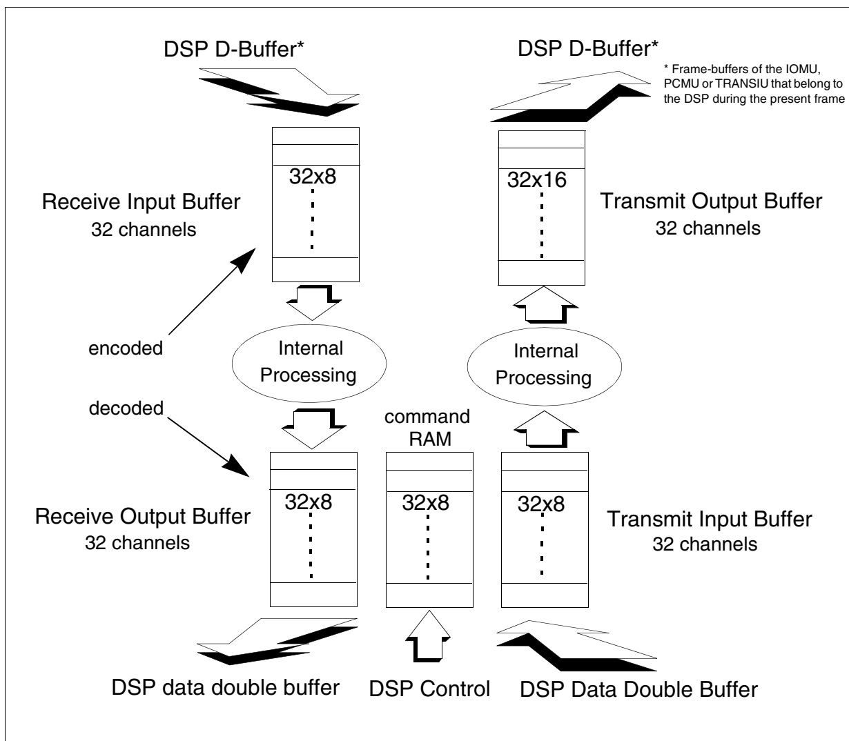
Figure 4-11 HDLCU General Block Diagram
