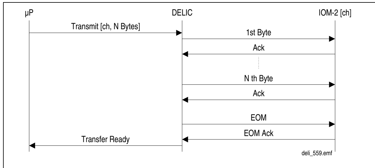
Figure 11-7 Monitor Flow Diagram: Transmit
