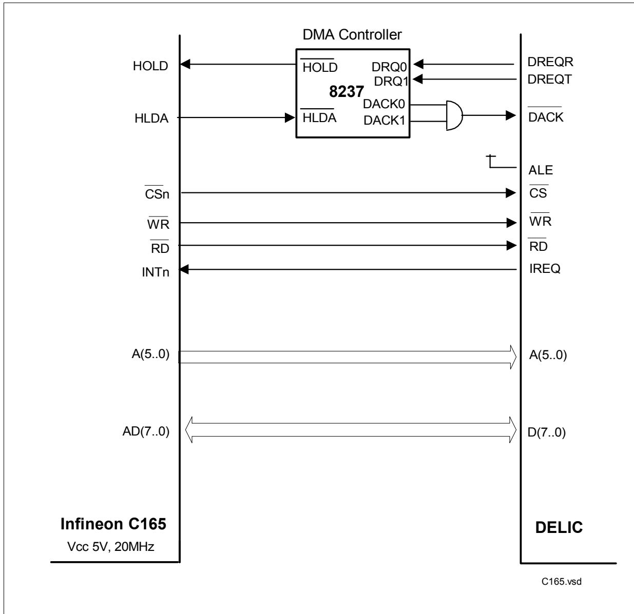
Figure 10-2 DELIC Connection to Siemens C165 (Demuxed Configuration)
