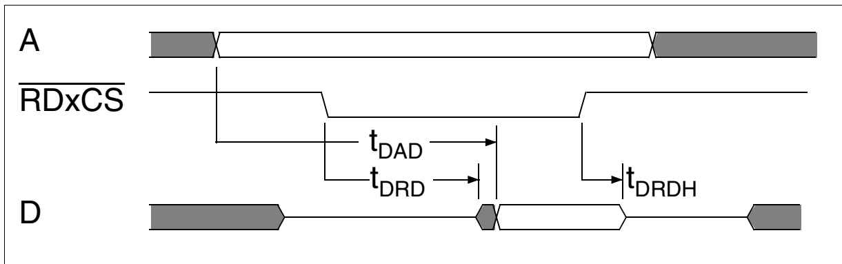
Figure 9-4 Read Cycle in Intel/Infineon De-multiplexed Mode
