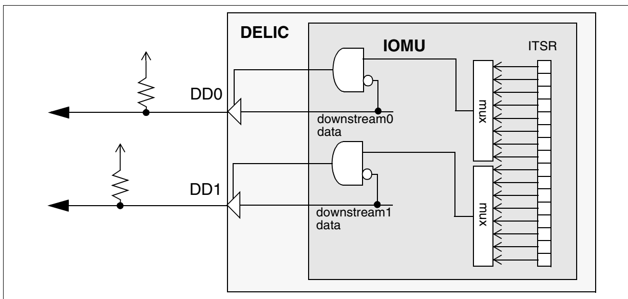
Figure 4-5 IOM-2 Interface Open-Drive Mode
