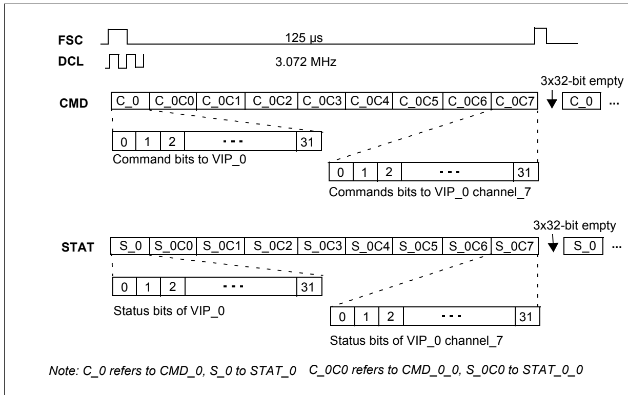
Figure 3-4 IOM-2000 CMD/STAT Handling (1 VIP with 8 Channels)
