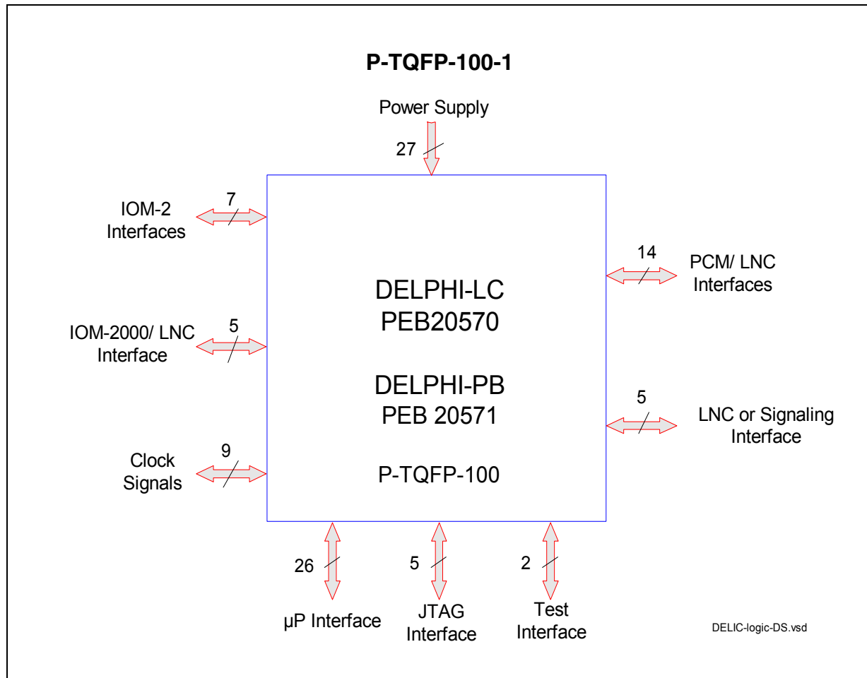
Figure 1-1 Logic Symbol
