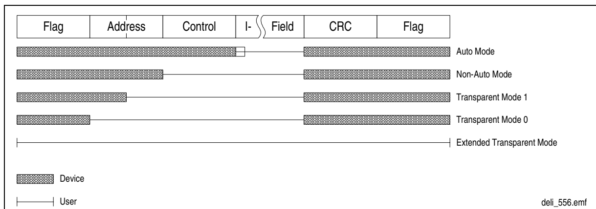
Figure 11-12 HDLC Frame Structure
