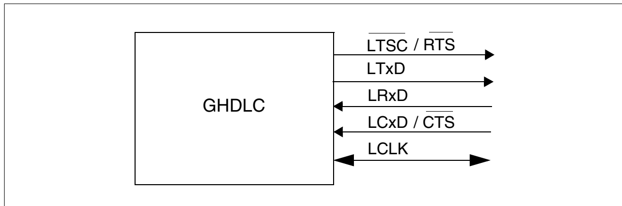
Figure 4-13 GHDLC Interface Lines
