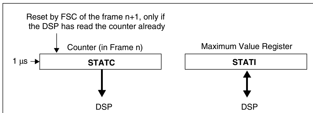
Figure 4-15 Statistics Registers
