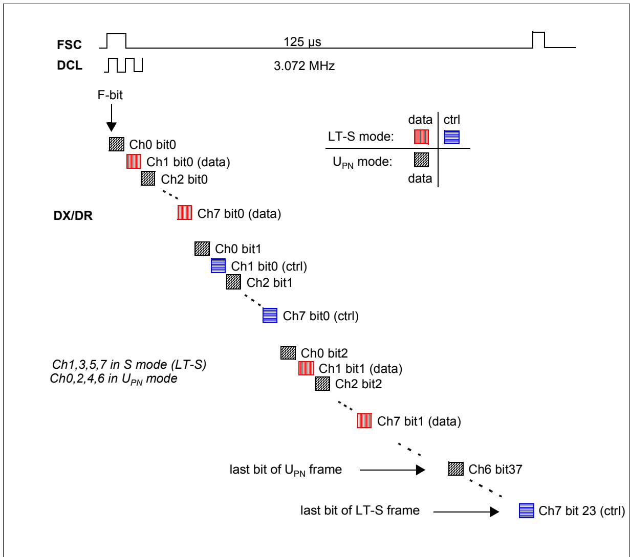
Figure 3-2 IOM-2000 Data Sequence (1 VIP with 8 Channels)
