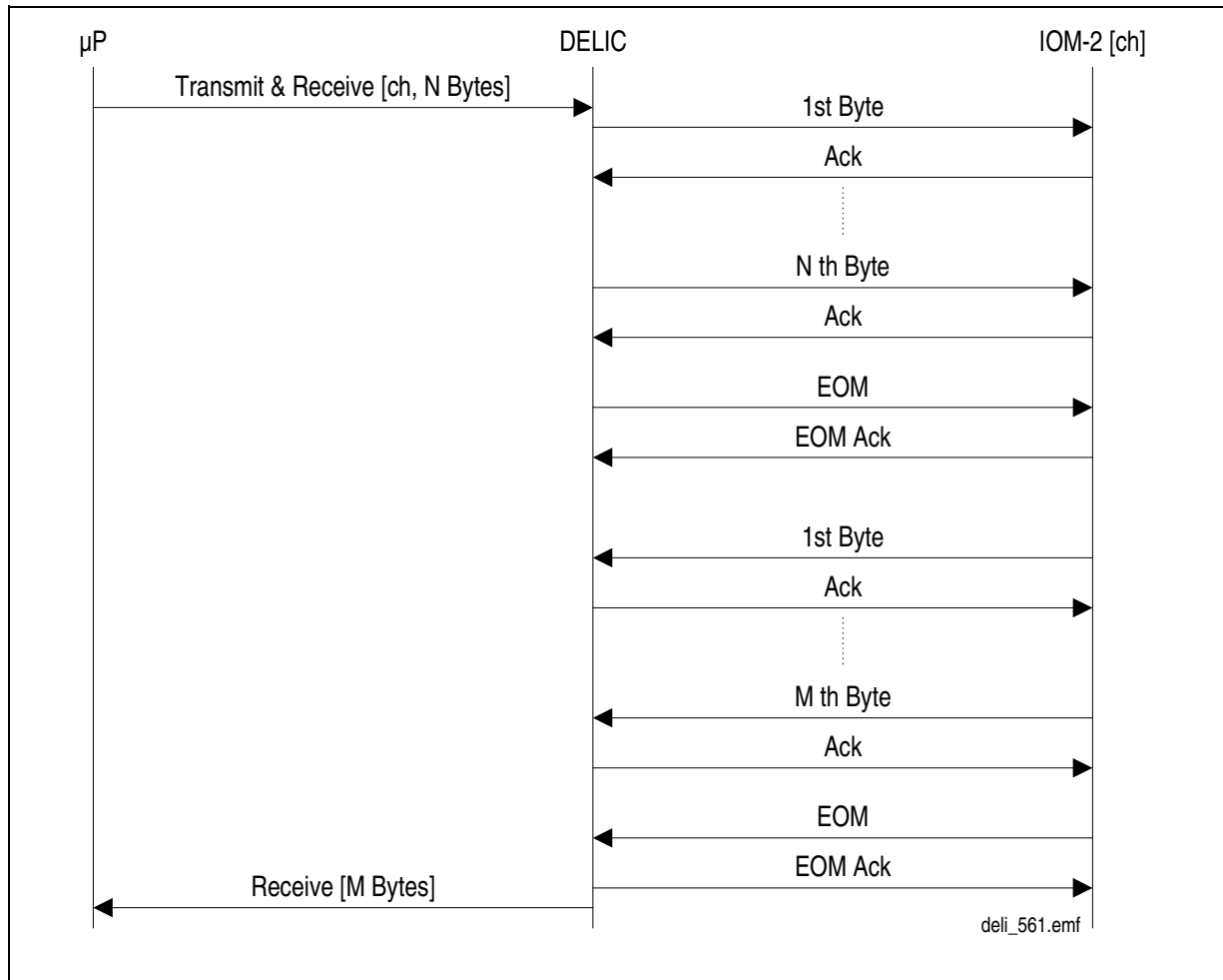
Figure 11-11 Monitor Flow Diagram: Transmit & Receive
