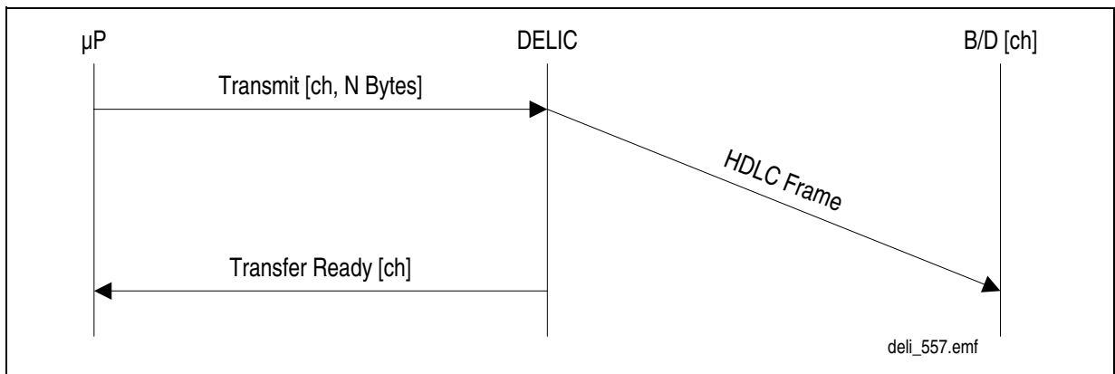
Figure 11-13 HDLC Flow Diagram: Transmit
