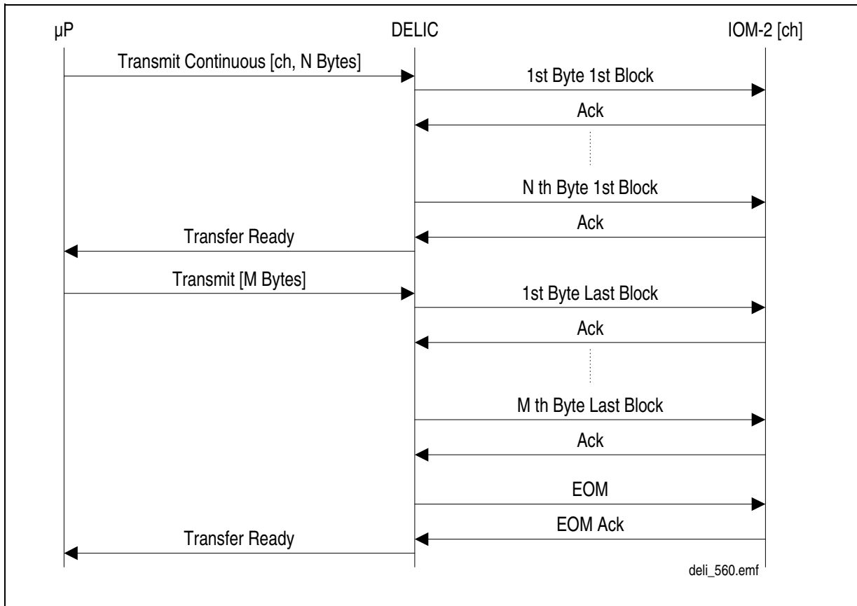
Figure 11-8 Monitor Flow Diagram: Transmit Continuous
