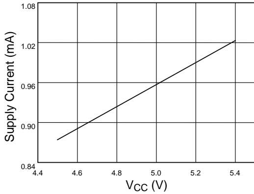
Fig. 2 Supply Current vs. Supply Voltage
