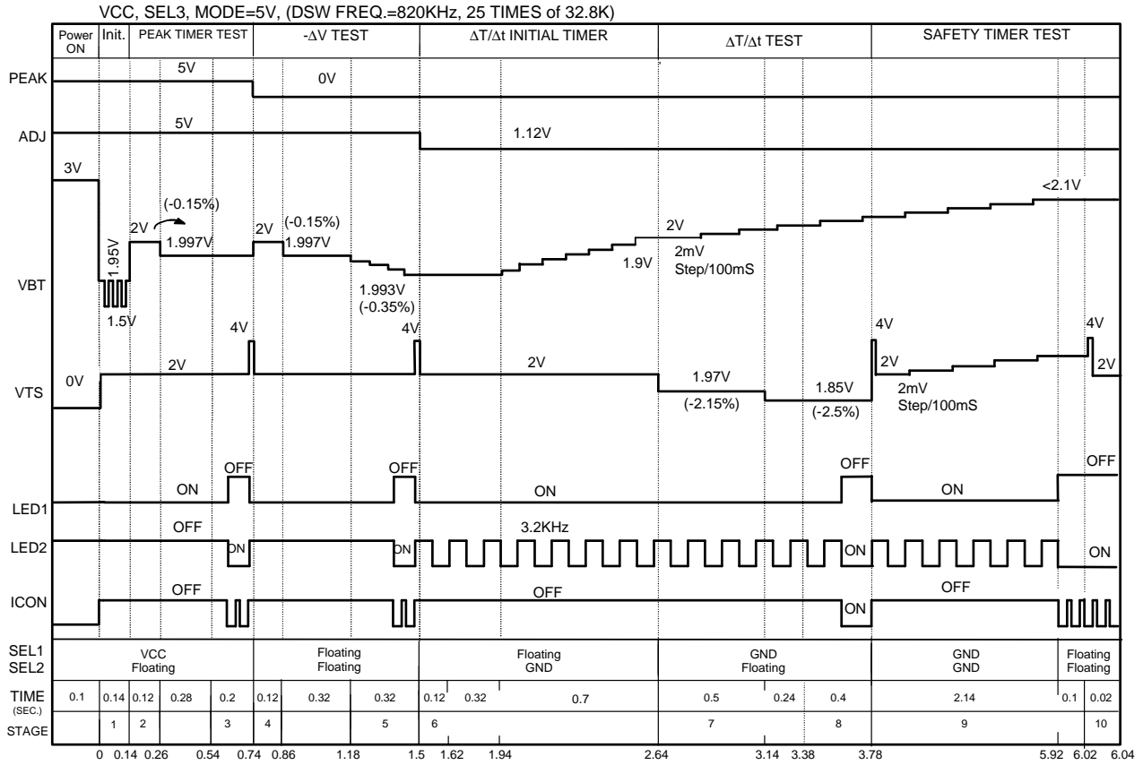
Fig. 20 Timing Diagram of AIC1781A in Test Mode
