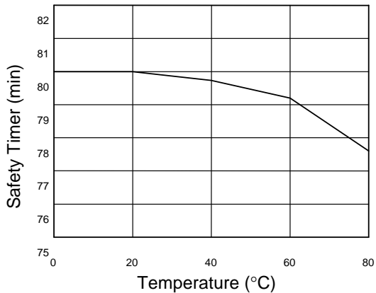
Fig. 6 Safety Timer vs. Temperature
