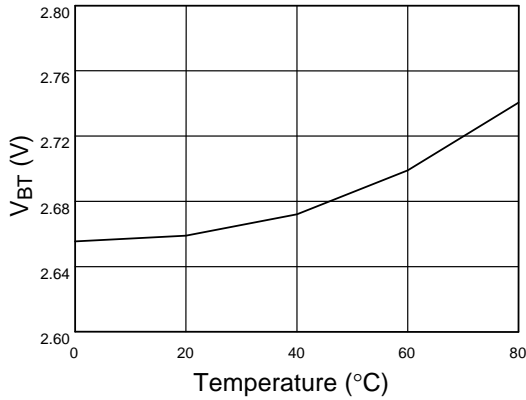
Fig. 8 VBT (High) Limit vs. Temperature (SEL3>3V)
