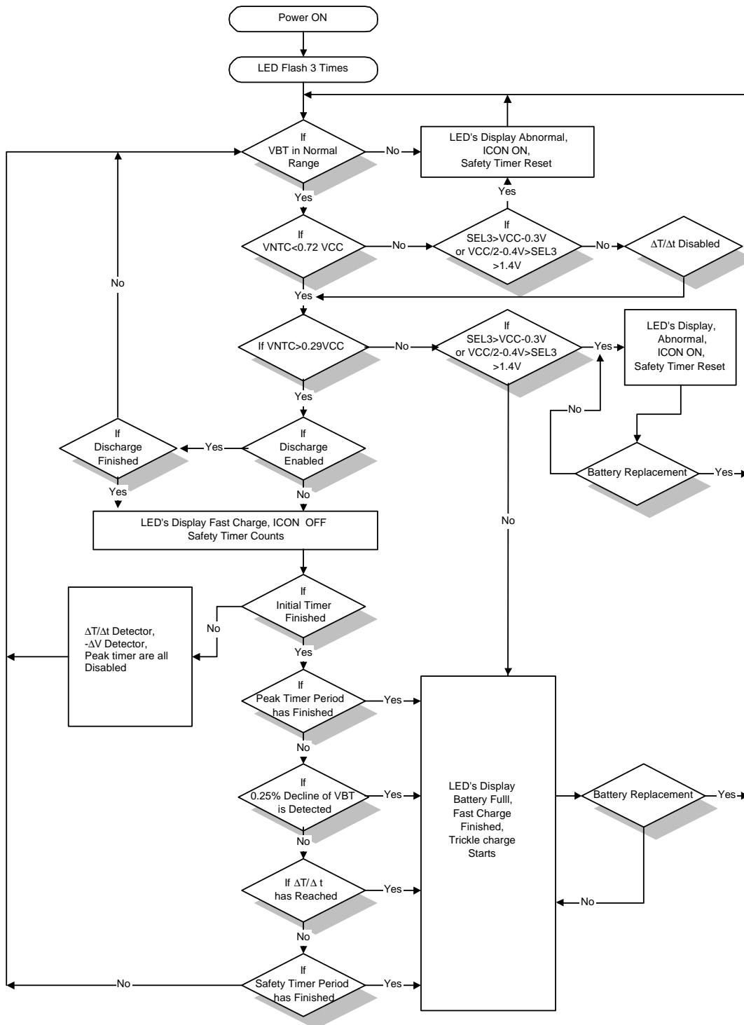
Fig. 16 Function Flow Chart of AIC1781A
