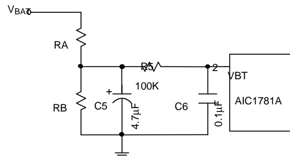
Fig. 17 Battery Voltage Divider
