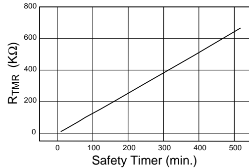
Fig. 19 Safety Timer vs. R_{TMR}
