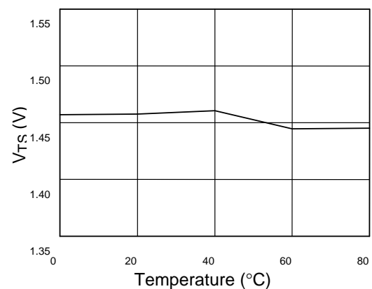
Fig. 13 V TS (High Temp) Limit vs. Temperature
