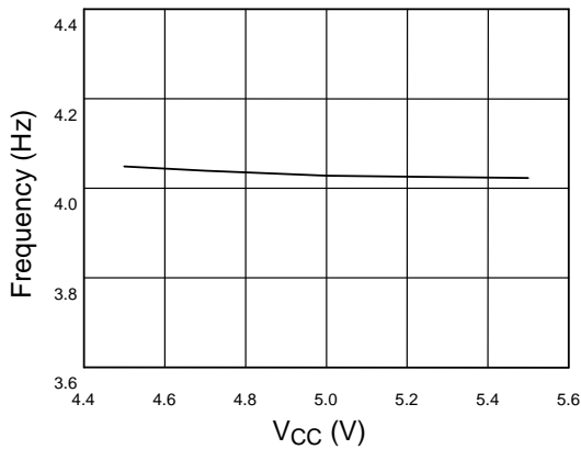
Fig. 4 LED Flashing Frequency vs. Supply Voltage
