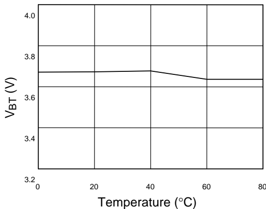
Fig. 12 VTS (Low Temp) Limit vs. Temperature
