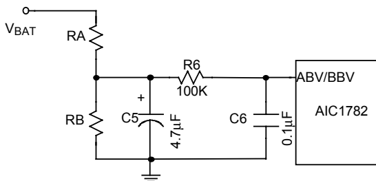
Fig. 2 Battery Voltage Divider
