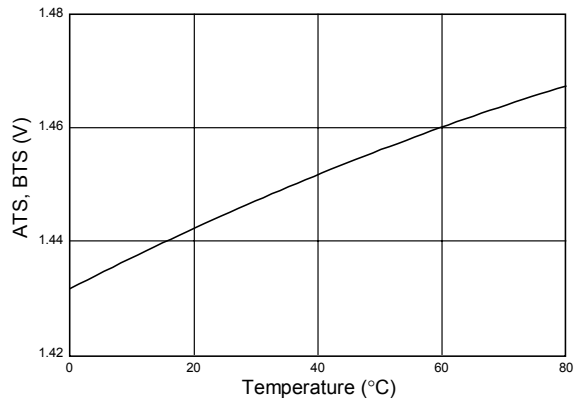
ATS and BTS (Low) Limit vs Temperature
