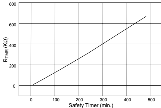
Fig. 4 Safety Timer vs R TMR
