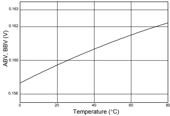
ABV and BBV (Low) Limit vs Temperature (Before Initial Timer)
