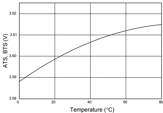
ATS and BTS (High) Limit vs Temperature
