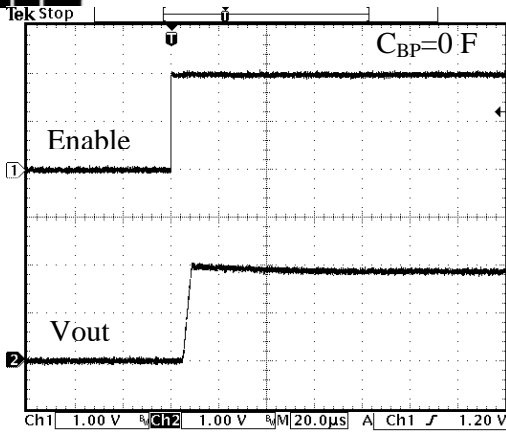
Fig. 19 Start-up Waveform
