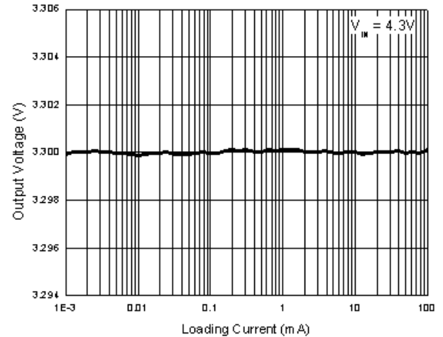
Fig. 12 Output Voltage VS Loading Current (3.3V)
