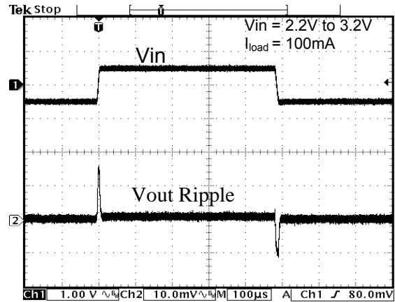
Fig. 14 Line Transient Response (1.2V)
