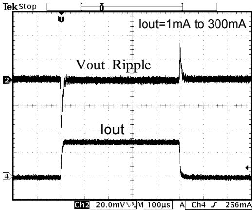
Fig. 13 Load Transient Response (1.2V)
