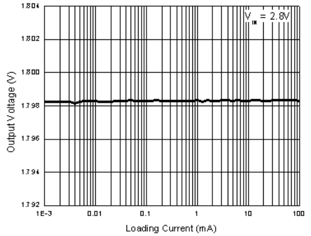
Fig. 10 Output Voltage VS Loading Current (1.8V)
