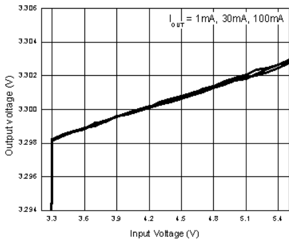
Fig. 11 Output Voltage VS Input Voltage (3.3V)
