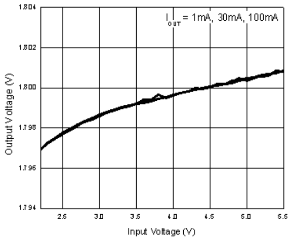
Fig. 9 Output Voltage VS Input Voltage (1.8V)
