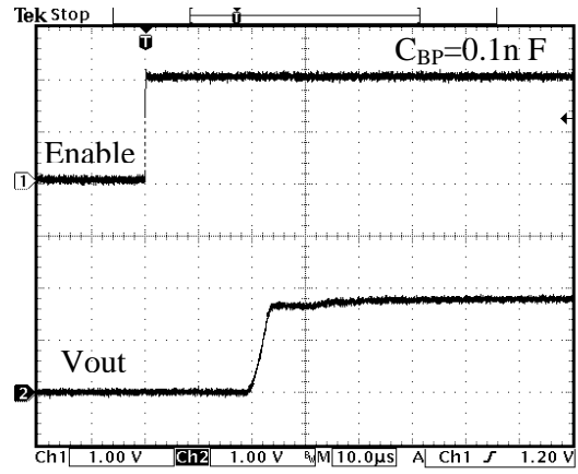
Fig. 20 Start-up Waveform
