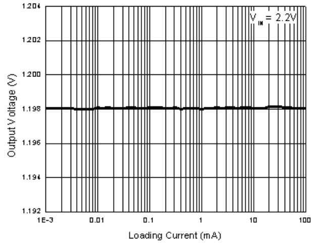
Fig. 8 Output Voltage VS Loading Current (1.2V)
