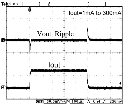
Fig. 15 Load Transient Response (1.8V)
