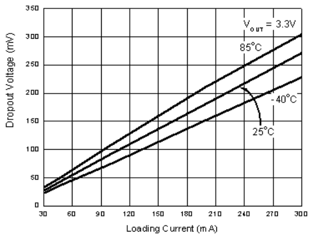
Fig.6 Dropout Voltage VS Loading Current (3.3V)
