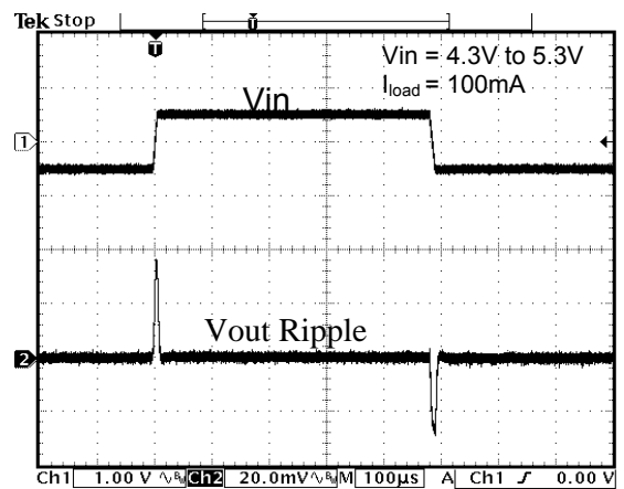
Fig. 18 Line Transient Response (3.3V)
