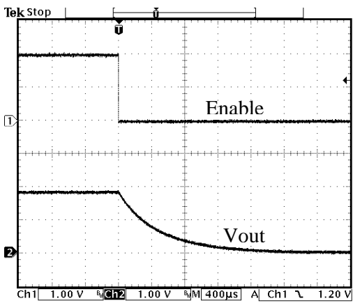
Fig. 21 Shutdown Waveform
