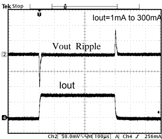
Fig. 17 Load Transient Response (3.3V)
