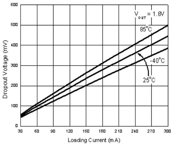
Fig.5 Dropout Voltage VS Loading Current (1.8V)
