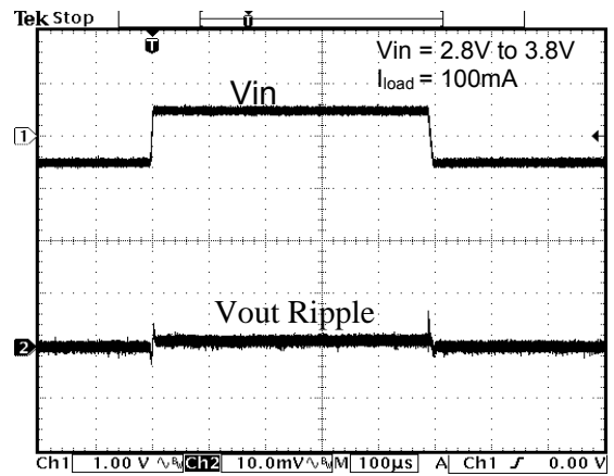
Fig. 16 Line Transient Response (1.8V)
