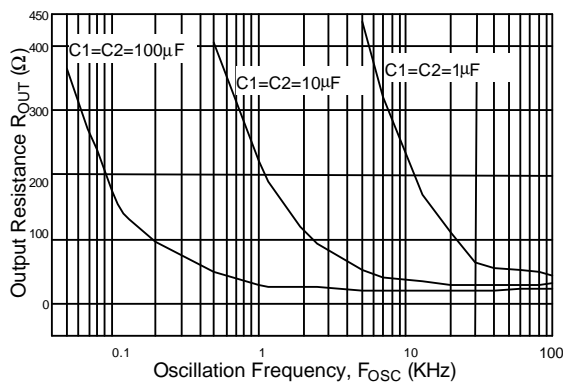
Fig. 7 Output Resistance vs. Oscillation Frequency
