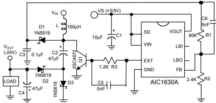
Fig. 4 -24V Output Inverting Converter for LCD
