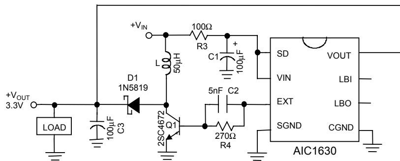
High Efficiency Step-Up DC/DC Converter
