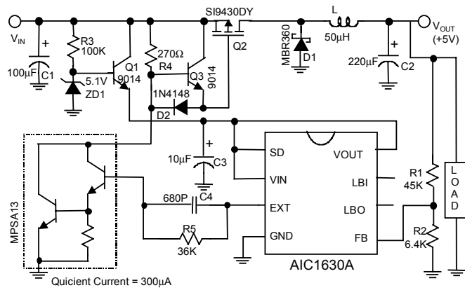
Fig. 8 5V Output Step-Down Converter -2
