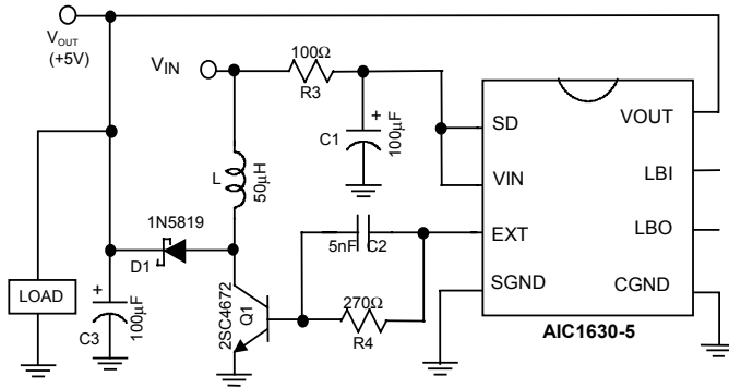
Fig. 1 5V Output Step-Up Converter
