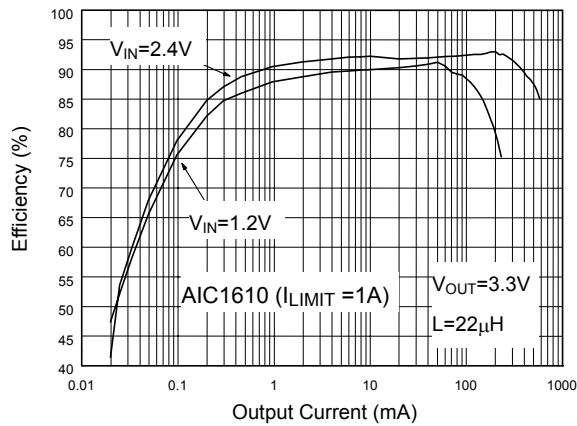
Fig. 43 Efficiency (ref. to Fig.38)
