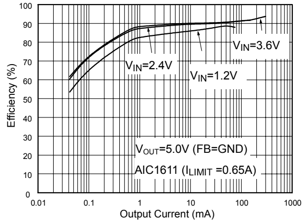
Fig. 8 Efficiency vs. Load Current (ref. to Fig.33)
