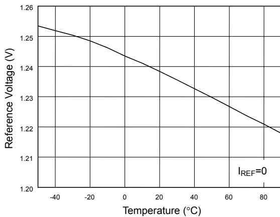
Fig. 17 Reference Voltage vs. Temperature
