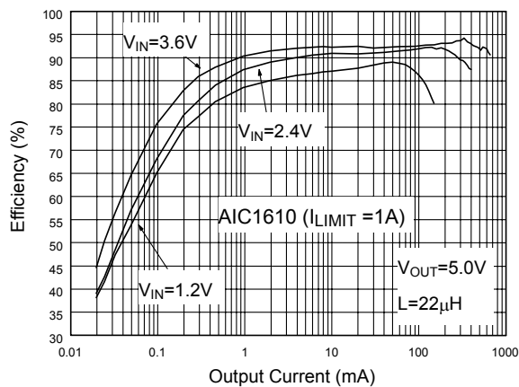
Fig. 39 Efficiency (ref. to Fig.38)
