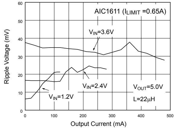
Fig. 42 Ripple Voltage (ref. to Fig.38)
