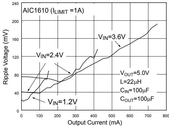
Fig. 7 Ripple Voltage (ref. to Fig.33)
