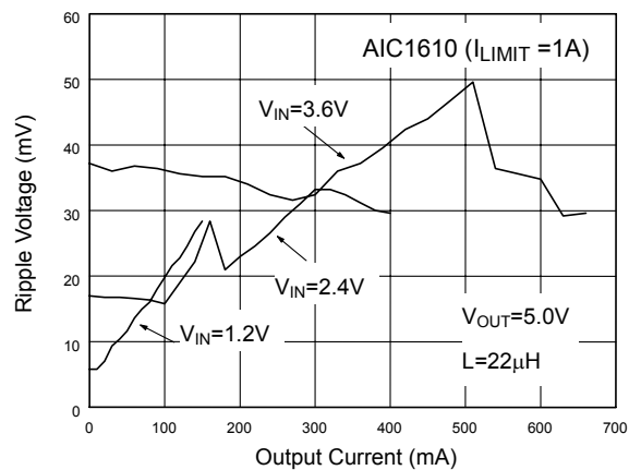
Fig. 40 Ripple Voltage (ref. to Fig.38)
