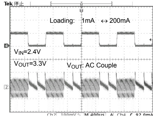
Fig. 26 Load Transient Response
