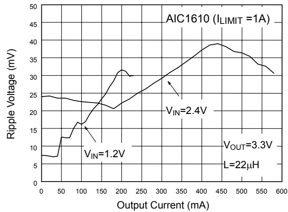
Fig. 44 Ripple Voltage (ref. to Fig.38)
