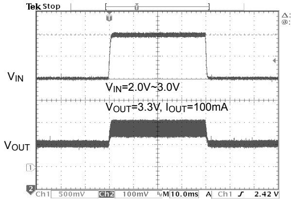
Fig. 27 Line Transient Response
