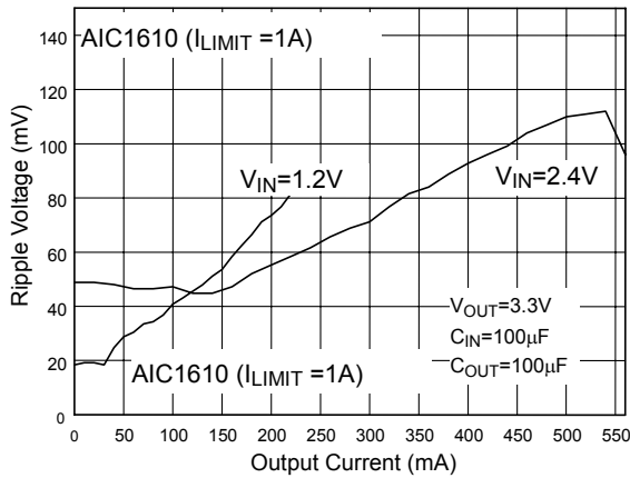
Fig. 13 Ripple Voltage (ref. to Fig.32)
