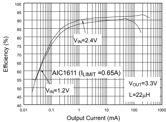
Fig. 45 Efficiency (ref. to Fig.38)
