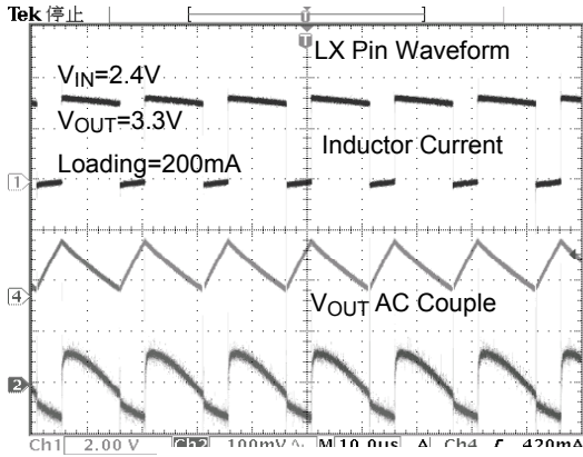
Fig. 25 Heavy Load Waveform
