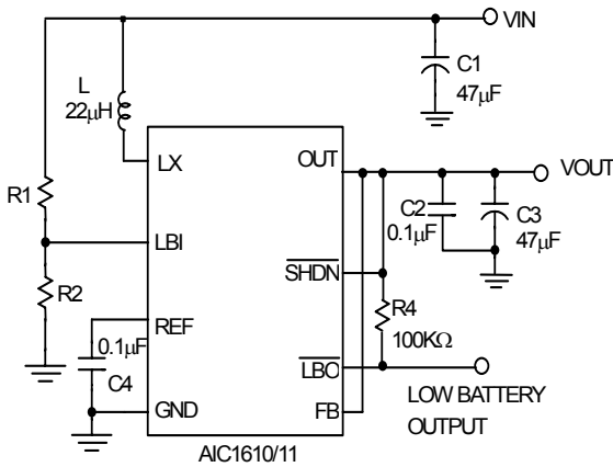
L: TDK SLF7045T-220MR90 C1, C3: NIPPON Tantalum Capacitor 6MCM476MB2TER Fig. 32. V_{OUT} = 3.3V Application Circuit.
