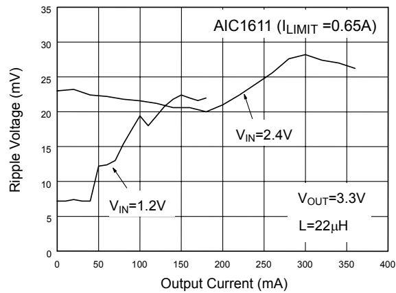
Fig. 46 Ripple Voltage (ref. to Fig.38)
