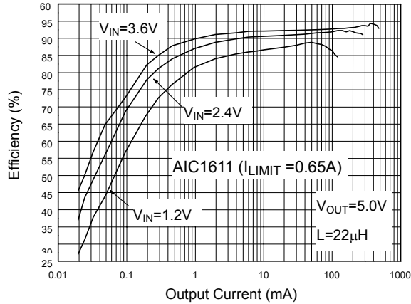
Fig. 41 Efficiency (ref. to Fig.38)
