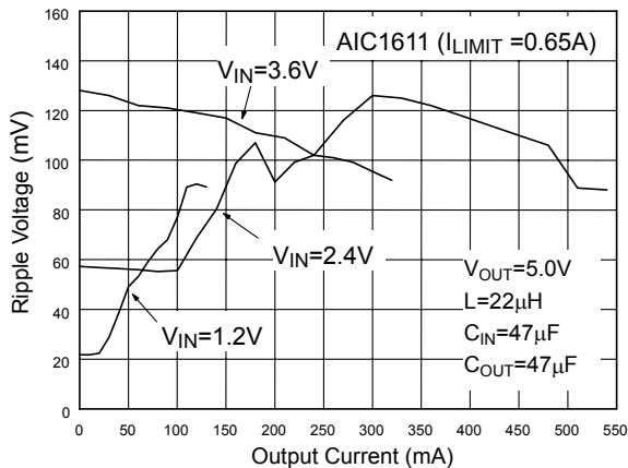
Fig. 9 Ripple Voltage (ref. to Fig.33)
