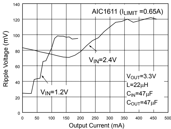
Fig. 15 Ripple Voltage (ref. to Fig.32)
