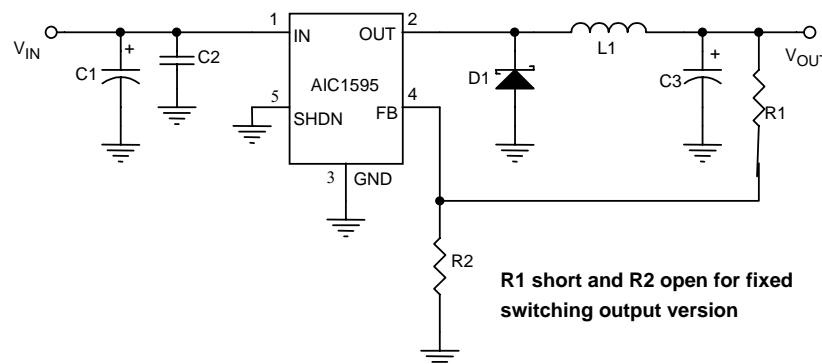
2A Precision PWM DC/DC Regulator
