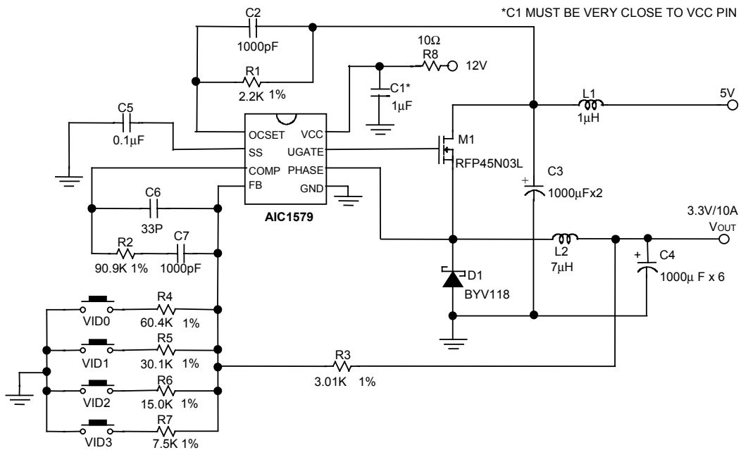
Switching Regulator for Pentium® V CORE Supply
