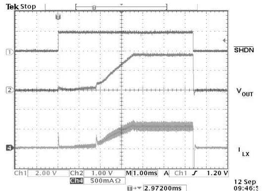
Fig. 16 Start-up from Shutdown, R_{LOAD}=3\Omega
