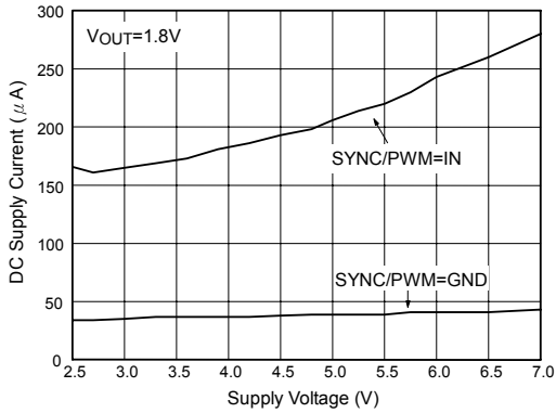
Fig. 13 DC Supply Current vs. Supply Voltage
