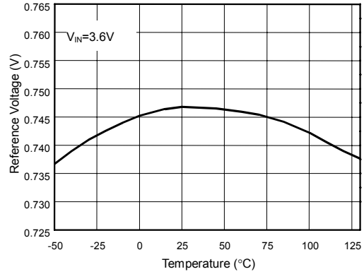
Fig. 8 Reference Voltage vs. Temperature
