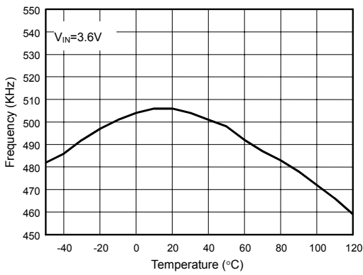
Fig. 9 Oscillator Frequency vs. Temperature
