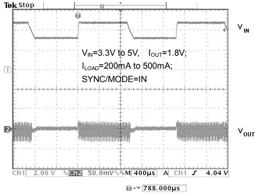
Fig. 19 Line Transient Response
