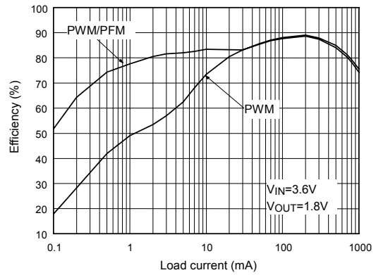
Fig. 14 Efficiency vs. Load current
