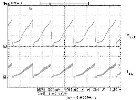
Fig. 20 Short Circuits Protection
