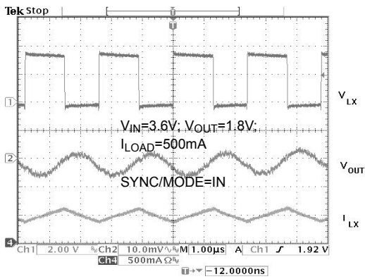
Fig. 21 Switching Waveform
