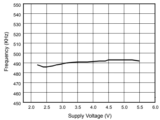
Fig. 10 Frequency vs. Input Voltage
