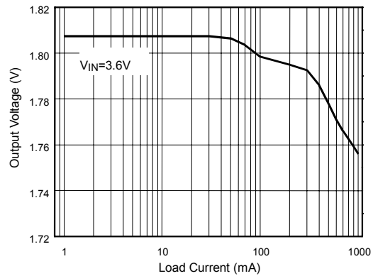
Fig. 12 Output Voltage vs. Load Current
