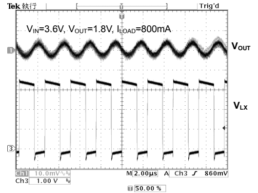
Fig. 22 Output Ripple voltage
