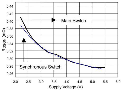
Fig. 11 RDSON vs. Supply Voltage
