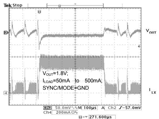
Fig. 18 Load Transient Response
