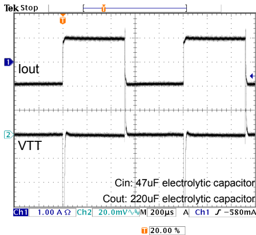
Fig.19 -0.9A to +0.9A load transient
