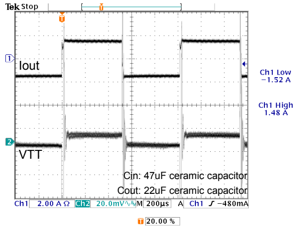
Fig.18 -1.5A to +1.5A load transient
