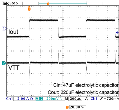
Fig.17 -1.5A to +1.5A load transient
