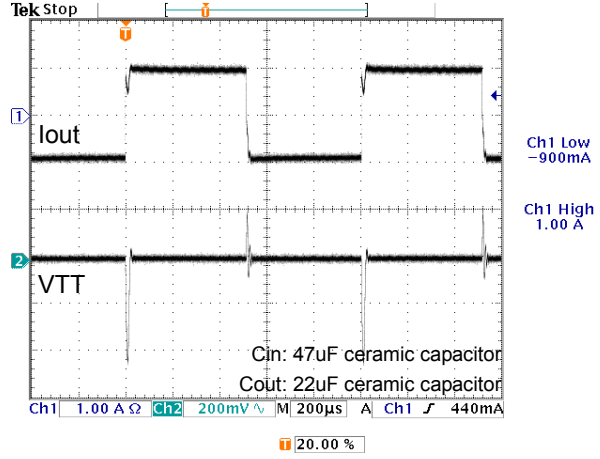
Fig.20 -0.9A to +0.9A load transient
