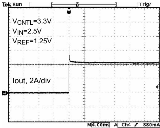
Fig. 7 Output Short-Circuit Protection (Sinking)
