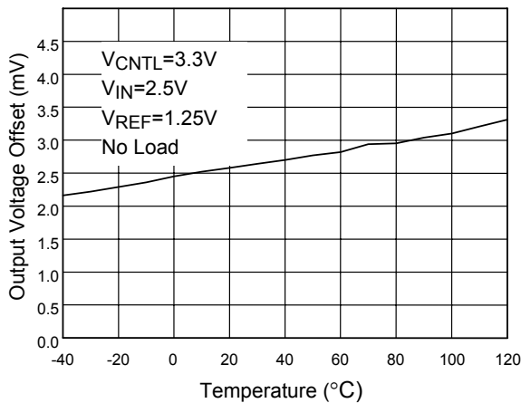
Fig. 3 Output Voltage Offset vs. Temp.
