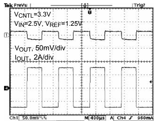
Fig. 6 Transient Response at 1.25V TT /3A
