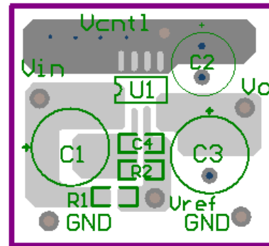
Fig. 11 Placement of SO-8
