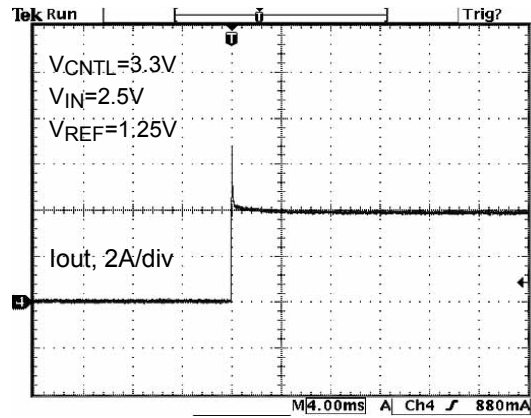
Fig. 8 Output Short-Circuit Protection (Sourcing)
