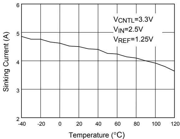
Fig. 5 Current-Limit (Sinking) vs. Temp.
