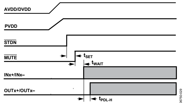
Figure 30. Recommended Power-Up Sequence
