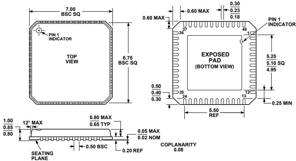
COMPLIANT TO JEDEC STANDARDS MO-220-VKKD-2 Figure 32. 48-Lead Lead Frame Chip Scale Package [LFCSP_VQ] 7 mm × 7 mm Body, Very Thin Quad (CP-48-1) Dimensions shown in millimeters
