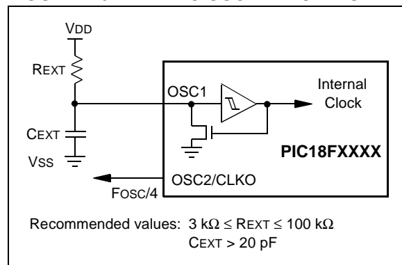
FIGURE 2-6: RC OSCILLATOR MODE
