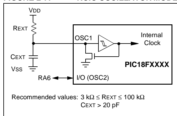
FIGURE 2-7: RCIO OSCILLATOR MODE
