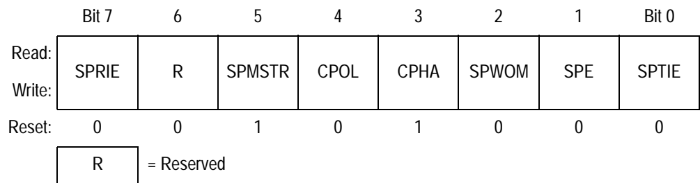
Figure 11. SPI Control Register (SPCR)
