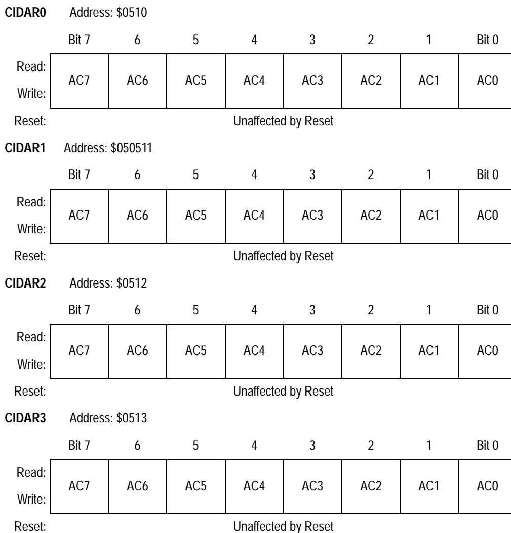
Figure 26. Identifier Acceptance Registers (CIDAR0–CIDAR3)
