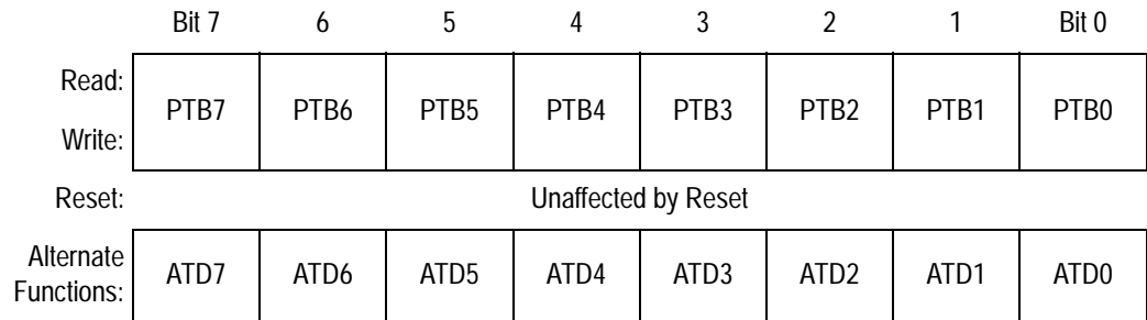
Figure 5. Port B Data Register (PTB)
