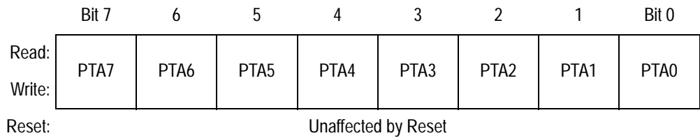
Figure 2. Port A Data Register (PTA)
