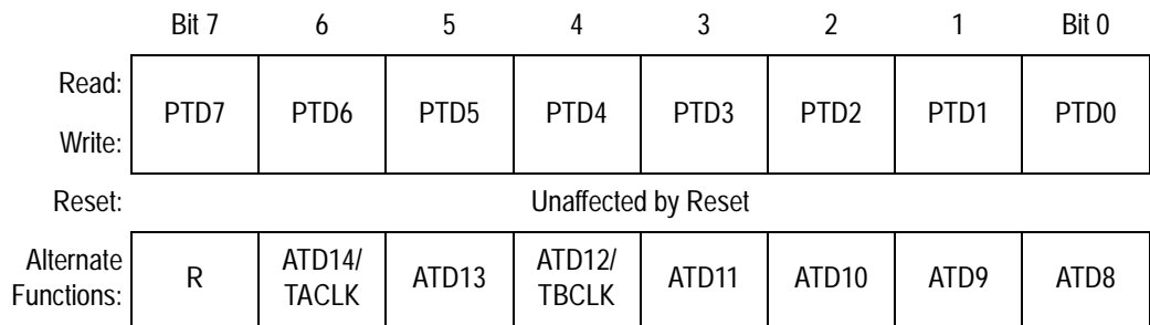
Figure 11. Port D Data Register (PTD)
