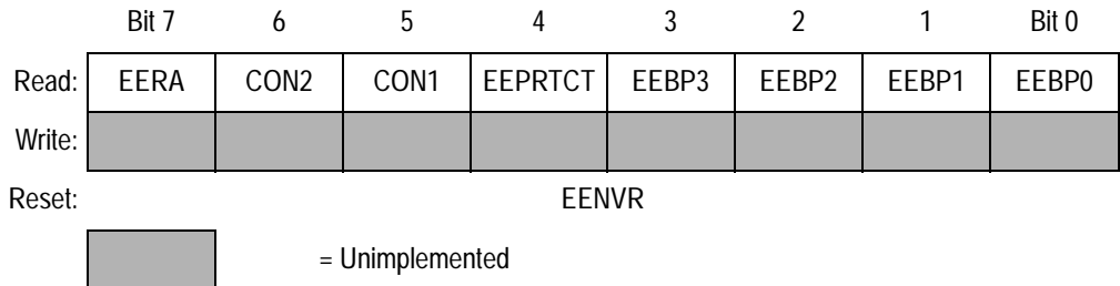
Figure 3. EEPROM-1 Array Control Register (EEACR1)
