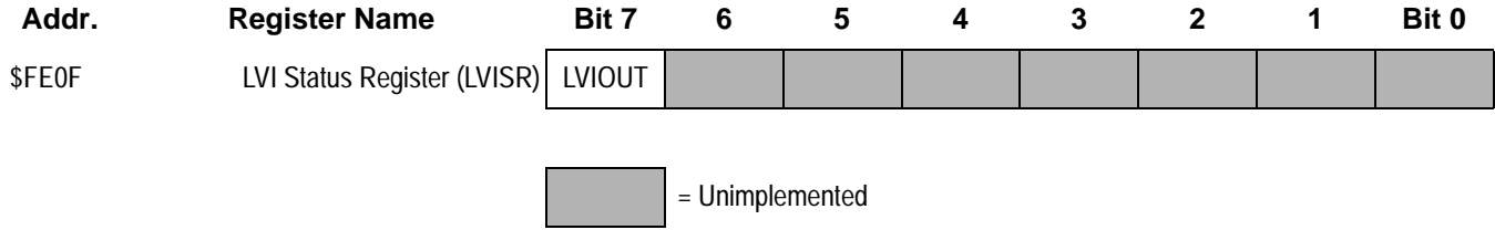
Figure 2. LVI I/O Register Summary
