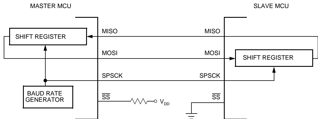
Figure 17-3. Full-duplex Master-Slave Connections
