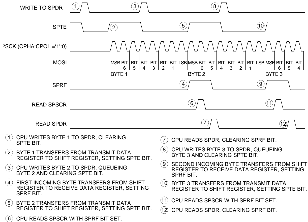
Figure 17-10. SPDR/SPTe CPU Interrupt Timing
