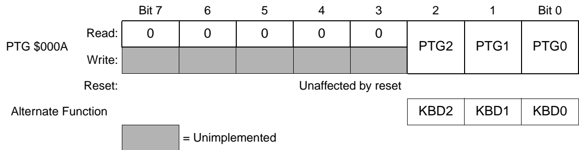
Figure 20-19. Port G Data Register (PTG)
