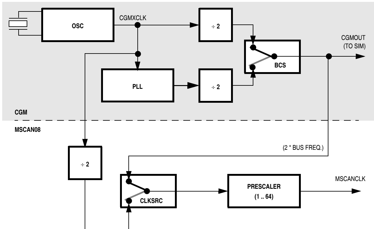
Figure 21-7. Clocking Scheme
