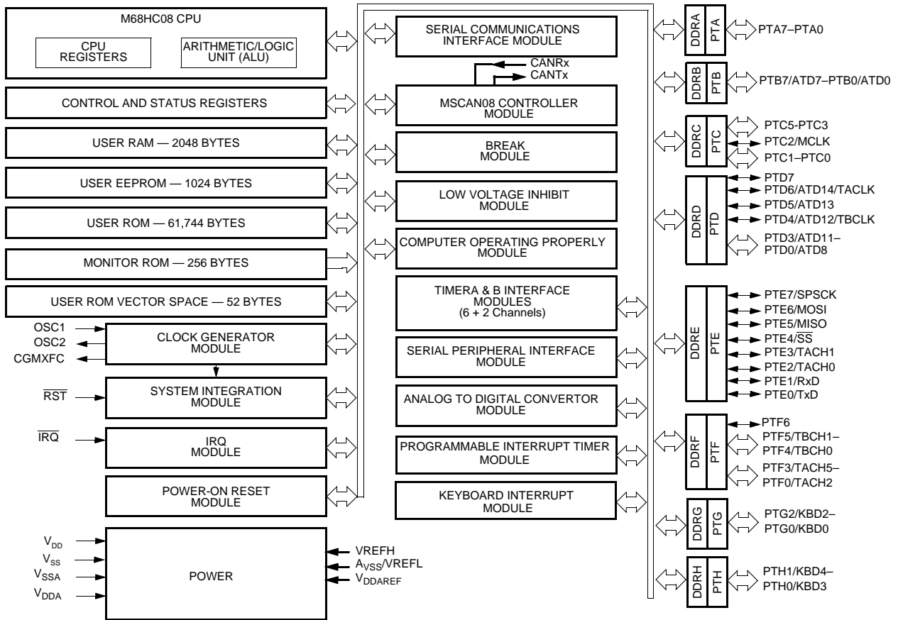
Figure 1-1. MC68HC08AZ60A MCU Block Diagram
