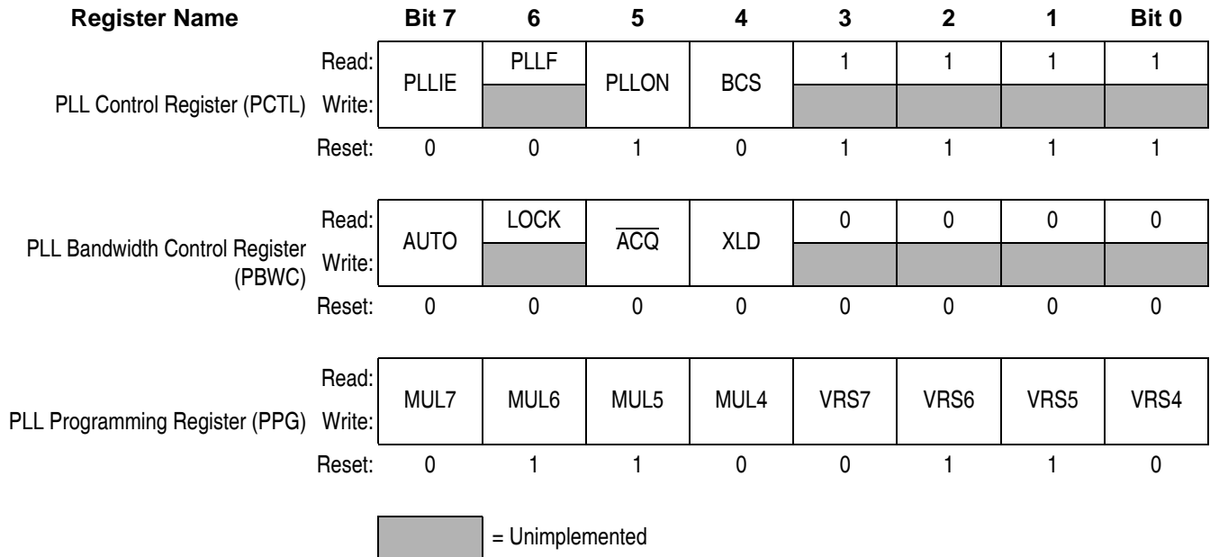
Figure 9-2. I/O Register Summary
