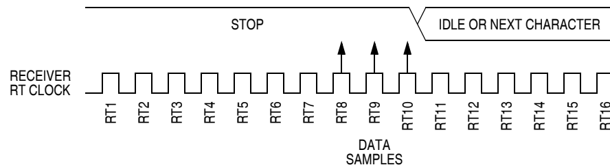
Figure 16-10. Fast Data
