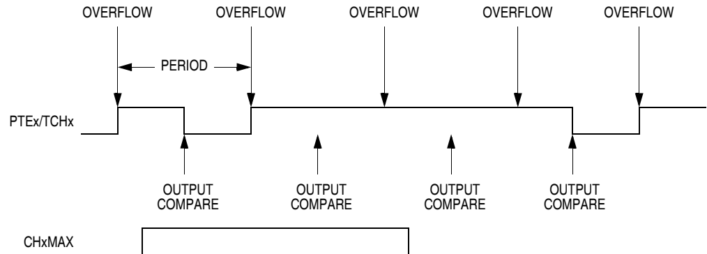
Figure 23-8. CHxMAX Latency
