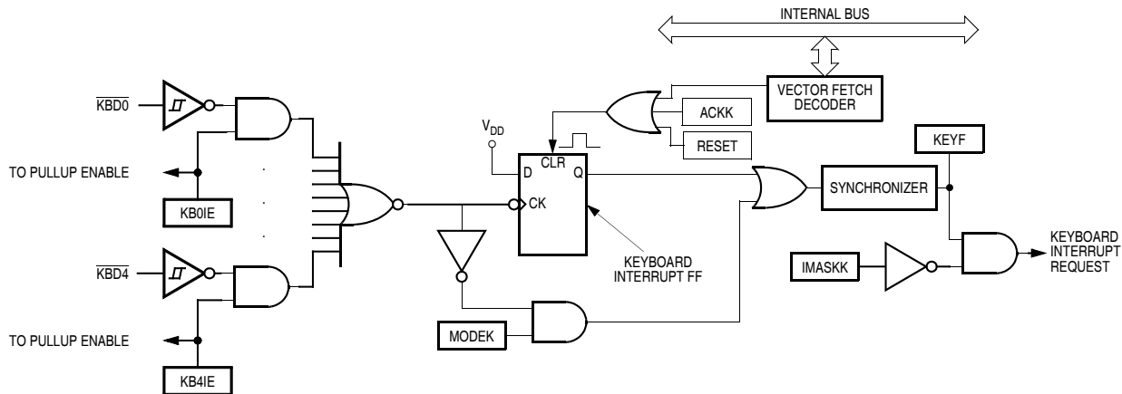
Figure 22-1. Keyboard Module Block Diagram
