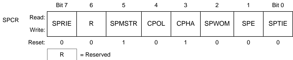
Figure 17-12. SPI Control Register (SPCR)
