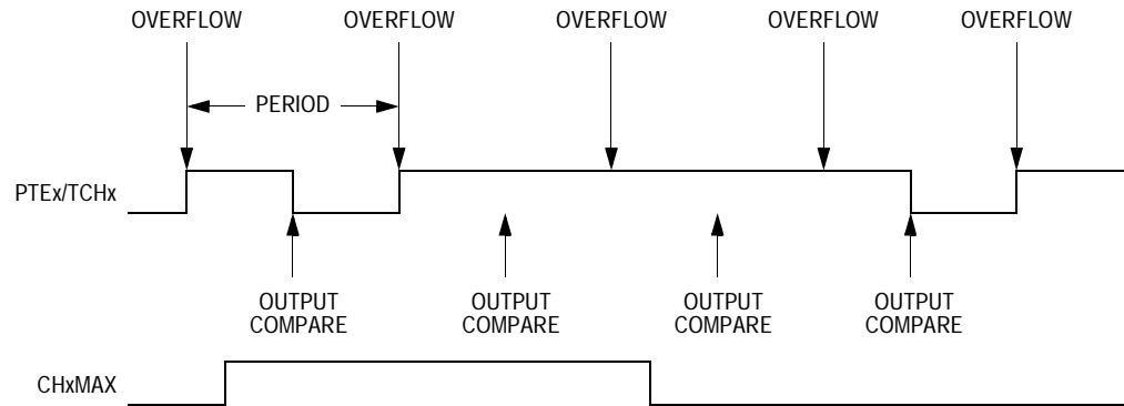
Figure 23-8. CHxMAX Latency
