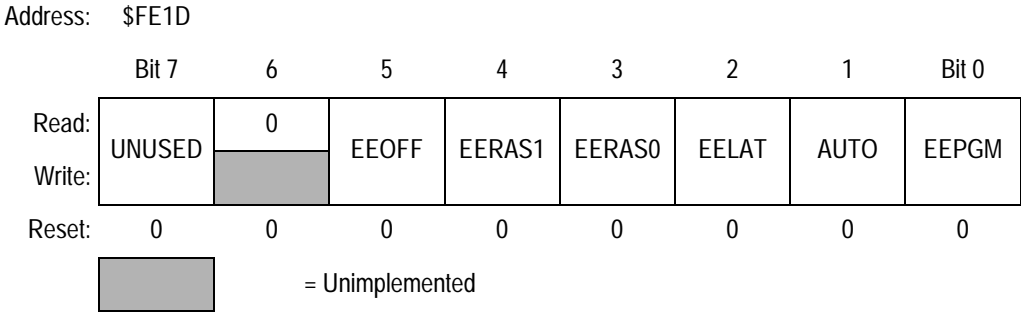
Figure 5-2. EEPROM-1 Control Register (EE1CR)
