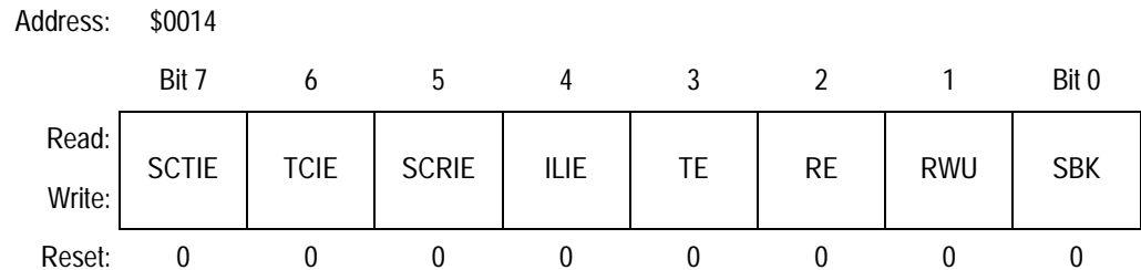
Figure 16-12. SCI Control Register 2 (SCC2)
