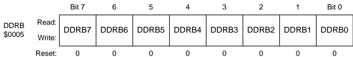
Figure 20-5. Data Direction Register B (DDRB)
