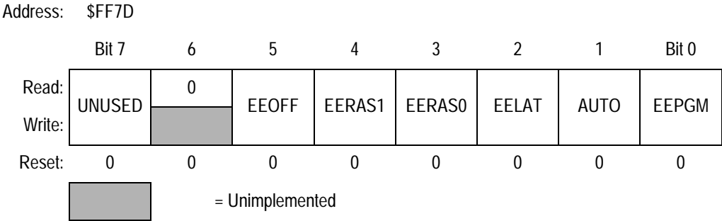
Figure 6-2. EEPROM-2 Control Register (EE2CR)
