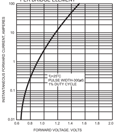
FIG.3- TYPICAL FORWARD CHARACTERISTICS PER BRIDGE ELEMENT
