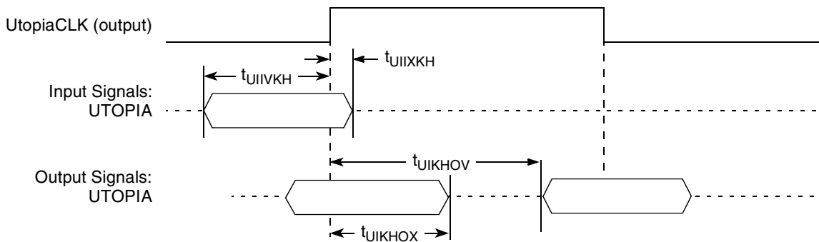
Figure 46. UTOPIA AC Timing (Internal Clock) Diagram
