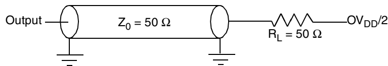
Figure 20. Local Bus C Test Load
