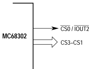
Figure 5-17. Chip-Select Pins
