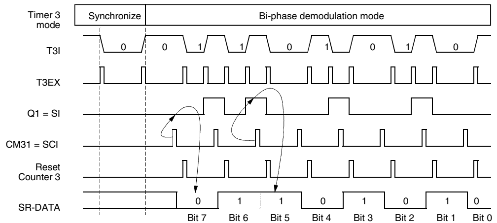
Figure 5-58. Bi-phase Demodulation
