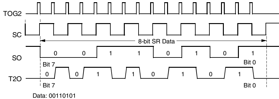
Figure 5-21. Manchester Modulation
