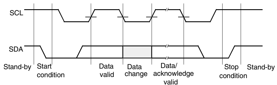
Figure 6-2. MCL Protocol
