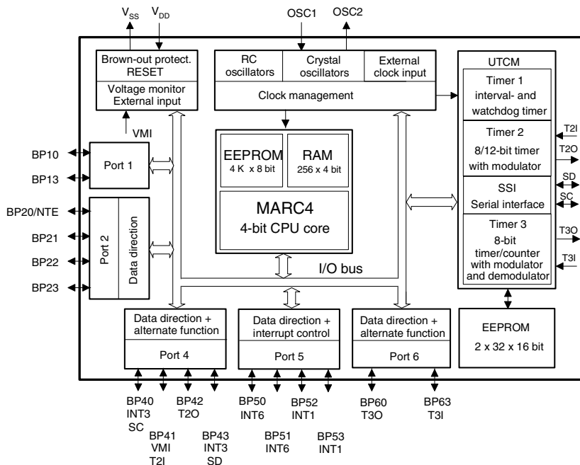
Figure 0-1. Block Diagram
