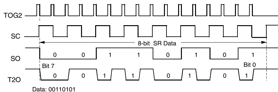
Figure 5-20. Bi-phase Modulation
