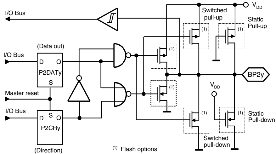
Figure 5-3. Bi-directional Port 2
