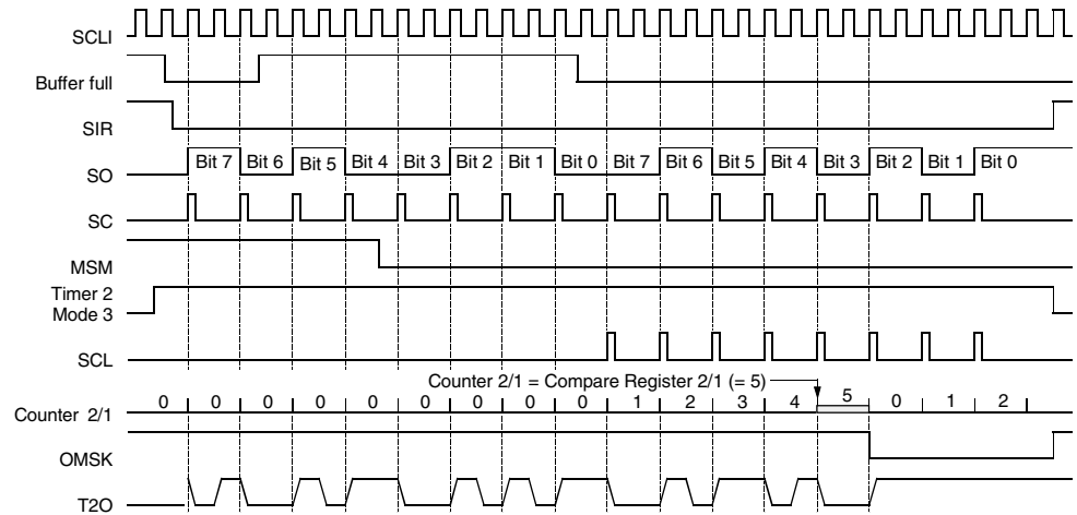
Figure 5-53. Bi-phase Modulation 2
