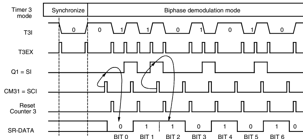
Figure 5-34. Bi-phase Demodulation
