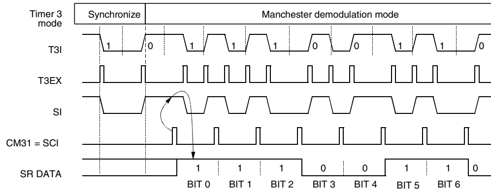
Figure 5-33. Manchester Demodulation
