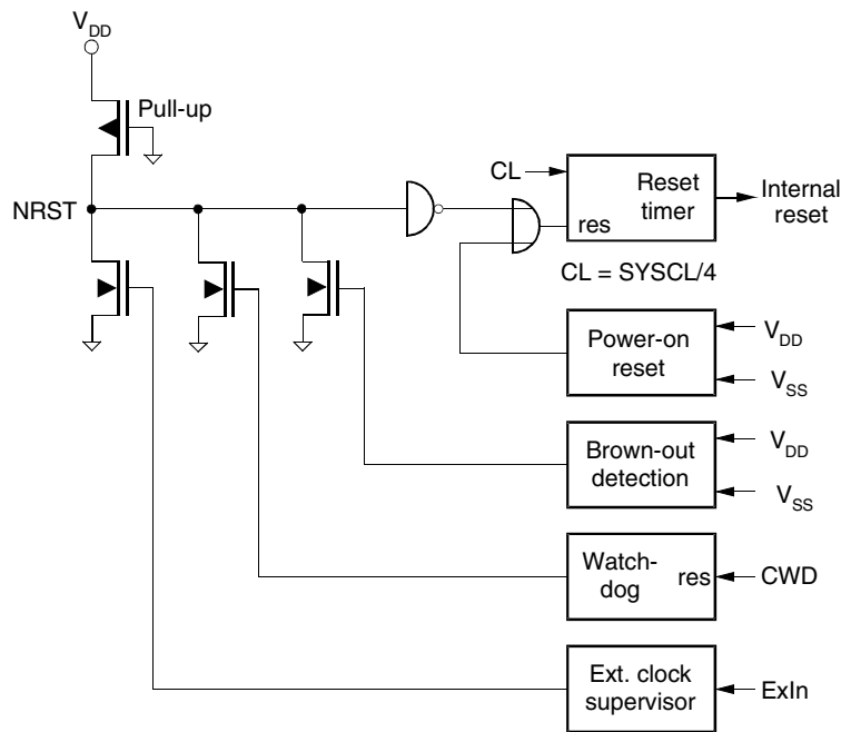
Figure 4-7. Reset Configuration
