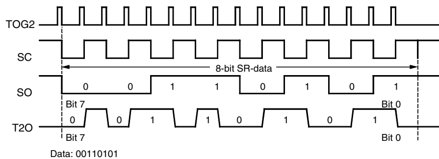
Figure 5-51. Manchester Modulation 1
