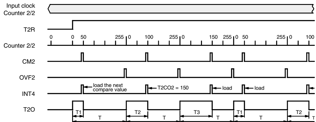
Figure 5-22. PWM Modulation
