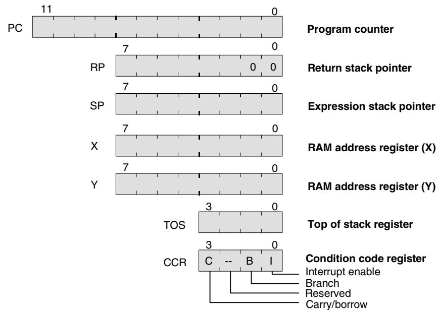
Figure 4-4. Programming Model
