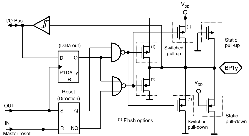
Figure 5-2. Bi-directional Port 1
