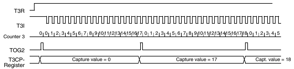
Figure 5-60. Frequency Measurement
