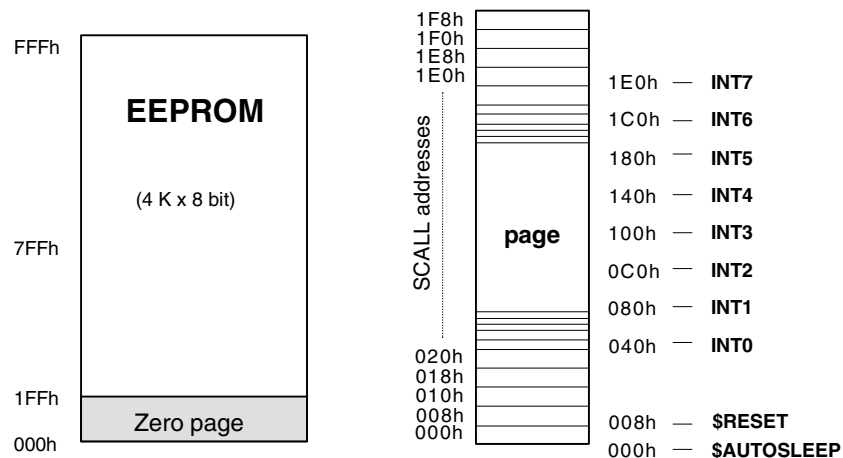
Figure 4-2. ROM Map
