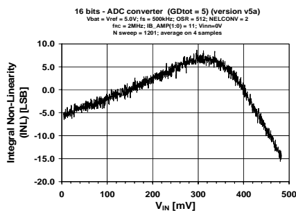
Figure 8.12: GAIN=5, 16 bit ADC setting
