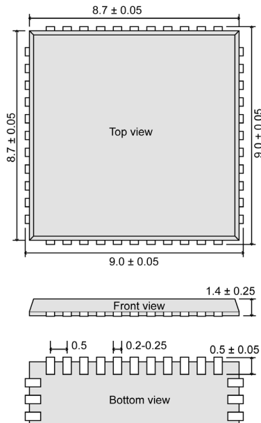
Figure 9.2: PLL-44L package,
