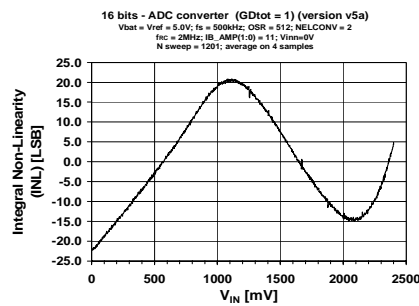
Figure 8.11: GAIN=1, 16 bit ADC setting
