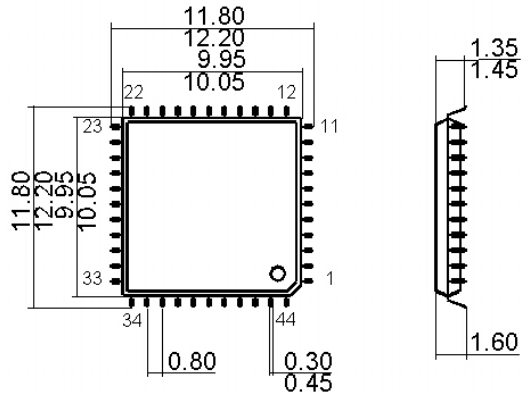
Figure 9.1: LQFP44 package, size in mm.
