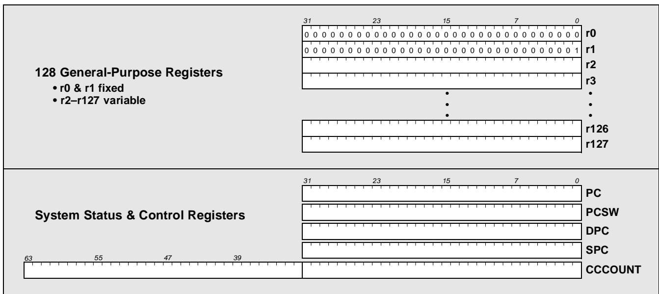
Figure 3-1. PNX1300 registers.
