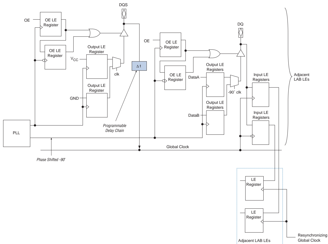
Figure 34. DDR SDRAM & FCRAM Interfacing
