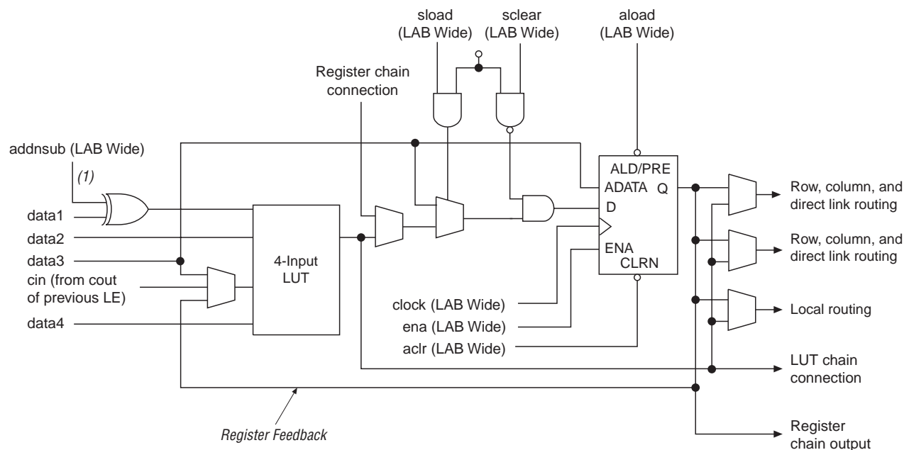
Figure 6. LE in Normal Mode
