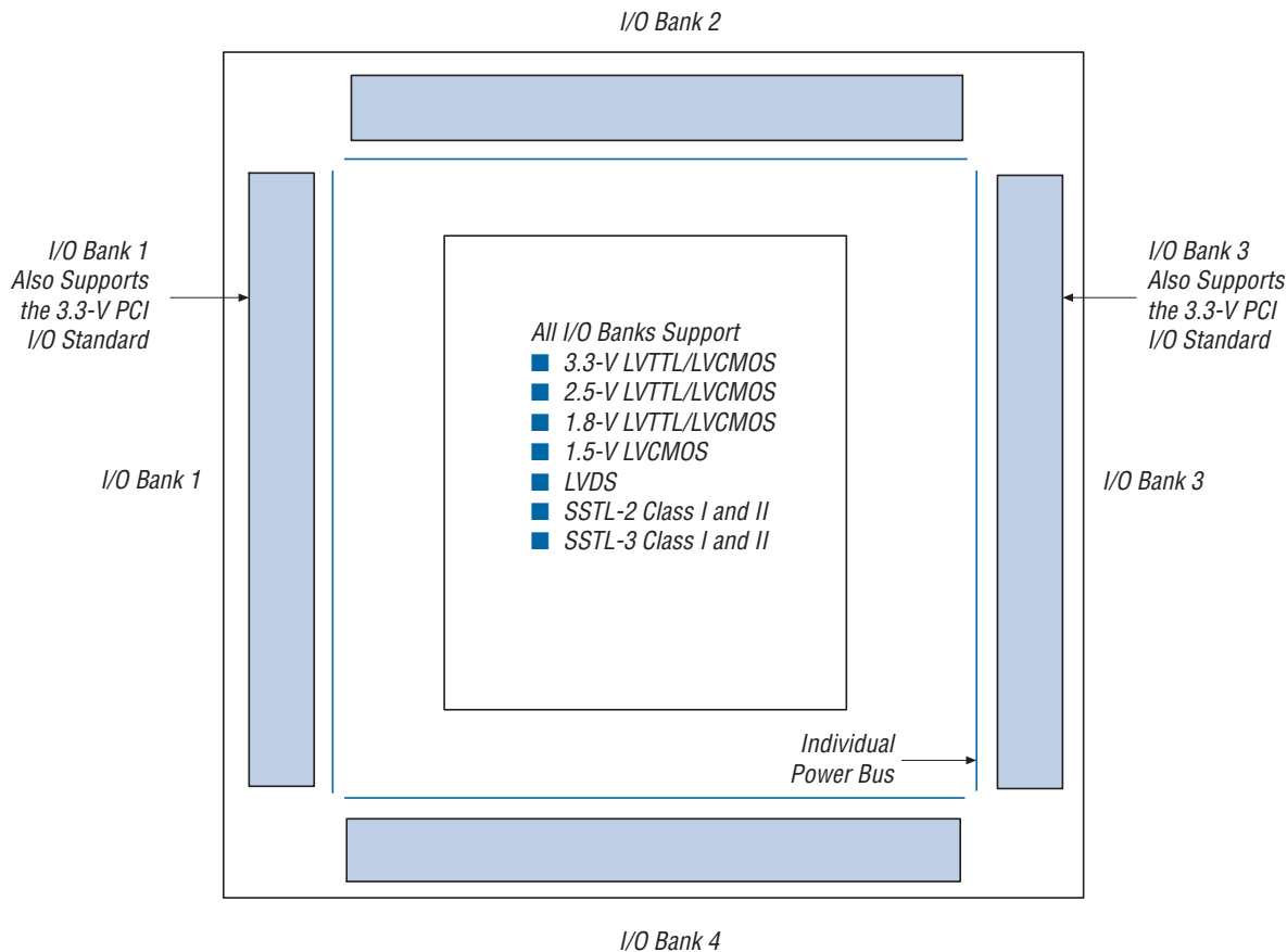
Figure 35. Cyclone I/O Banks Notes (1), (2)
