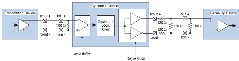
Figure 11-3. Typical LVDS Application
