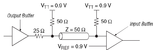
Figure 10-6. 1.8-V SSTL Class II Termination
