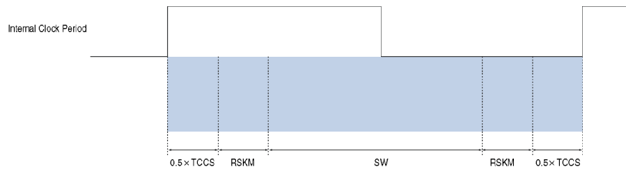
Figure 11–16. Cyclone II High-Speed I/O Timing Budget Note (1)
