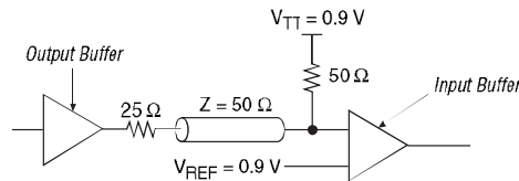
Figure 10-5. 1.8-V SSTL Class I Termination
