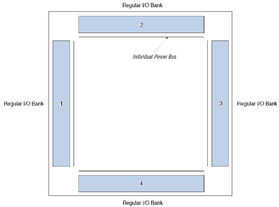
Figure 10-19. EP2C5 & EP2C8 Device I/O Banks Notes (1), (2)
