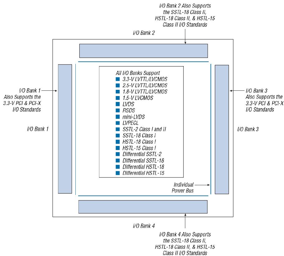
Figure 11–1. I/O Banks in EP2C5 & EP2C8 Devices
