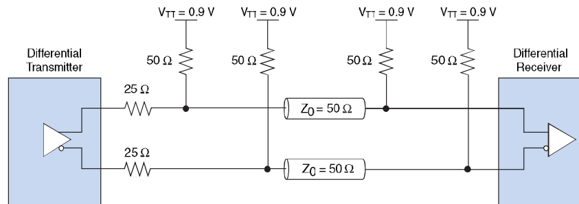
Figure 10-10. Differential SSTL-18 Class II Termination
