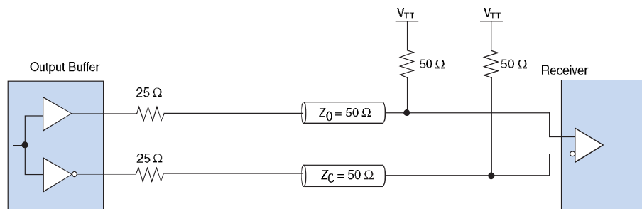
Figure 11–11. Differential SSTL Class I Interface
