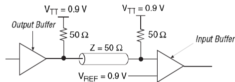
Figure 10-8. 1.8-V HSTL Class II Termination
