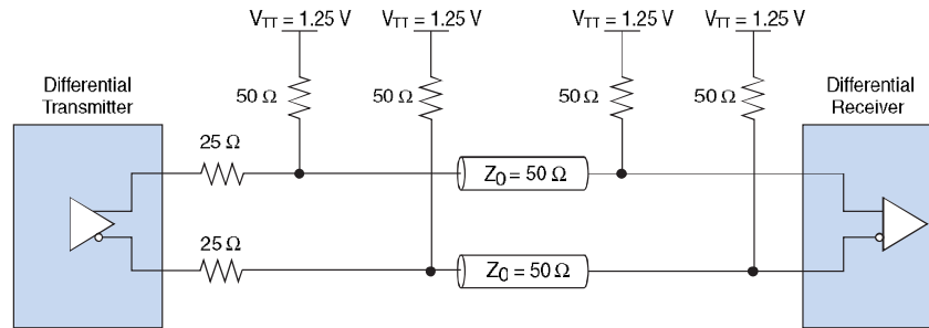
Figure 10-4. SSTL-2 Class II Differential Termination
