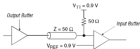
Figure 10-7. 1.8-V HSTL Class I Termination
