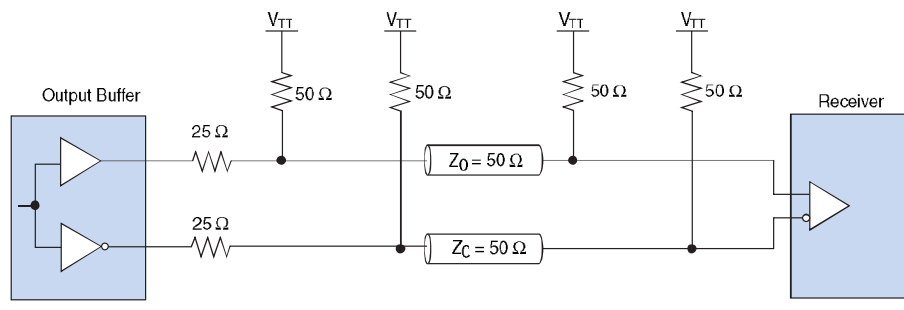
Figure 11–12. Differential SSTL Class II Interface
