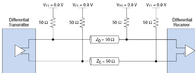
Figure 10–12. 1.8-V Differential HSTL Class II Termination
