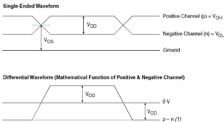
Figure 11-6. Transmitter Output Signal Level Waveforms for RSDS
