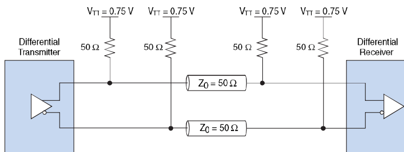
Figure 10–16. 1.5-V Differential HSTL Class II Termination
