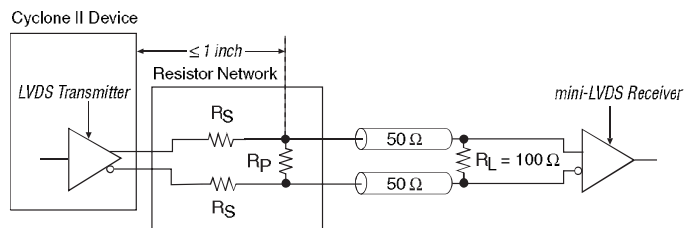
Figure 11-9. mini-LVDS Resistor Network
