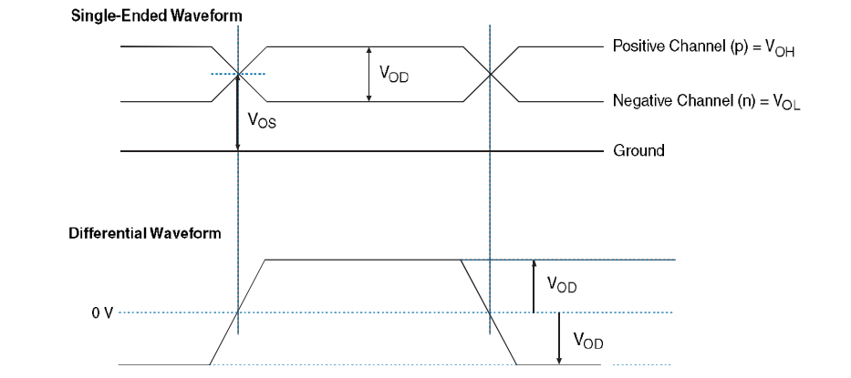
Figure 11-8. Transmitter Output Signal Level Waveforms for mini-LVDS
