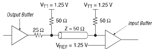
Figure 10–2. SSTL-2 Class II Termination
