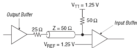
Figure 10-1. SSTL-2 Class I Termination
