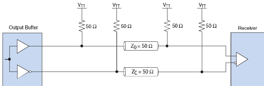
Figure 11-14. Differential HSTL Class II Interface
