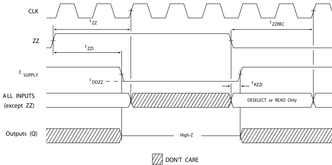
Figure 5. ZZ Mode Timing
