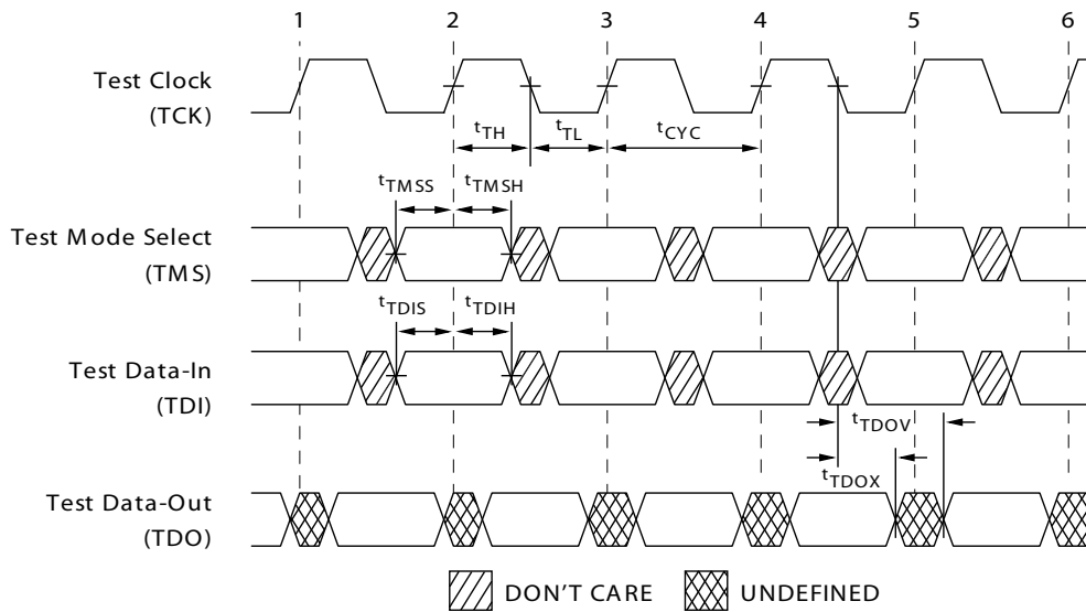
Figure 2. TAP Timing
