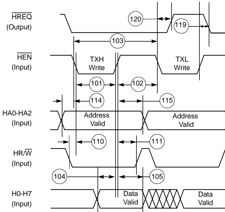
Figure 27 Host Write Cycle (Non-DMA Mode)
