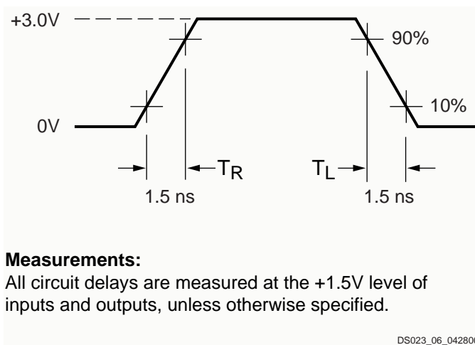
Figure 5: Voltage Waveform
