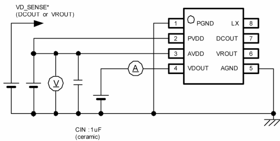
Circuit 9 VD Output Current
