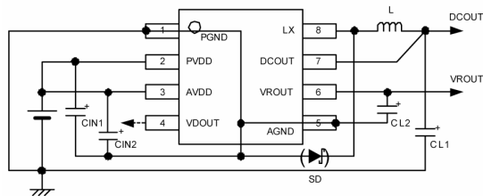
SOP-8 (TOP VIEW)
