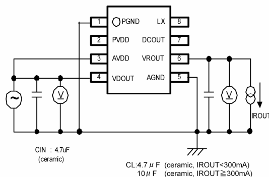
Circuit 12 Ripple Rejection Rate
