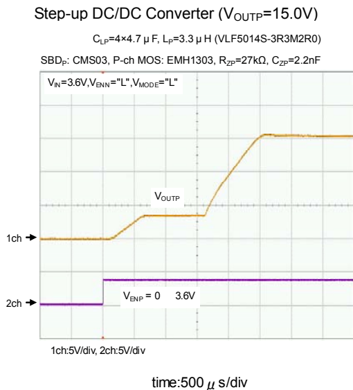
(17) Output Voltage Rise Wave Form
