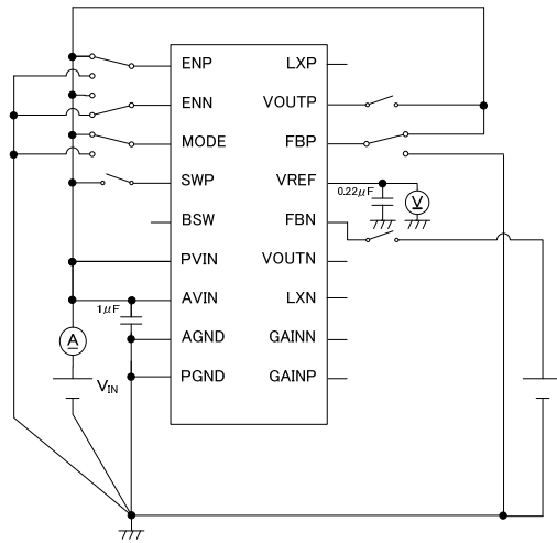
3) Circuit
