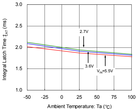
(21) Latch Time vs. Ambient Temperature
