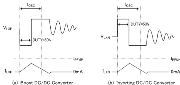
Fig. Maximum PFM Current Duty
