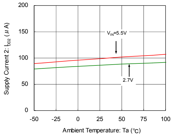
Supply Current 2
