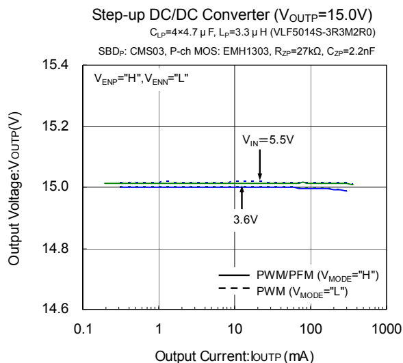
(2) Output Voltage vs. Output Current (Continued)
