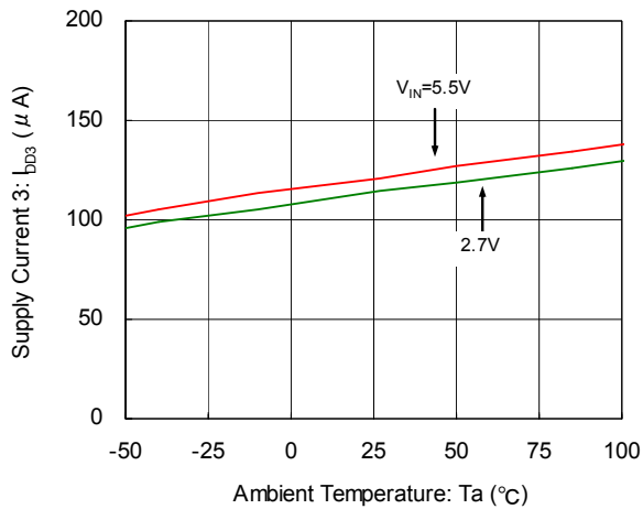
Supply Current 3
