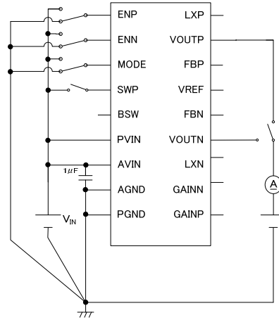
2) Circuit
