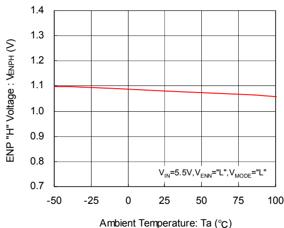
(9) ENP "H" Voltage vs. Ambient Temperature
