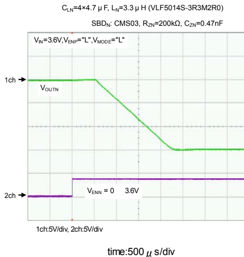
Inverting DC/DC Converter ( V_{OUTN}=-15.0V )
