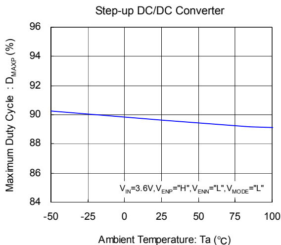
(19) Maximum Duty Cycle vs. Ambient Temperature
