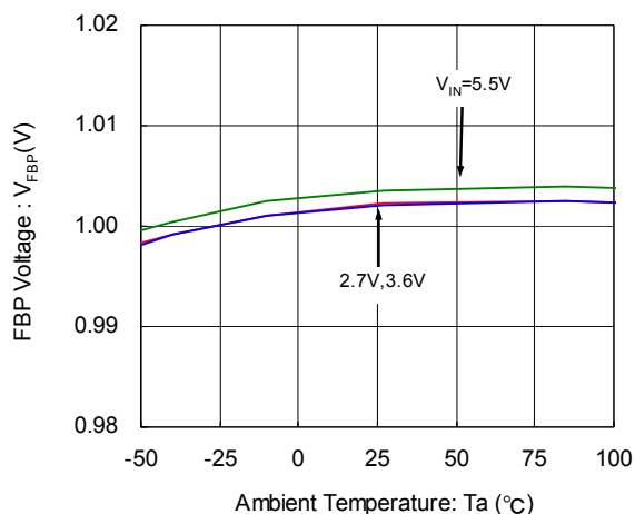
(6) FBP Voltage vs. Ambient Temperature
