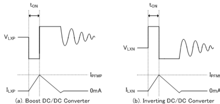
Fig. PFM Current
