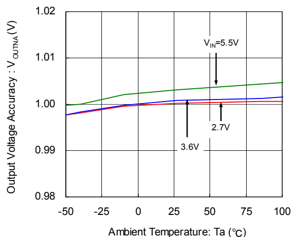
(7) Output Voltage Accuracy vs. Ambient Temperature
