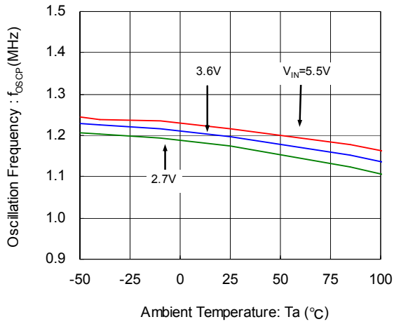
(4) Oscillation Frequency vs. Ambient Temperature
