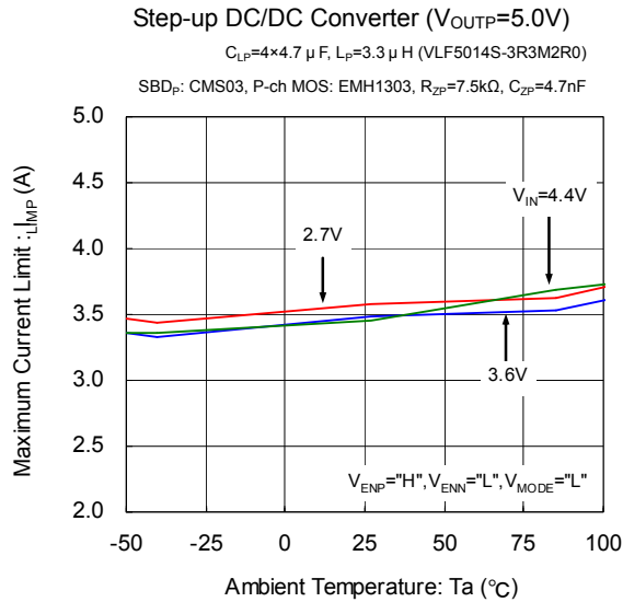
(20) Maximum Current Limit vs. Ambient Temperature
