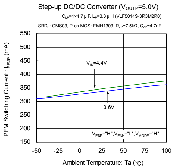
(23) PFM Switching Current vs. Ambient Temperature
