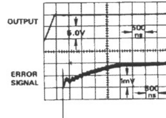
Figure 3. Settling Time of AD509
