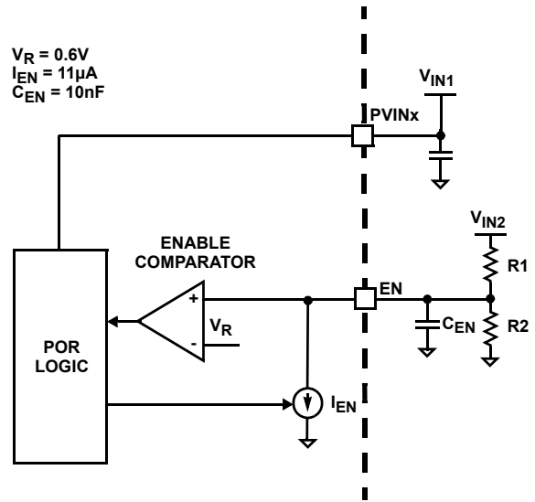
FIGURE 7. ENABLE CIRCUIT
