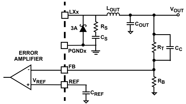
FIGURE 11. SCHOTTKY DIODE AND R-C SNUBBER
