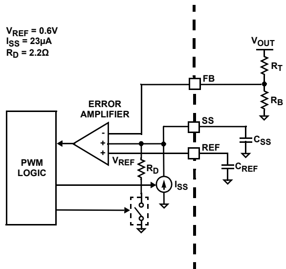
FIGURE 8. SOFT-START CIRCUIT
