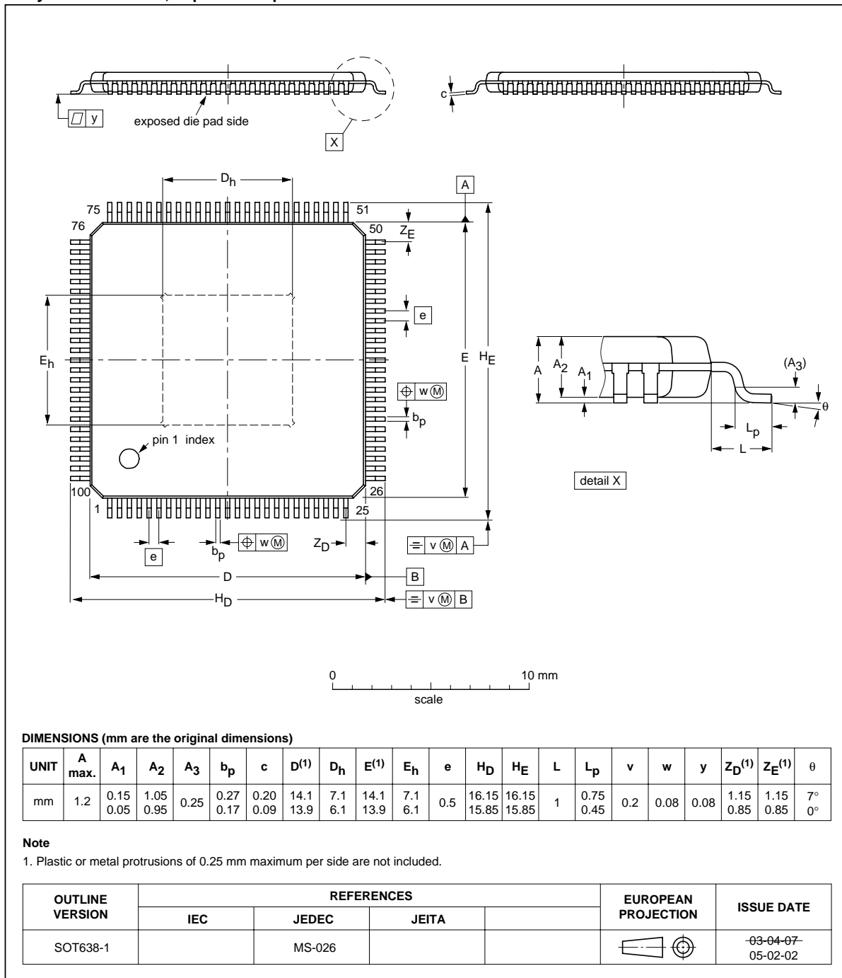
Fig 22. Package outline SOT638 (HTQFP100)
