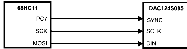
FIGURE 12. 68HC11 Interface
