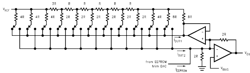
FIGURE 5. Equivalent Circuit of R-2R Ladder and Output Amplifier
